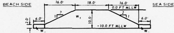
SECTION W-W'
