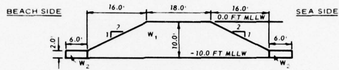
SECTION W-W'
