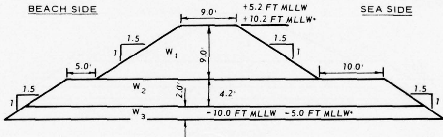
SECTION E-E'
