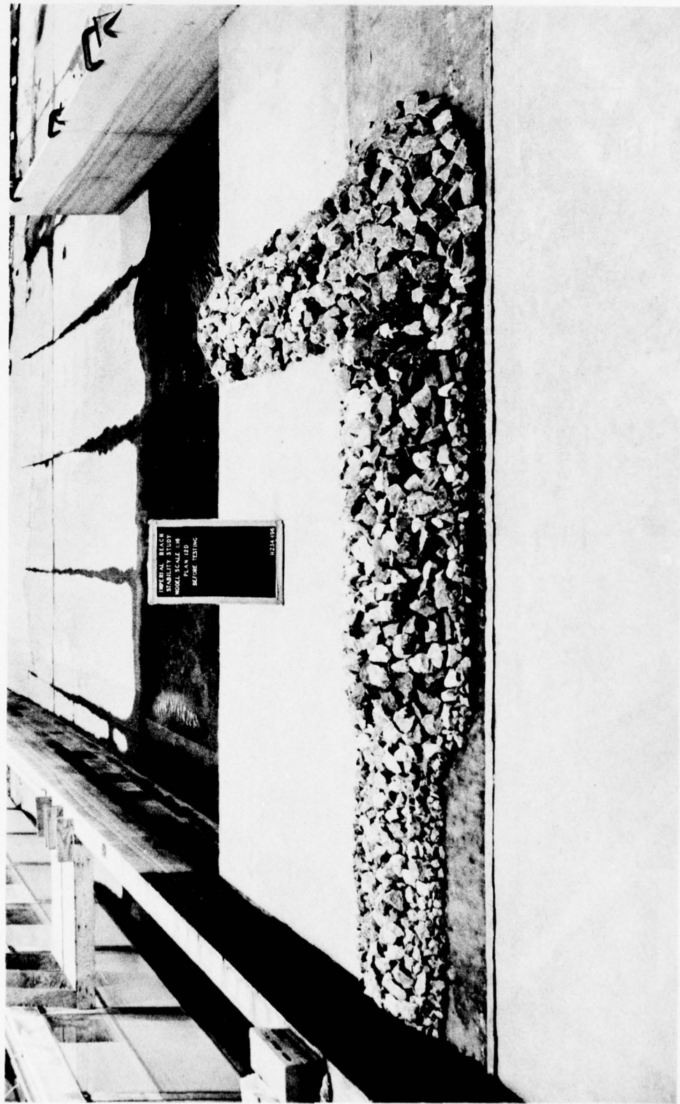
Photo 79. Sea-side view of Plan I2D before wave attack
