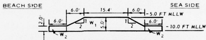
SECTION X-X'
