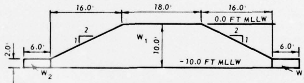
SECTION W-W'
