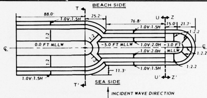
PLAN VIEW
