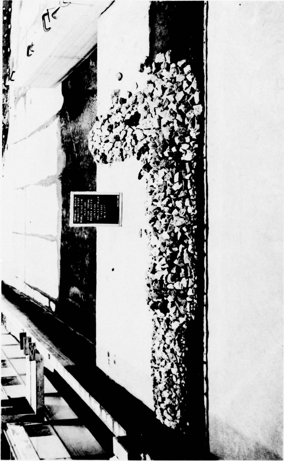
Photo 80. Sea-side view of Plan 12D in the deeper water location after 2.0 hr of 14.0-sec, 12.1-ft waves at an swl of +5.4 ft mllw
