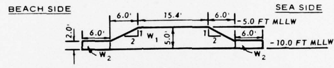
SECTION X-X' MATERIAL CHARACTERISTICS
