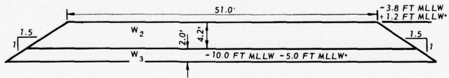
SECTION F-F'
