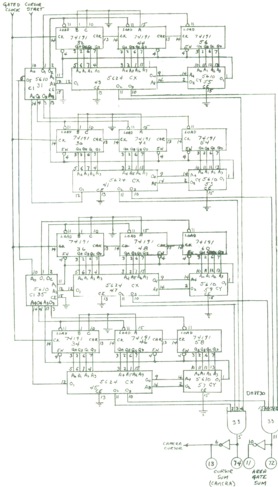
Fig. A1-13. Cursor Generator Function Logic (Sheet 3 of 3).
