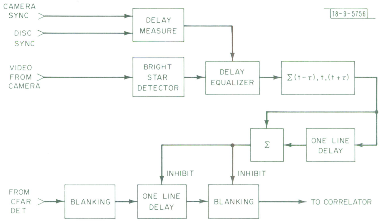
Fig. 17. Bright star blanking circuit.
