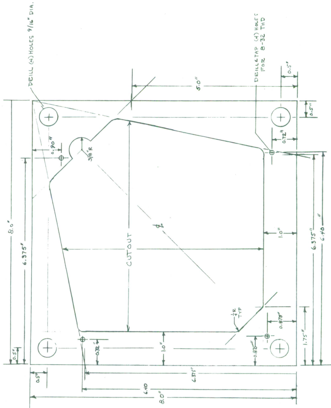
Fig. A11-46. Head Alignment Jig Make (1) From 3/8" Alum.
