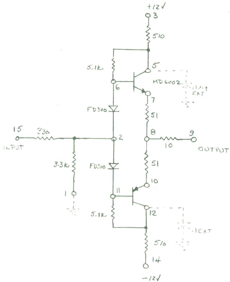
Fig. AII-2. 75 Ω Video line driver on component carrier.
