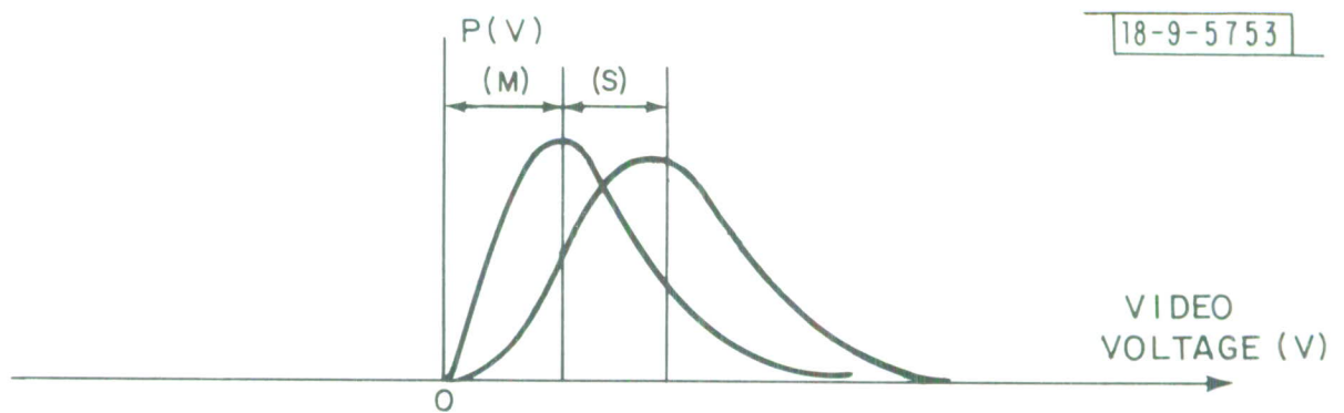
Fig. 14. Probability density of video noise background before subtraction.
