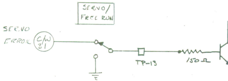
ORIGINAL CIRCUIT
