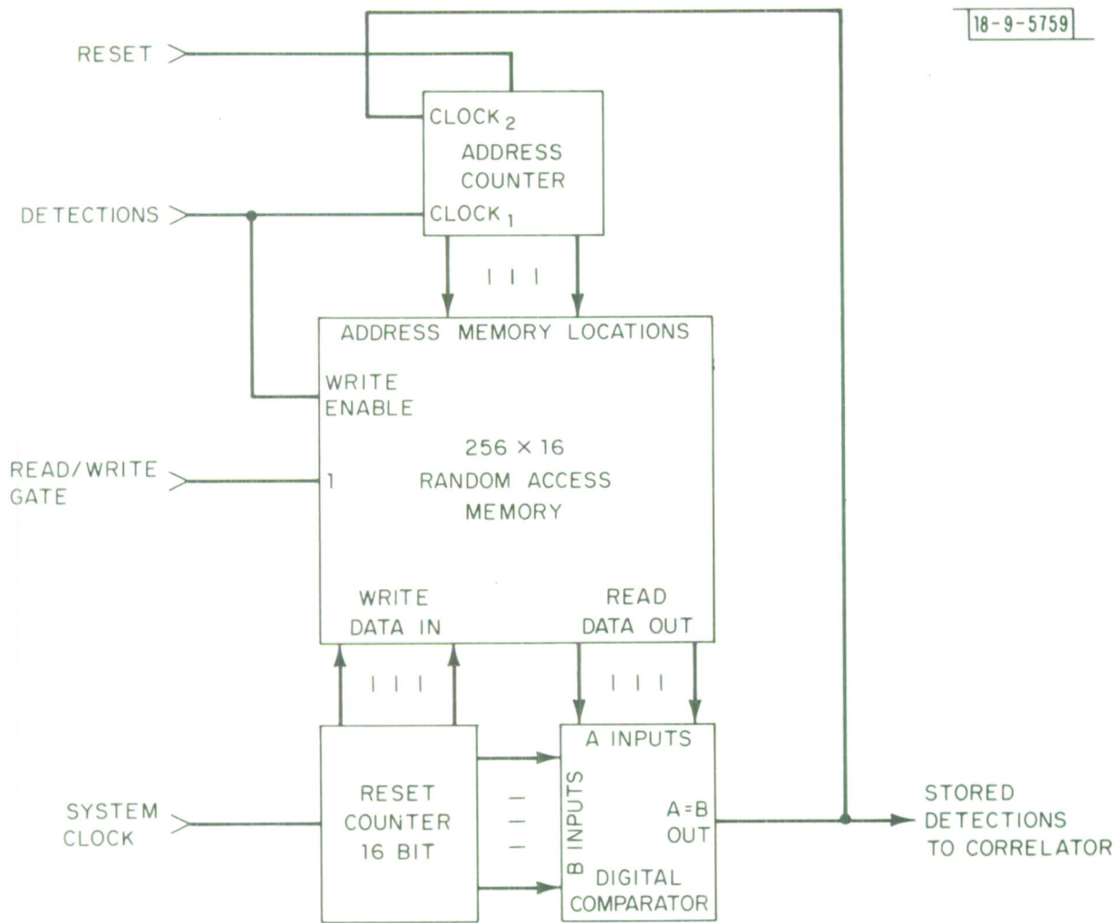
Fig. 21. Correlator memory.
