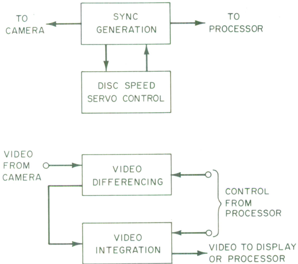
Fig. 9. Video and sync signal distribution system.
