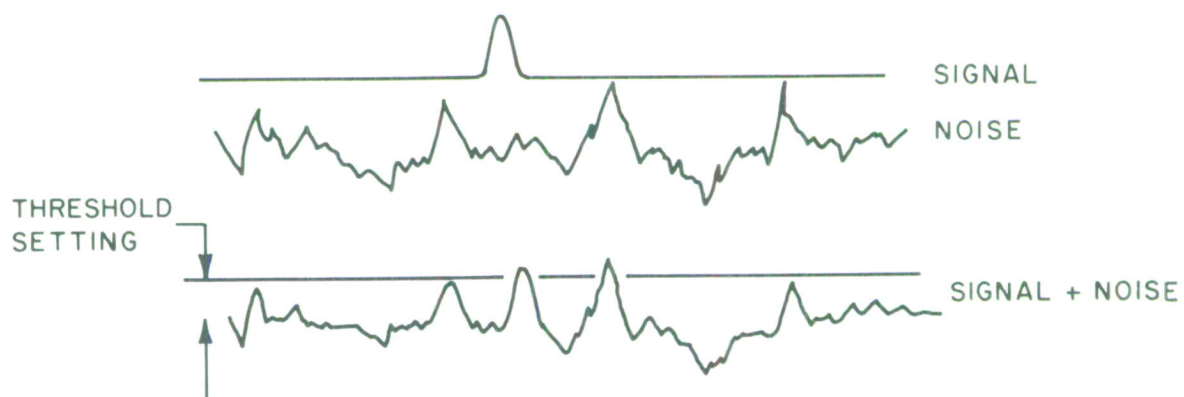
Fig. 12. Hypothetical video voltage waveforms (noise and signal + noise).
