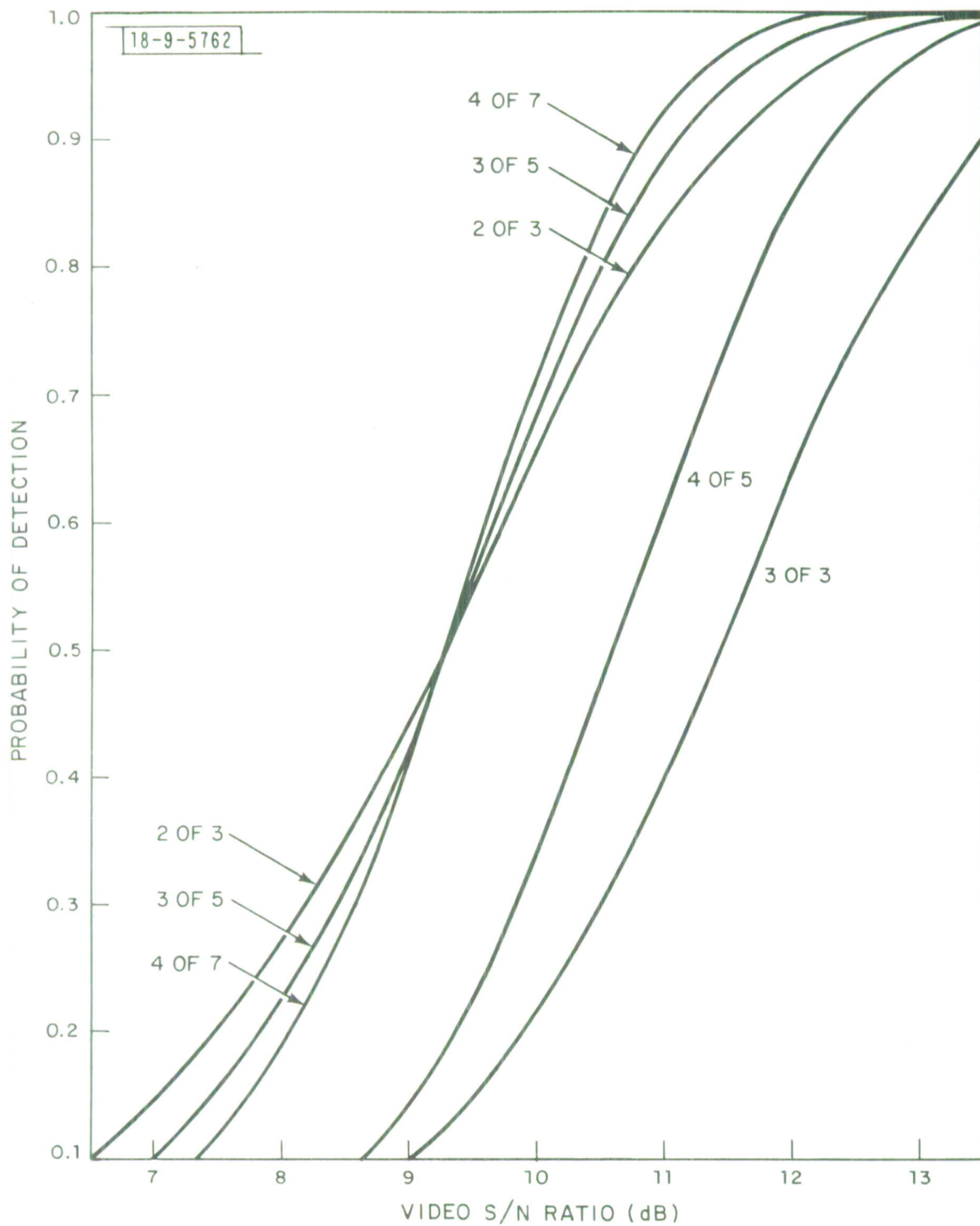
Fig. 25. Calculated probability of detection vs signal/noise.
