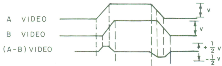
Fig. 3. Pictorial representation of timing errors.
