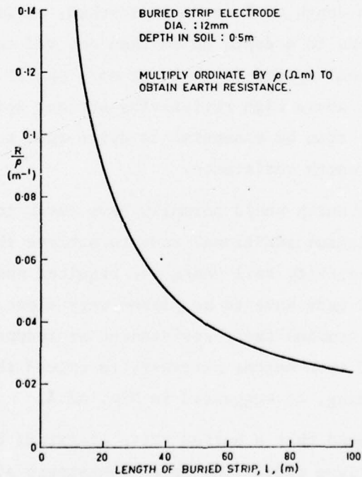
Fig. A4.2 Relation between earth resistance of buried strip 12mm dia., buried 0.5m into ground, and length of strip.
