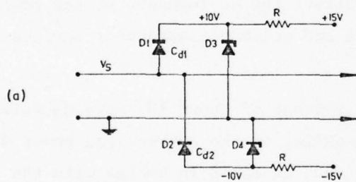
Fig. 30 Two forms of biased secondary protection for balanced signal transmission.
