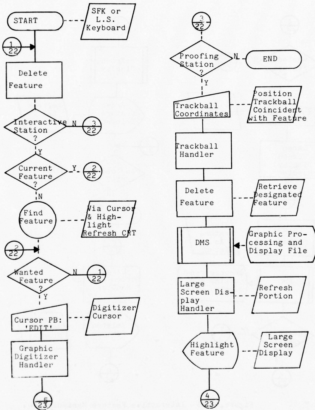
Figure III-25 - Interactive Feature Manipulation Delete Feature III-179 (Page 22 of 30)
