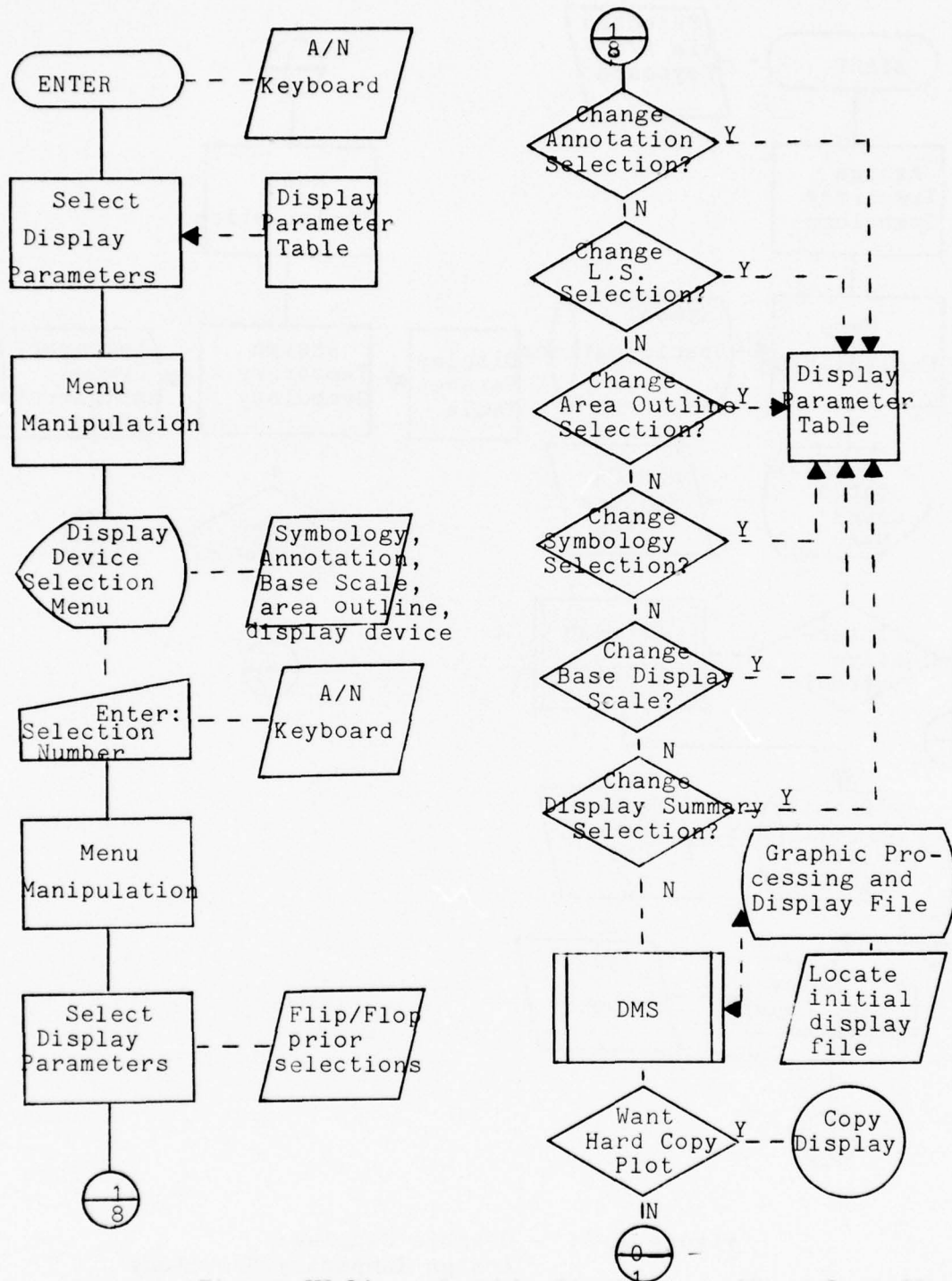
Figure III-24 - Graphic Display- (Page 8 of 22) Select Display Parameters III-137
