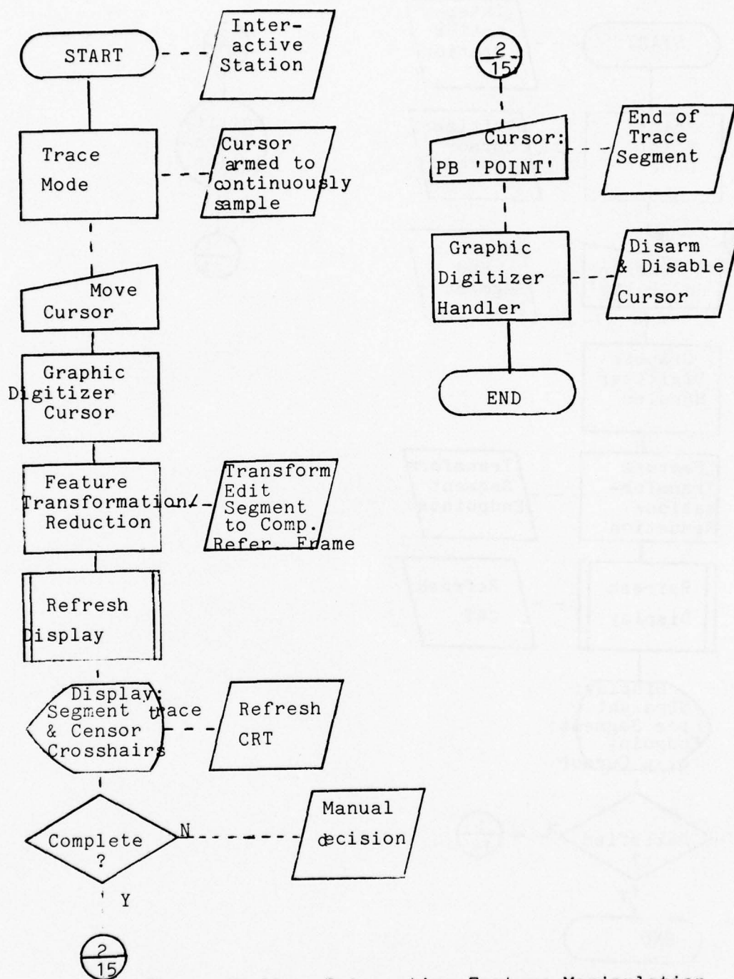
Figure III-25 - Interactive Feature Manipulation Trace Mode (Page 15 of 30)
