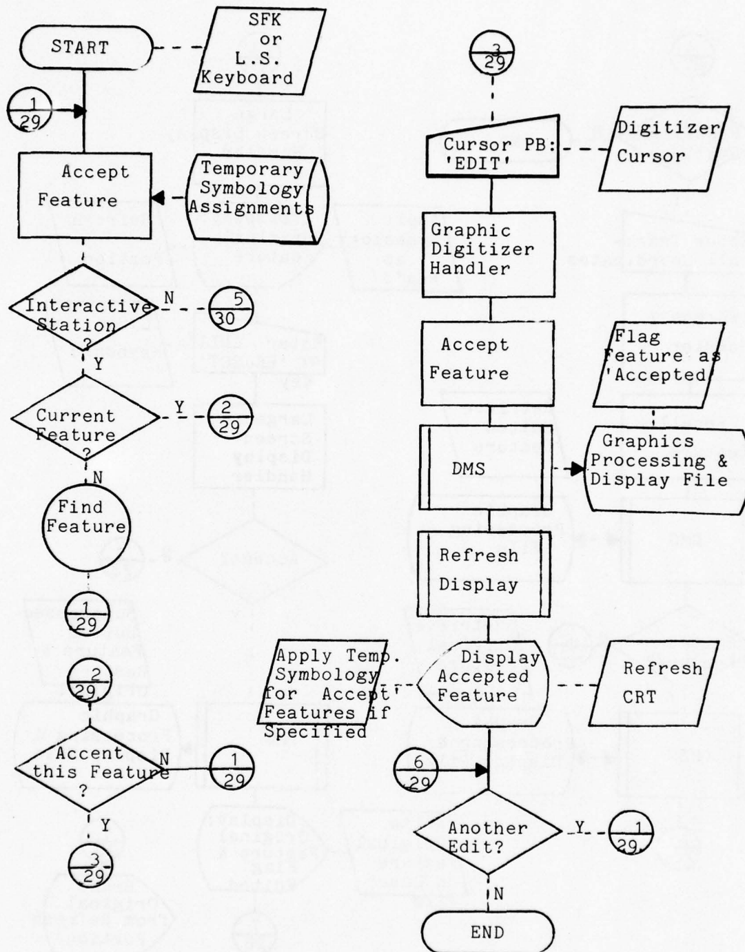
Figure III-25 - Interactive Feature Manipulation Accept Feature (Page 29 of 30)
