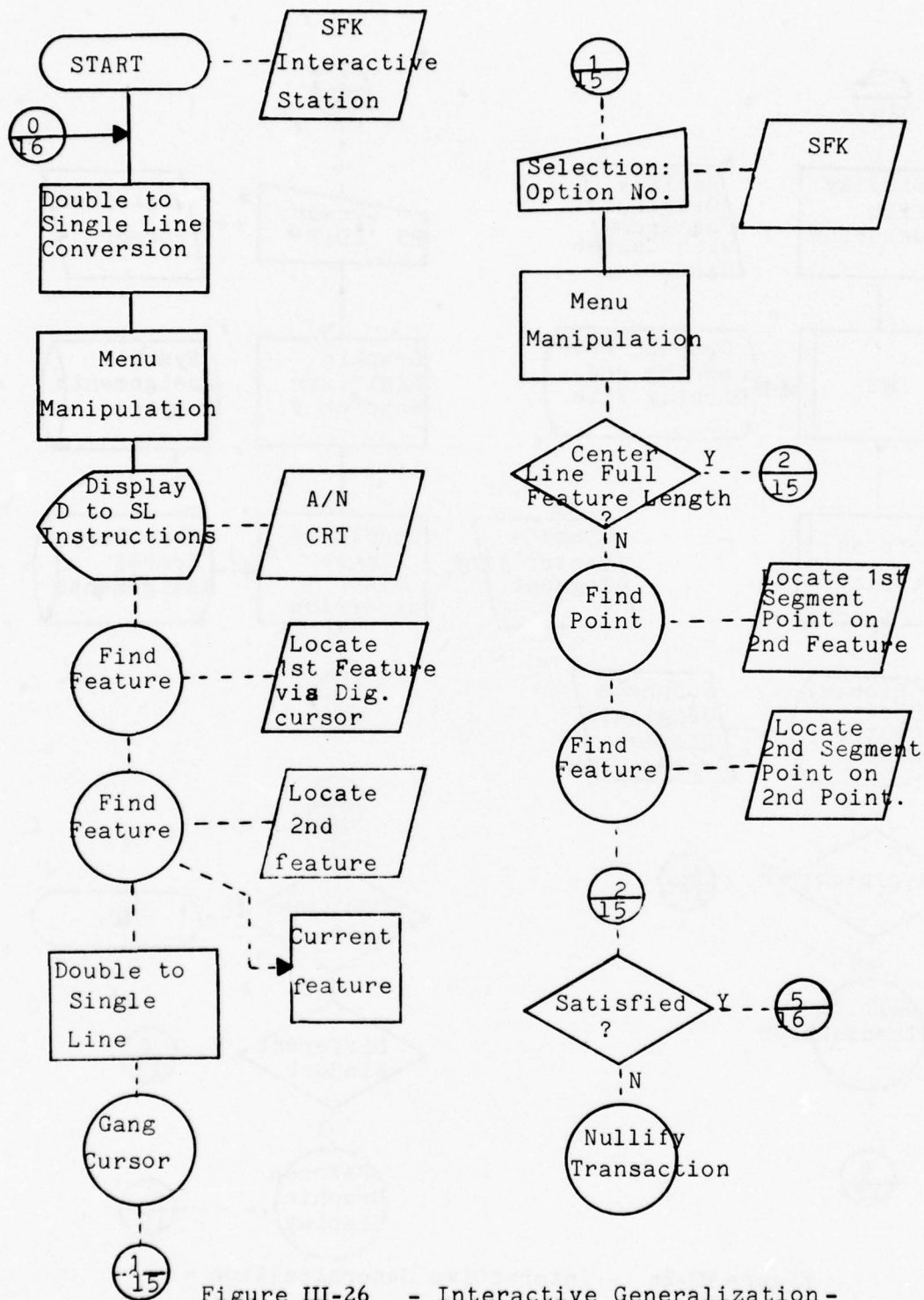
Figure III-26 - Interactive Generalization - Double to Single Line Conversion III-205 (Page 15 of 16)
