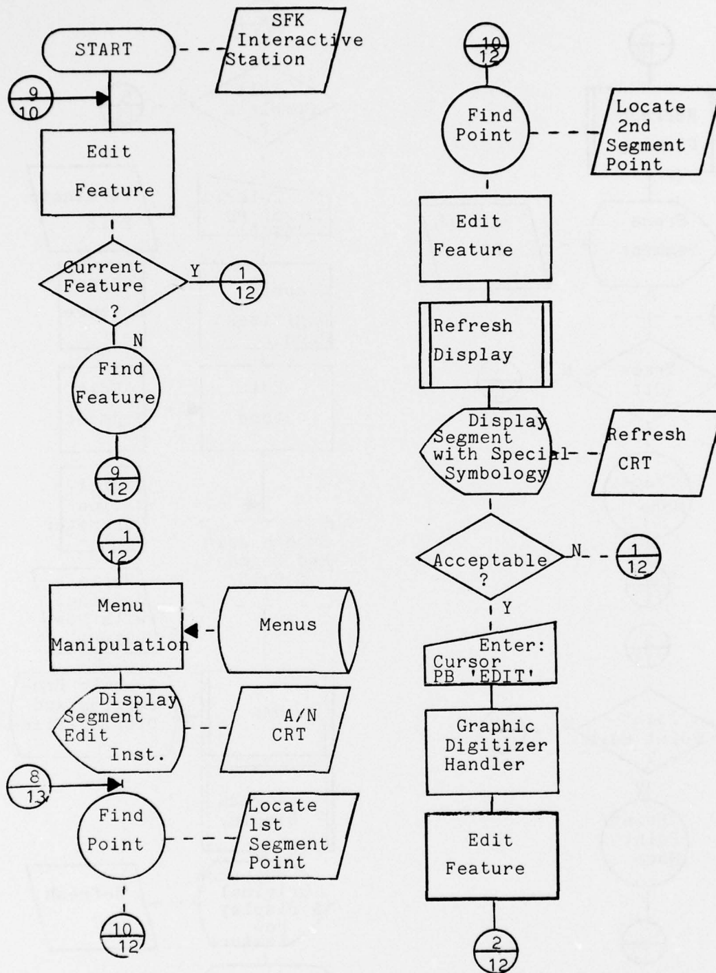
Figure III-25 - Interactive Feature Manipulation Edit Feature (Page 12 of 30) III-169
