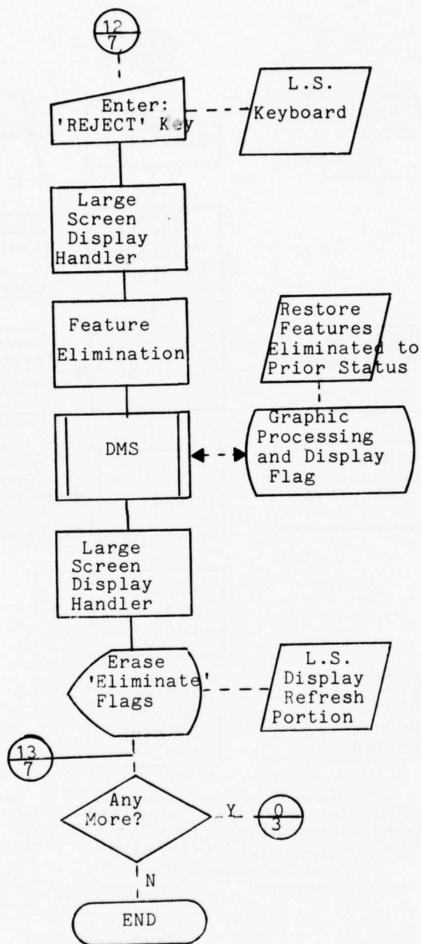
Figure III-26 - Interactive Generalization Feature Elimination (Page 8 of 16)
