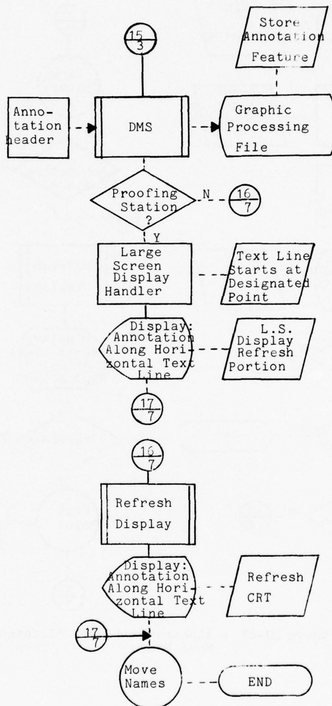
Figure III-27 - Alphanumeric Text Placement- Names Placement (Page 7 of 14) III-215
