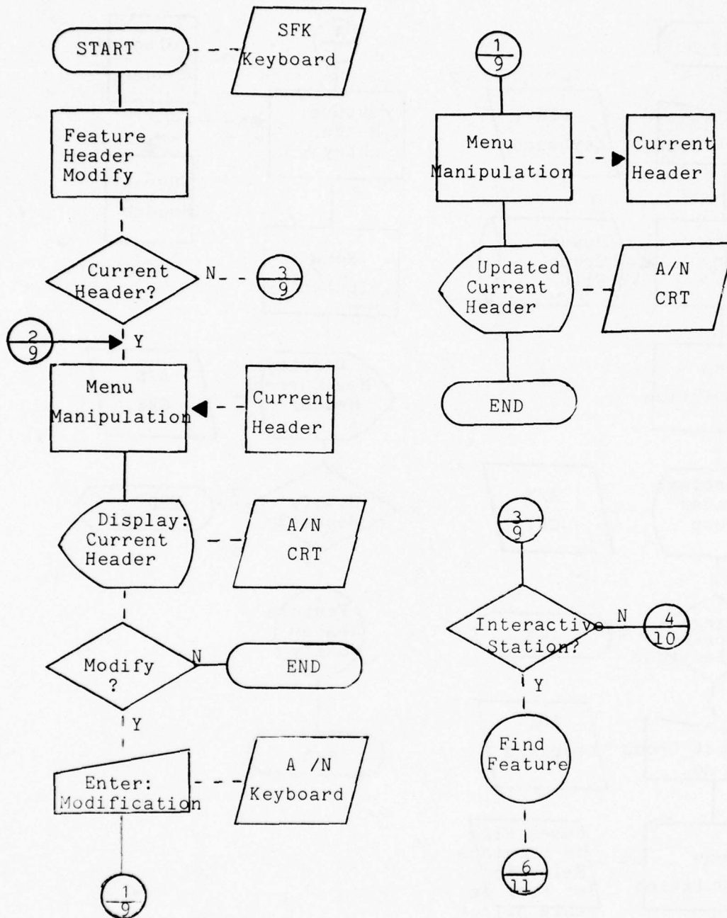
Figure III-23 - Graphic Data Extraction- Feature Header Modify (Page 9 of 11)
