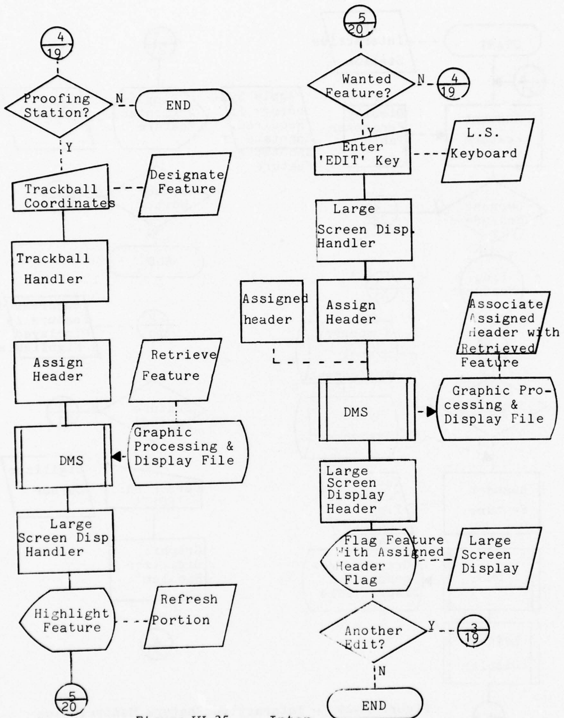
Figure III-25 - Inter- active Feature Manipulation III-177 Assign Header (Page 20 of 30)
