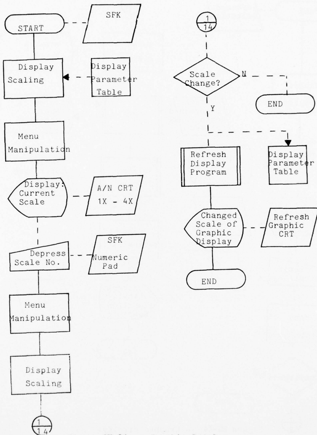
Figure III-24 - Graphic Display- Refresh Display Scale
