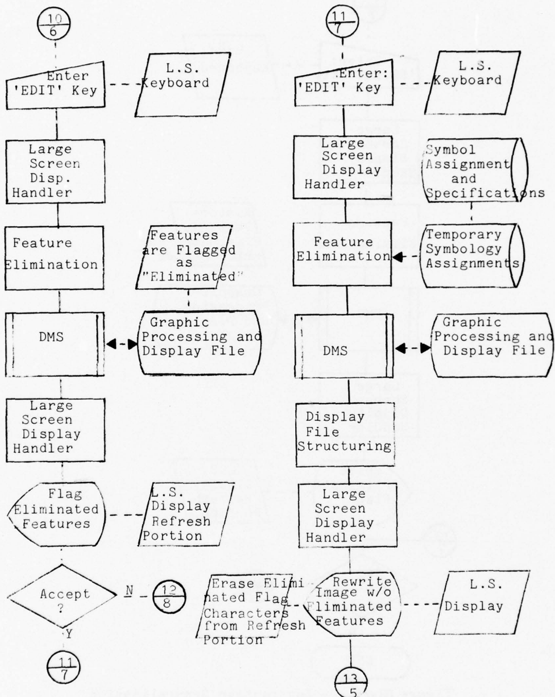
Figure III-26 - Interactive Generalization Feature Elimination (Page 7 of 16)
