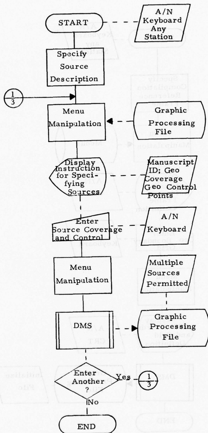
Figure III-21 - Source Assessment - Specify Source Description (Page 3 of 7) III-106
