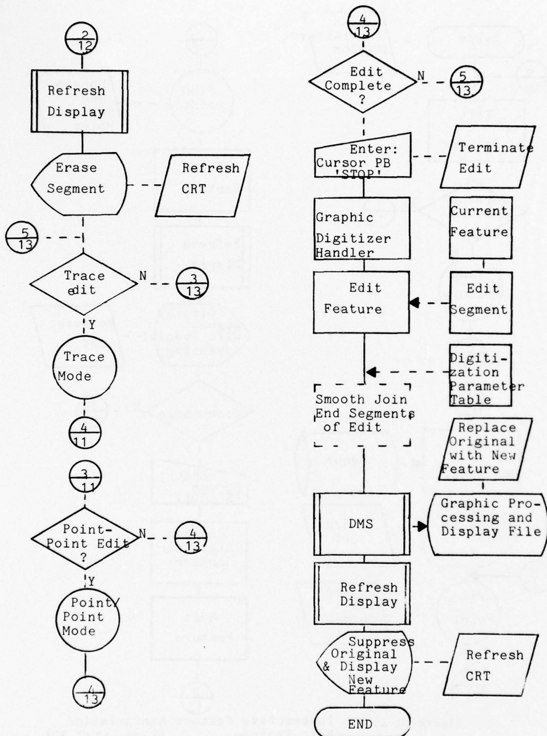
Figure III-25 - Interactive Feature Manipulation Edit Feature (Page 13 of 30) III-170
