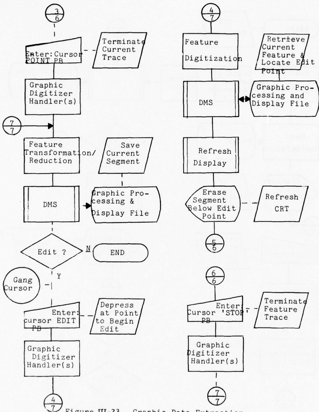
Figure III-23 Graphic Data Extraction- Feature Digitization (Page 7 of 11) III-122
