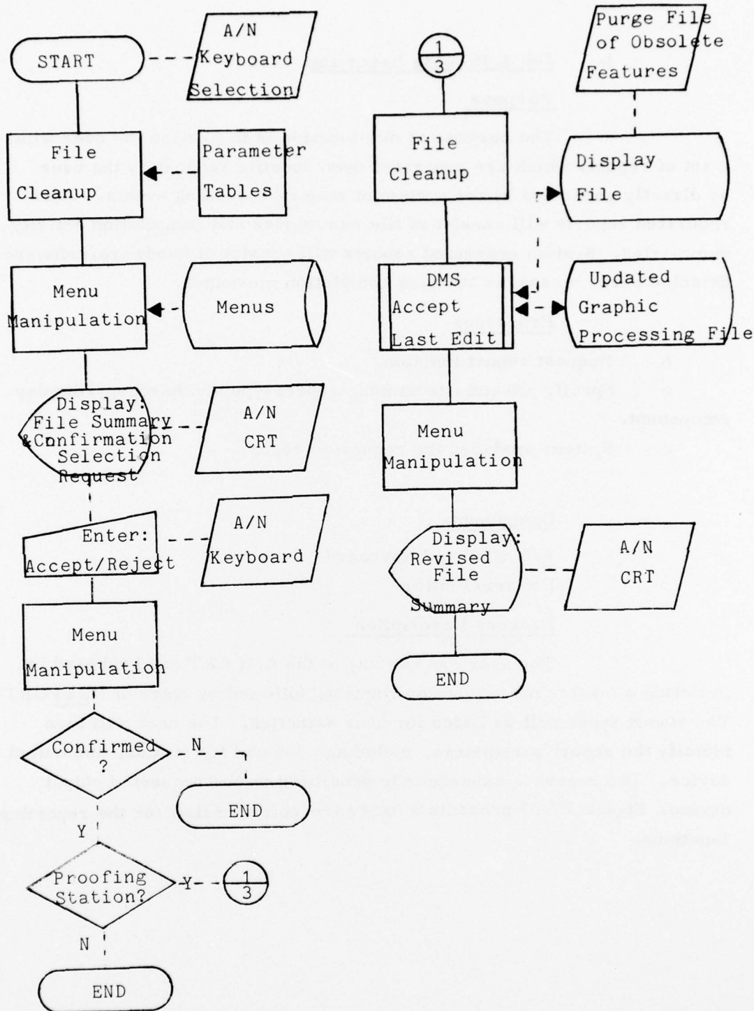
Figure III-28 - System Services - File Cleanup (Page 3 of 3)
