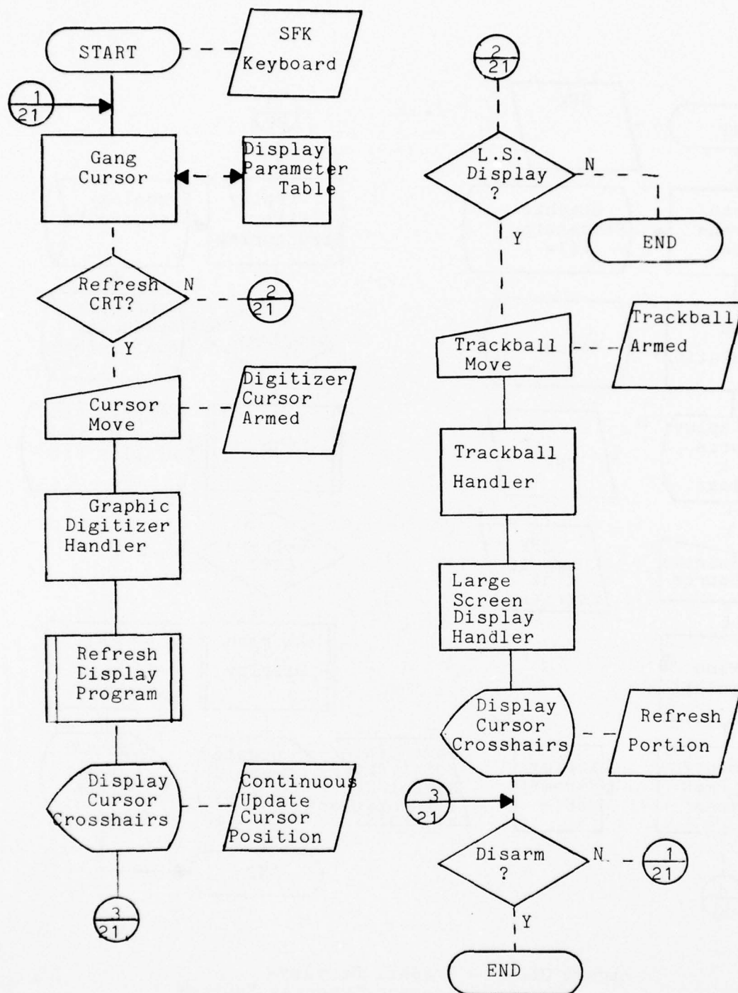
Figure III-24 - Graphic Display- Gang Cursor
