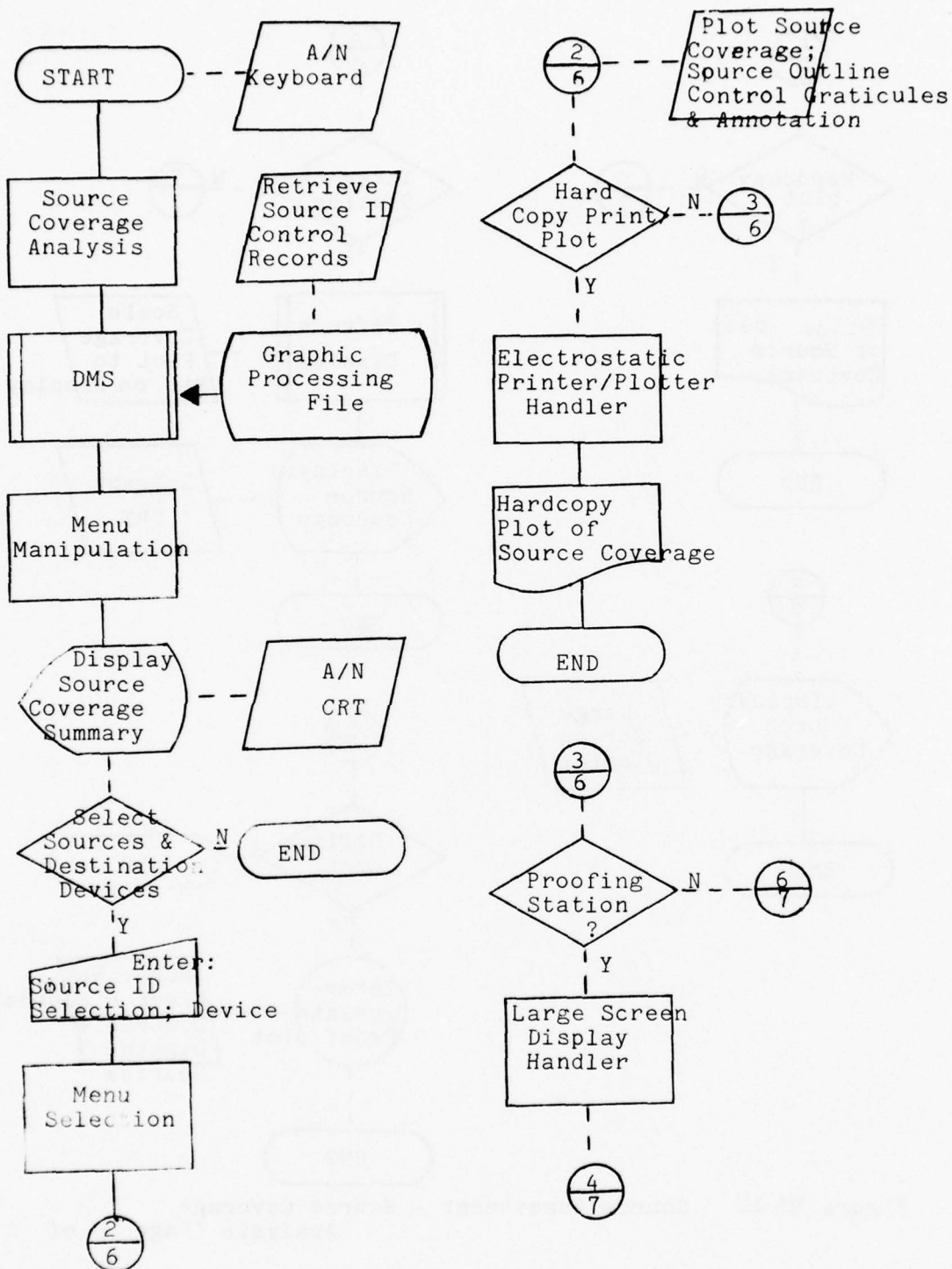
Figure III-21 Source Assessment-Source Coverage Analysis (Page 6 of 7)
