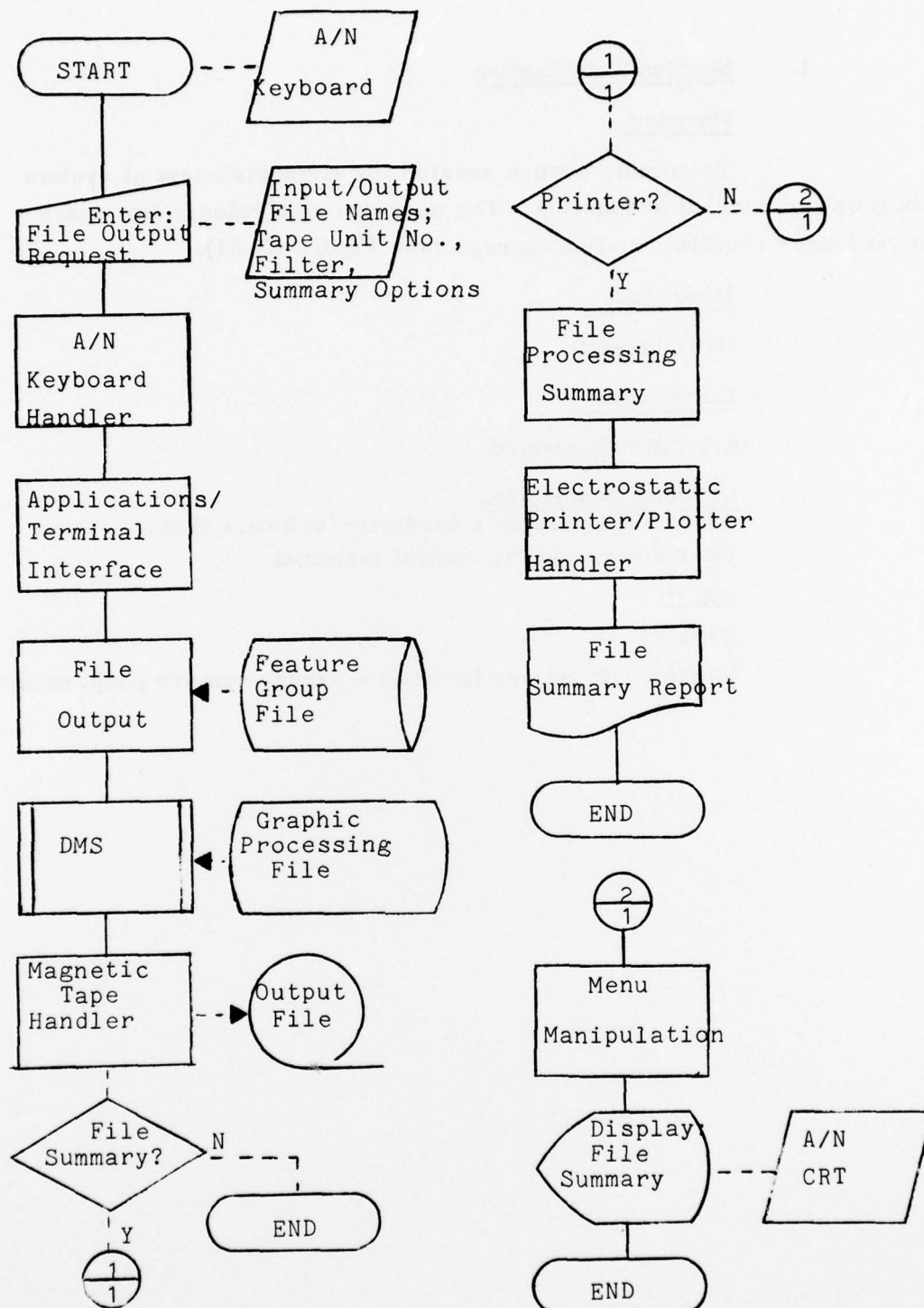
Figure III-30 - Output Processing (Page 1 of 1) III-231
