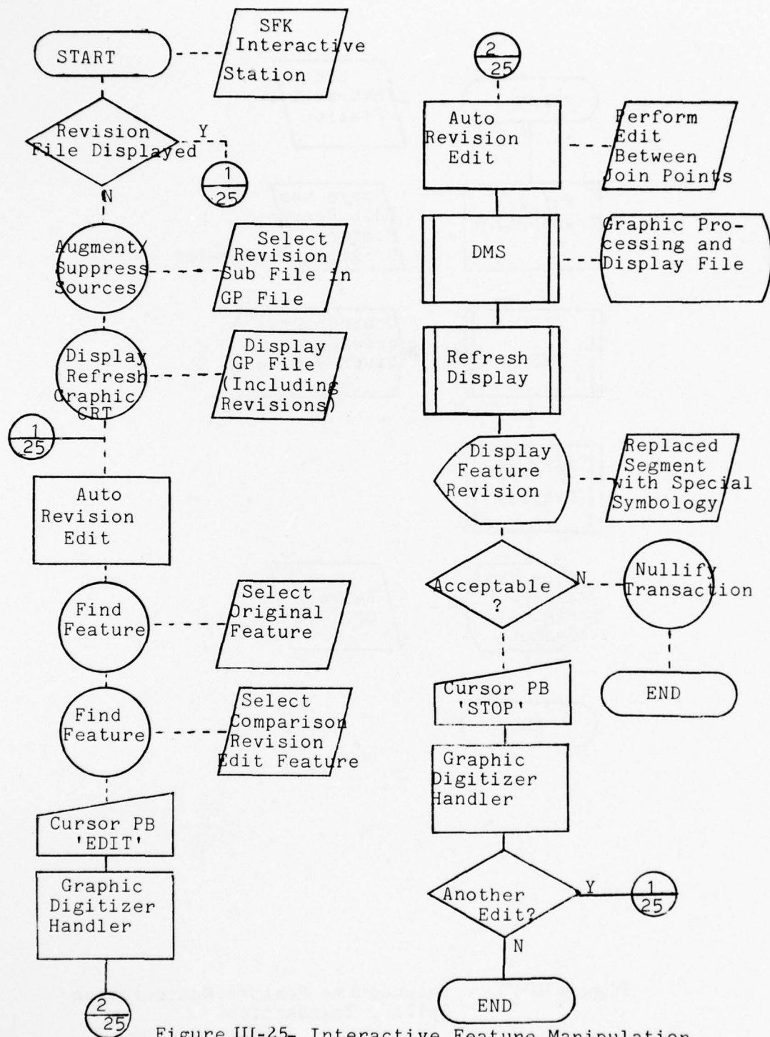
Figure III-25- Interactive Feature Manipulation Auto Revision Edit (Page 25 of 30) III-182
