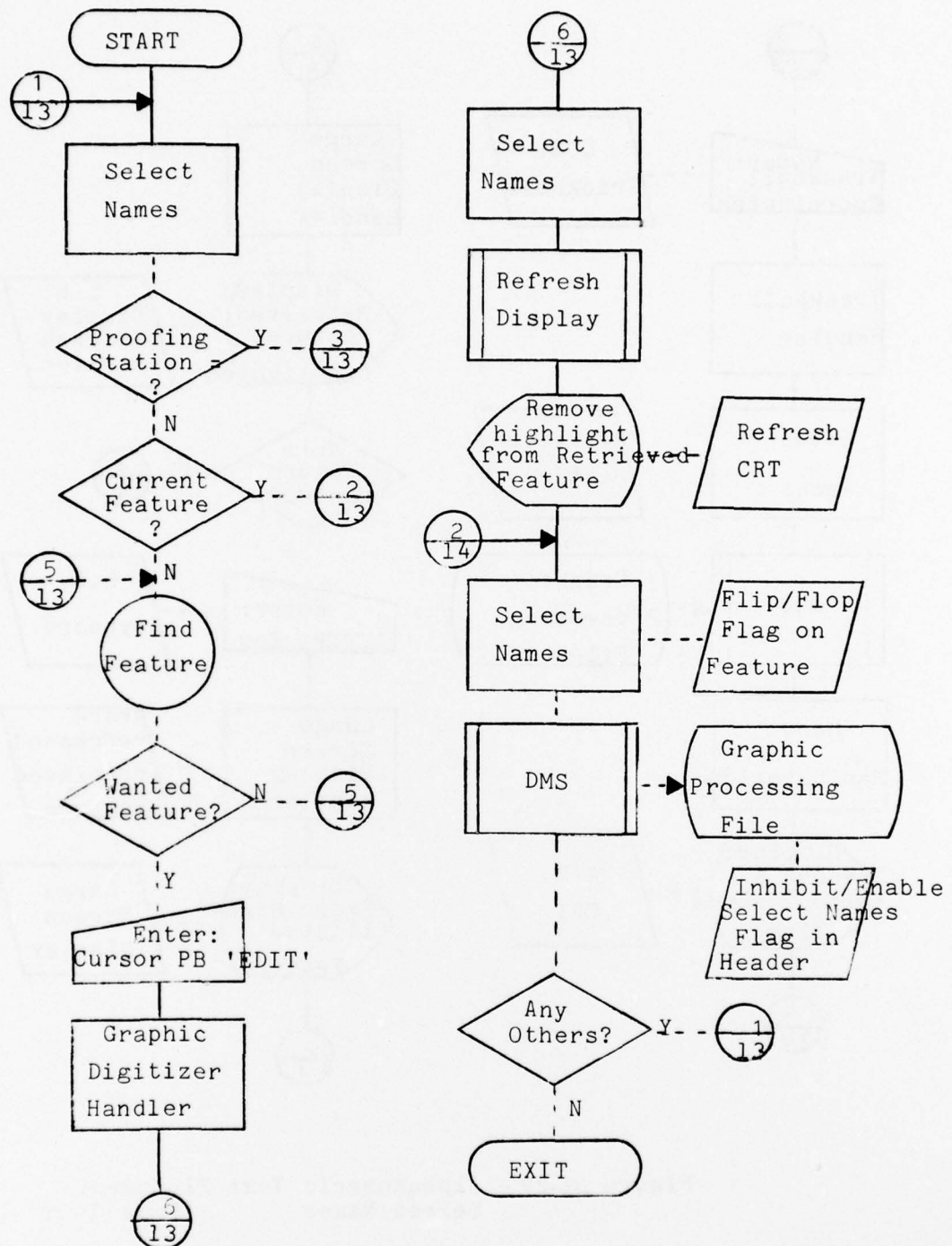
Figure III-27 - Alphanumeric Text Placement- Select Names (Page 13 of 14) III-221
