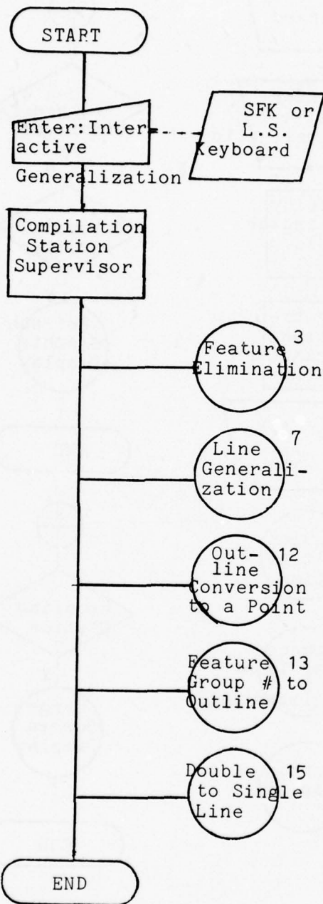
Figure III-26 - Interactive Generalization (Page 2 of 16)
