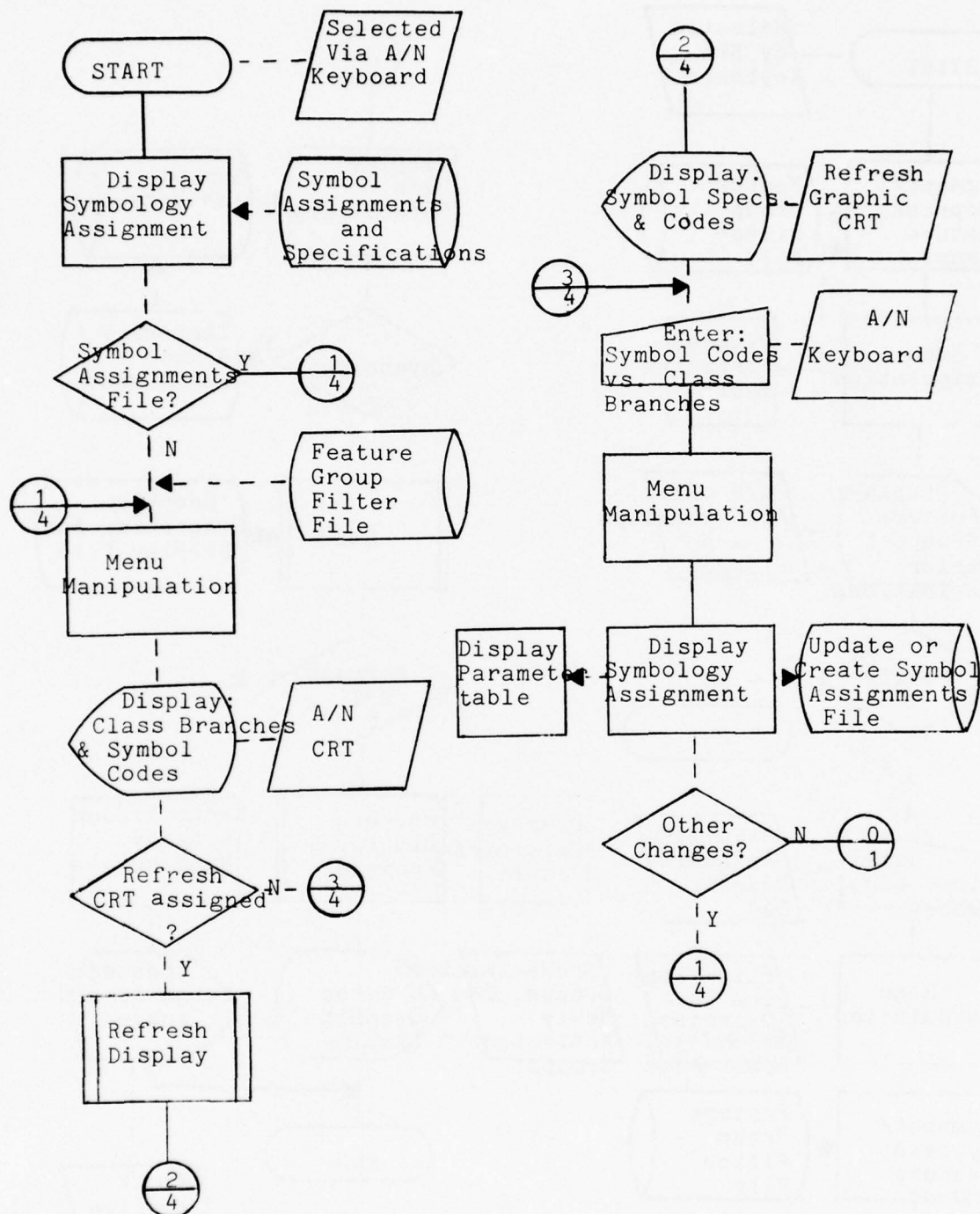
Figure III-24 - Graphic Display-Assign Symbology
