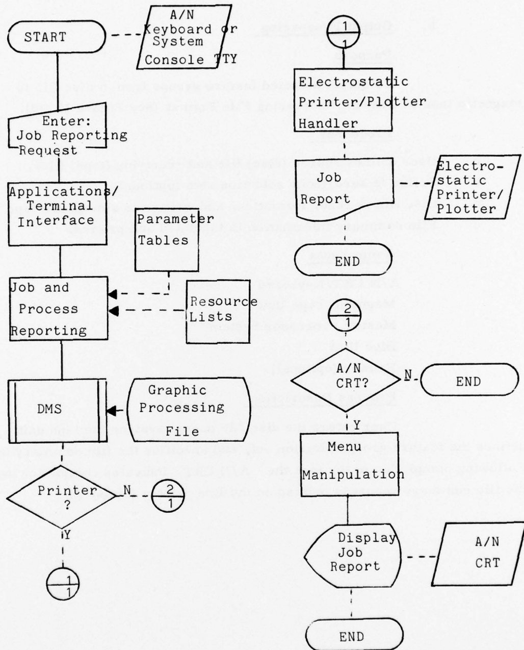
Figure III-29 - Job Reporting
