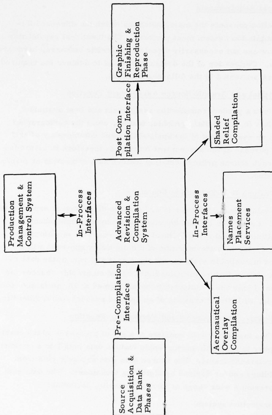
Figure I-2 System Interfaces
