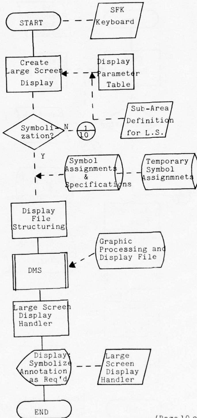
Figure III-24 - Graphic Display - Large Screen Display Hard Copy Display III-139 (Page 10 of 22)
