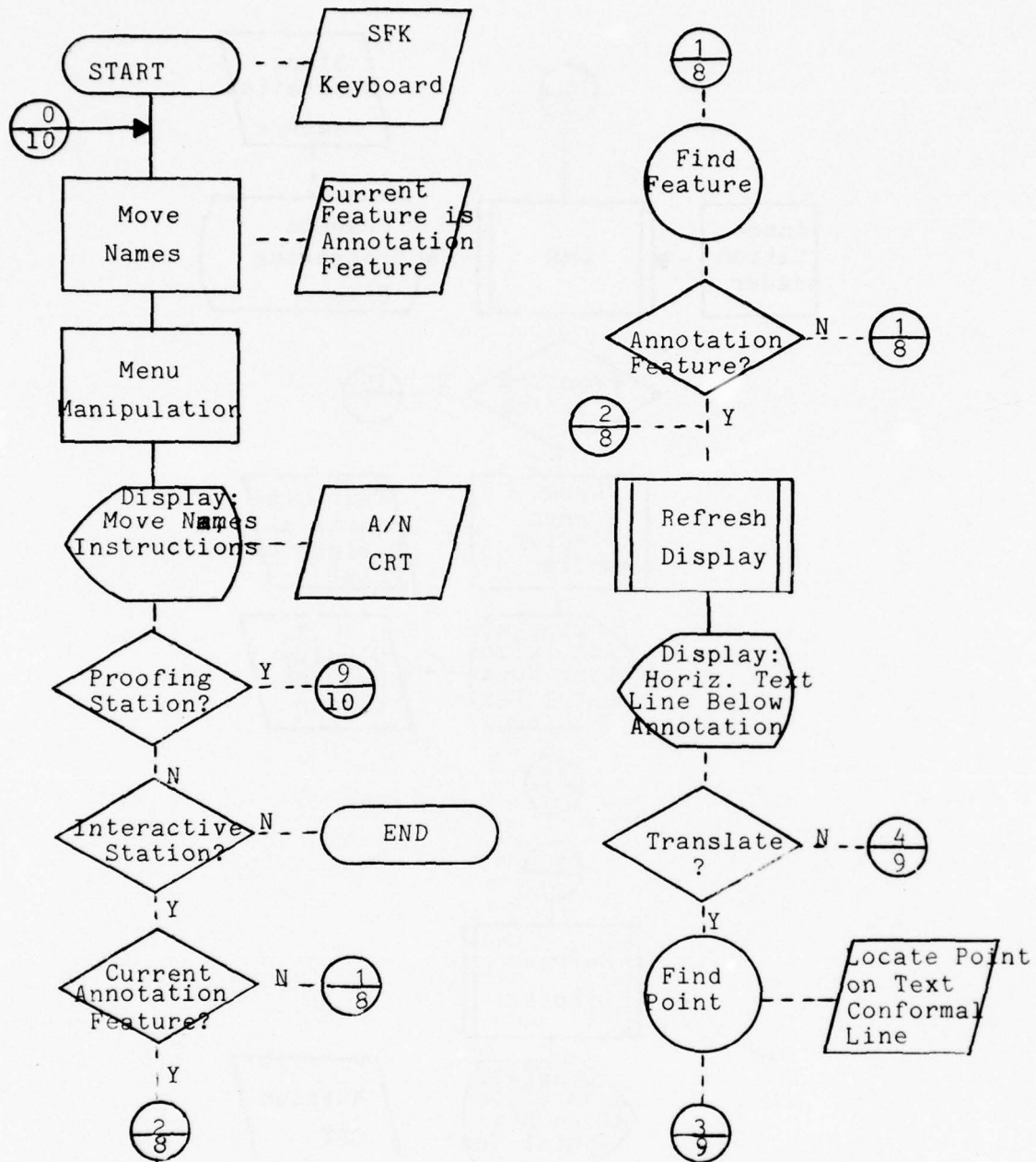
Figure III-27 - Alphanumeric Text Placement - Move Names (Page 8 of 14)
