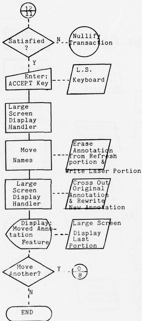
Figure III-27 - Alphanumeric Text Placement - Move Names (Page 12 of 14)
