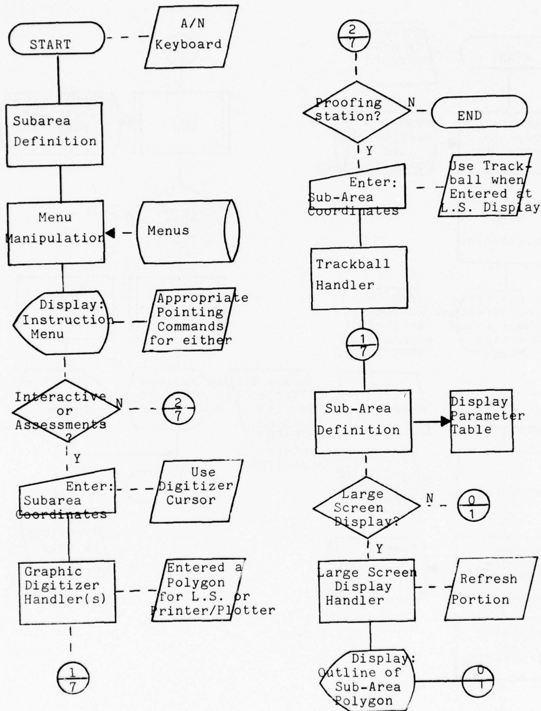
Figure III-24 - Graphic Display - Sub-Area Definition III-136
