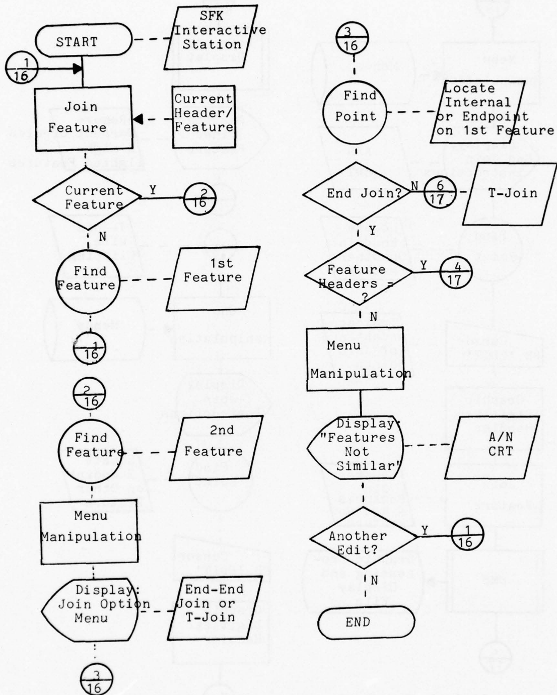
Figure III-25 - Interactive Feature Manipulation Join Feature (Page 16 of 30)
