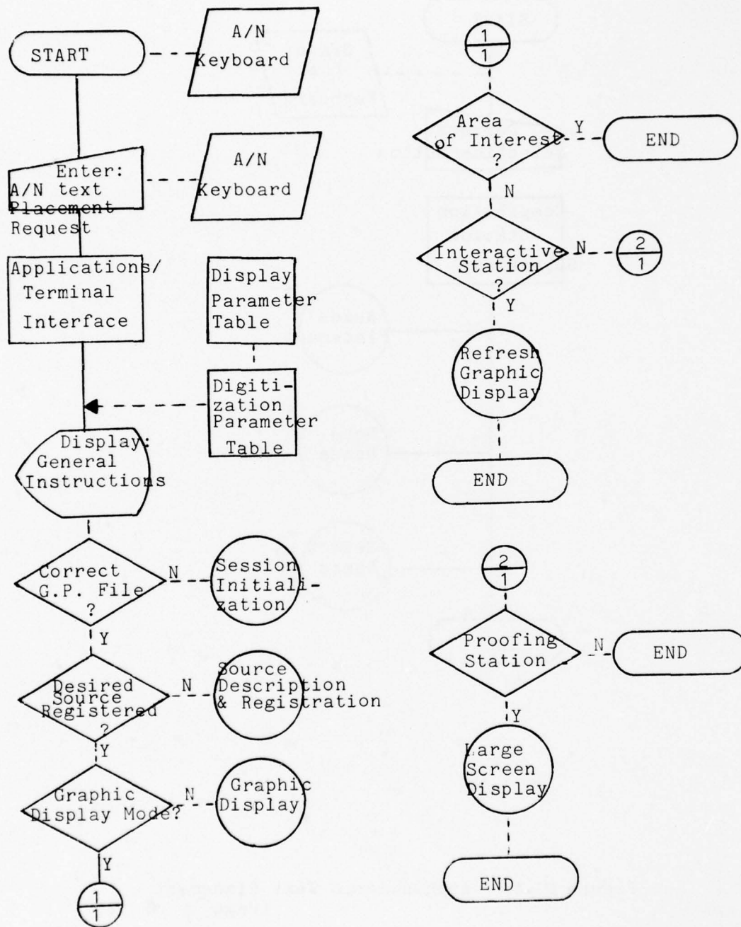
Figure III-27 - Alphanumeric Text Placement (Page 1 of 14)
