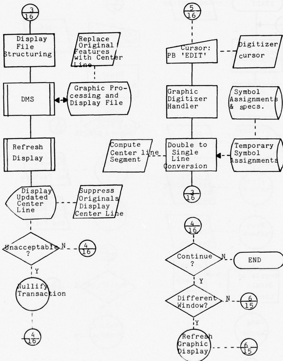
Figure III-26 - Interactive Generalization - Double to Single Line Conversion III-206 (Page 16 of 16)
