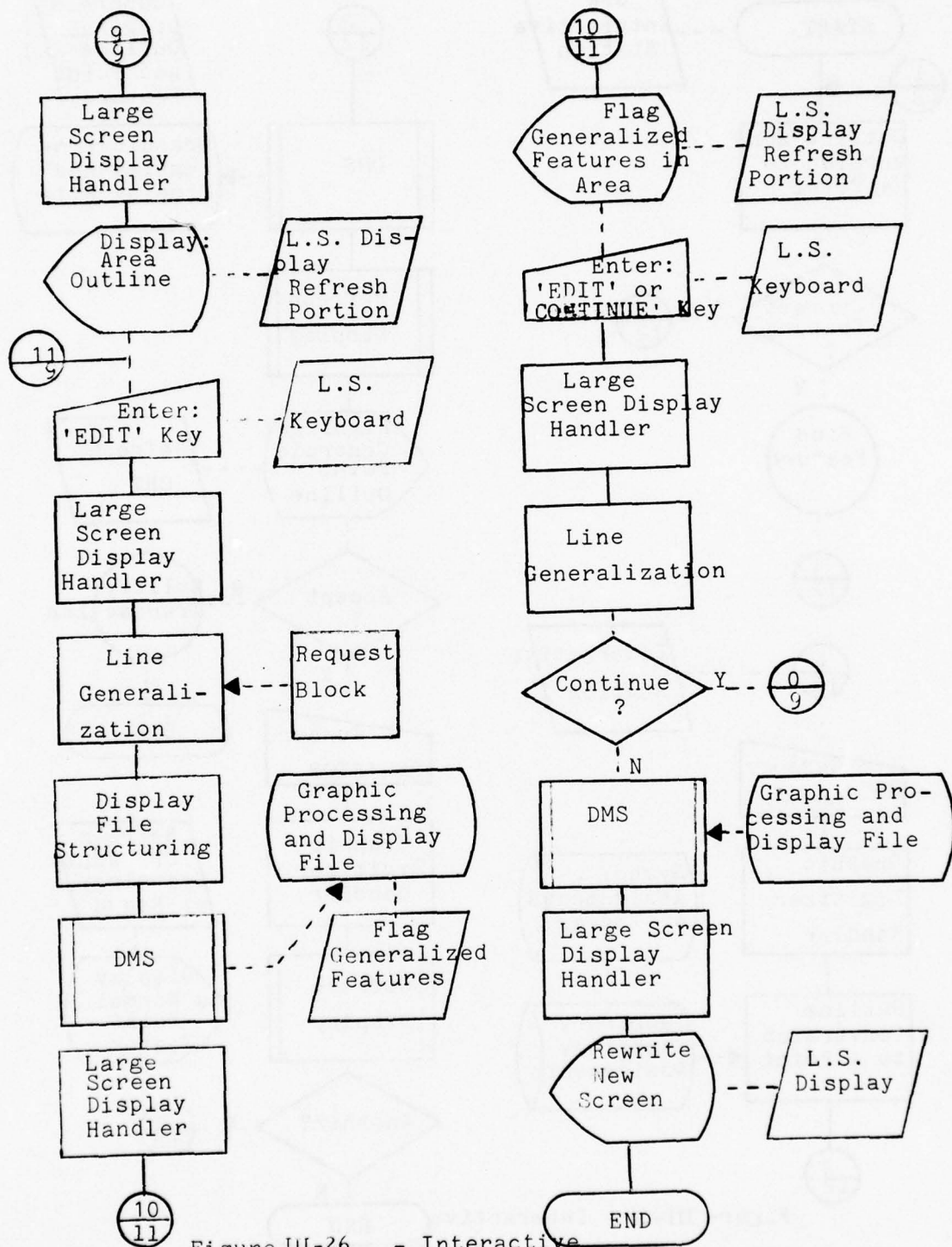
Figure III-26 - Interactive Generalization-Line Generalization III-201 (Page 11 of 16)
