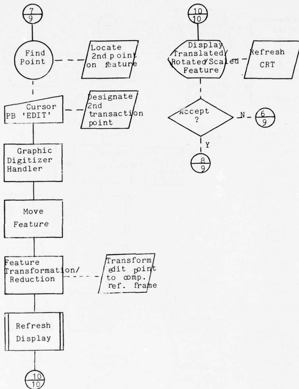
Figure III-25 - Interactive Feature Manipulation - Move Feature (Page 10 of 30)
