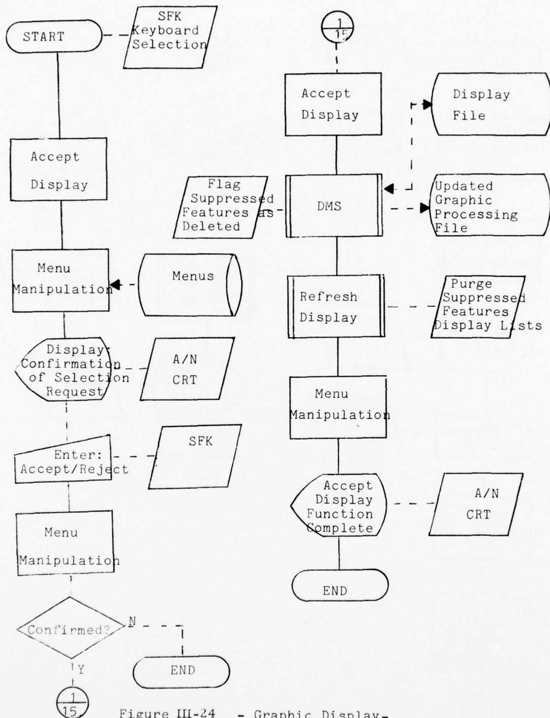
Figure III-24 - Graphic Display - Accept Display - (Page 15 of 22) III-144
