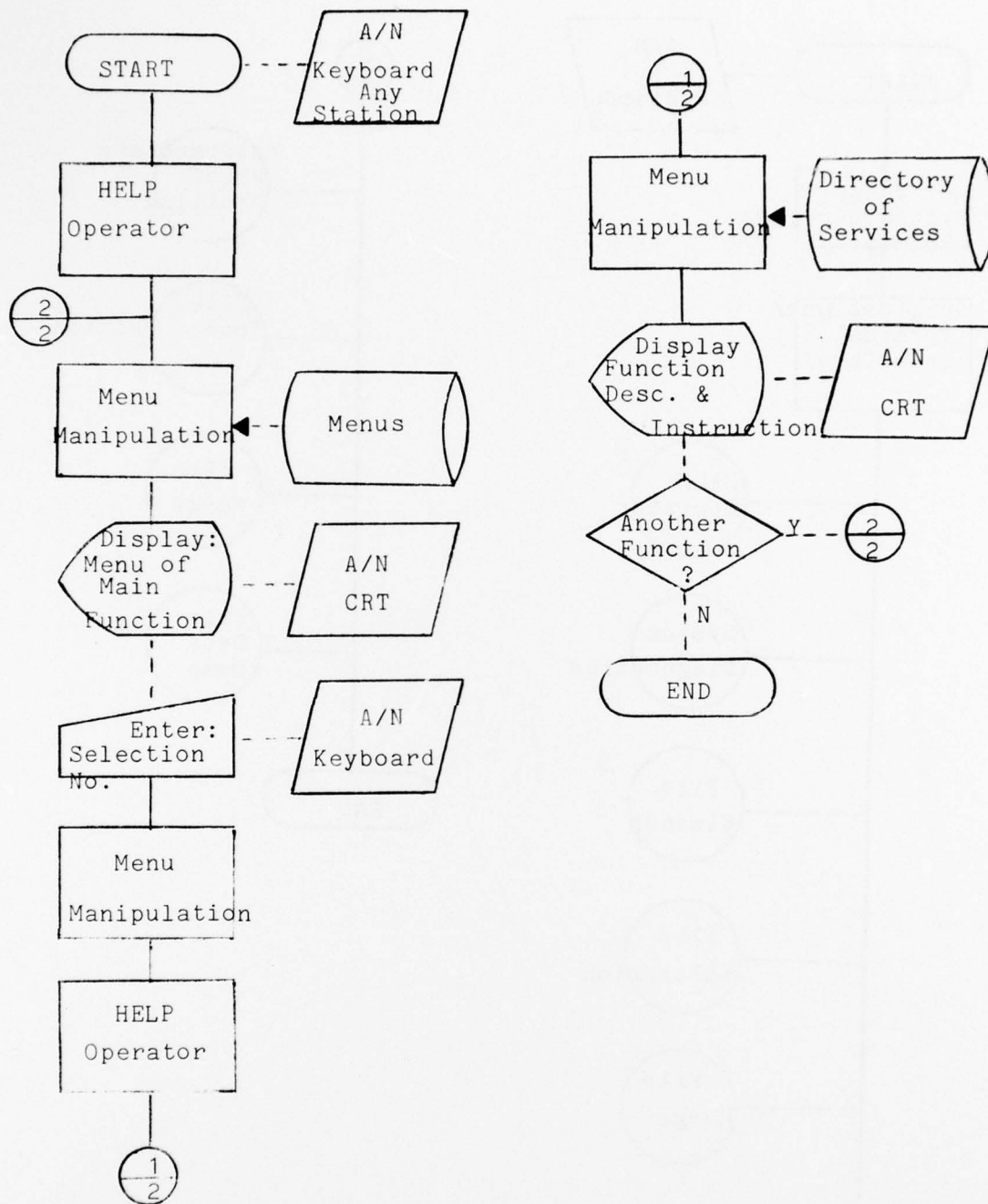
Figure III-28 - System Services - HELP Operator
