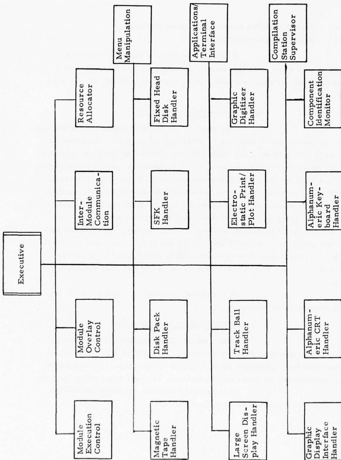
Figure III-4 Executive Program
