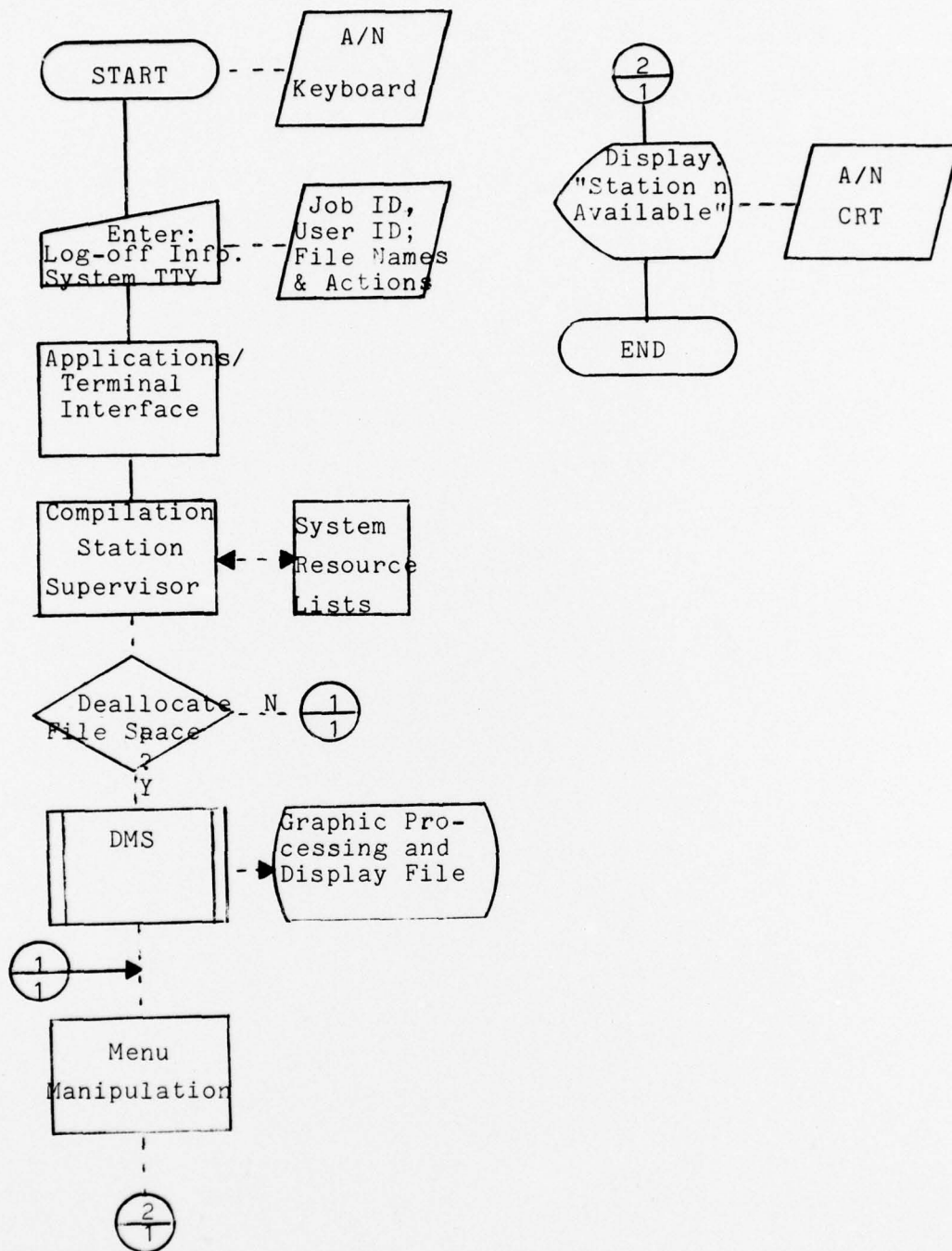
Figure III-31 - Session Termination
