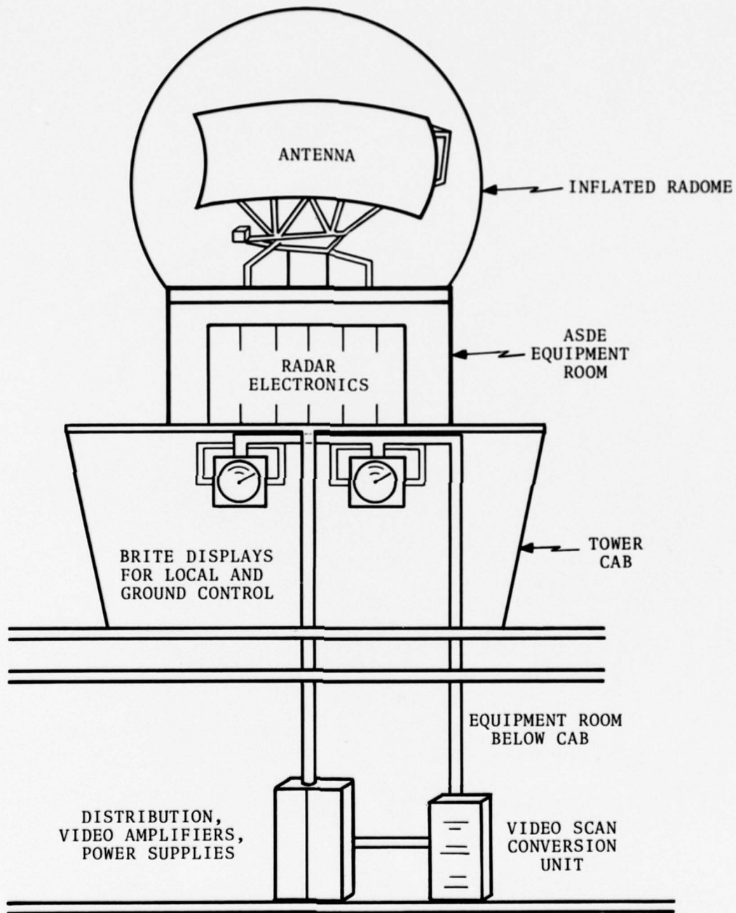
FIGURE 5.2-1. ASDE-2 EQUIPMENT LAYOUT
