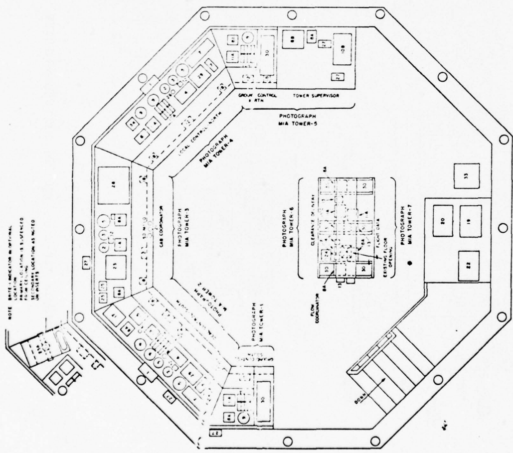
FIGURE 4.6-3. LAYOUT OF MIAMI TOWER
