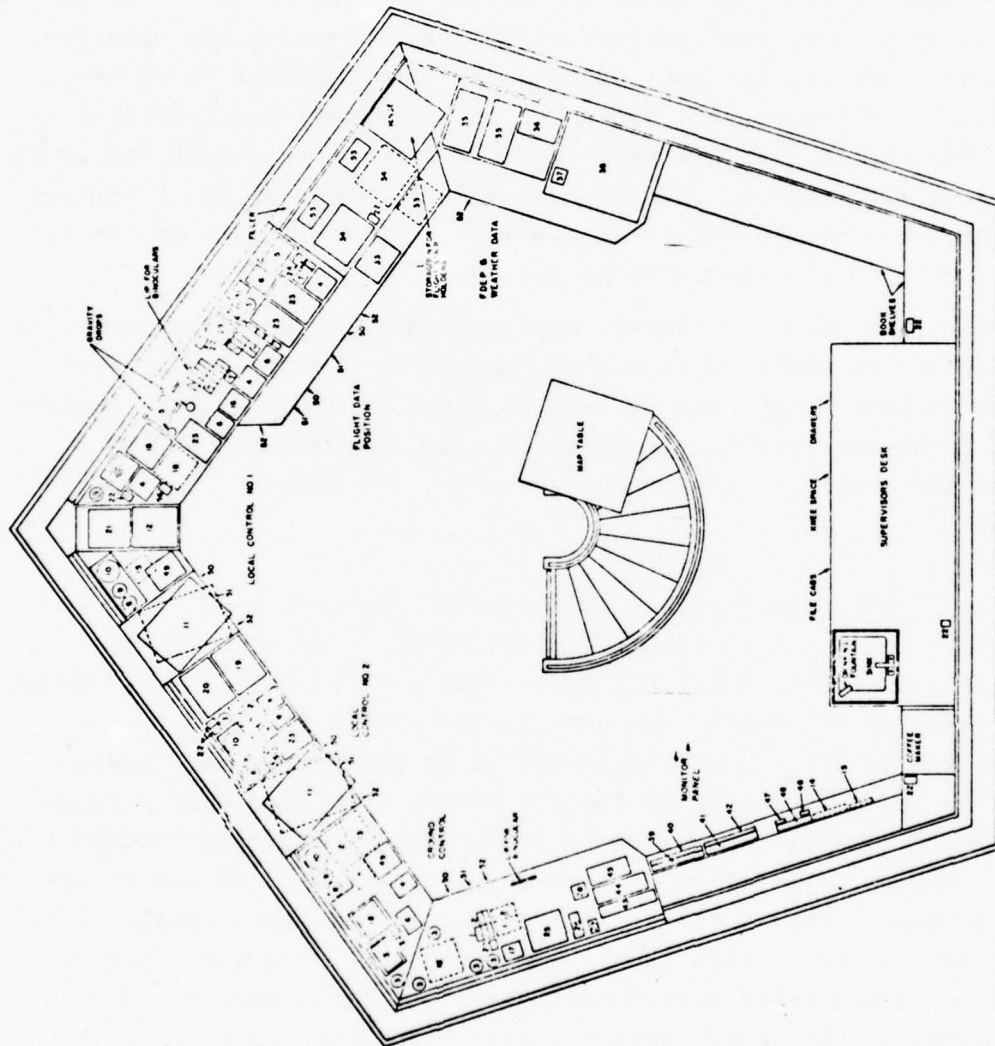
FIGURE 4.6-6. LAYOUT OF HOUSTON TOWER
