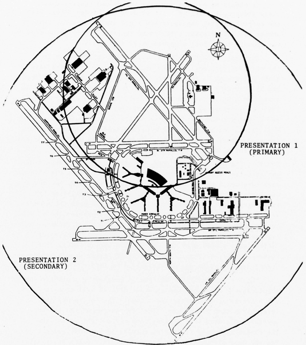
FIGURE 5.2-6. TYPICAL PRESENTATIONS FOR NORTH LOCAL CONTROL AT O'HARE
