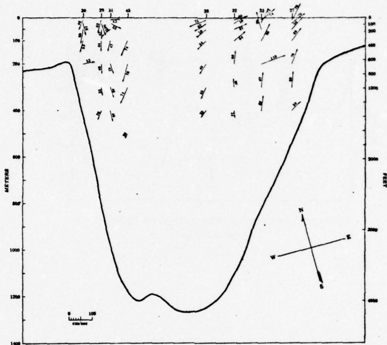
FIGURE 11 MAXIMUM OBSERVED VELOCITY VECTORS CROSS SECTION A
