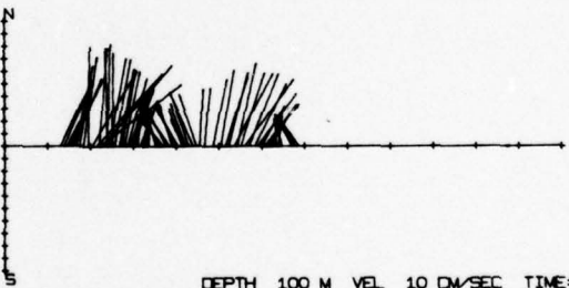
DEPTH 100 M VEL 10 CM/SEC TIME = 4 HRS/DIV
