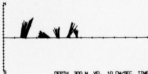
DEPTH 300 M VEL 10 CM/SEC TIME = 4 HRS/DIV
