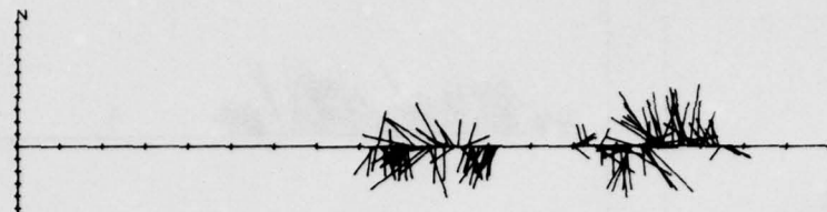
DEPTH 10 M VEL 5 CM/SEC TIME = 4 HRS/DIV
