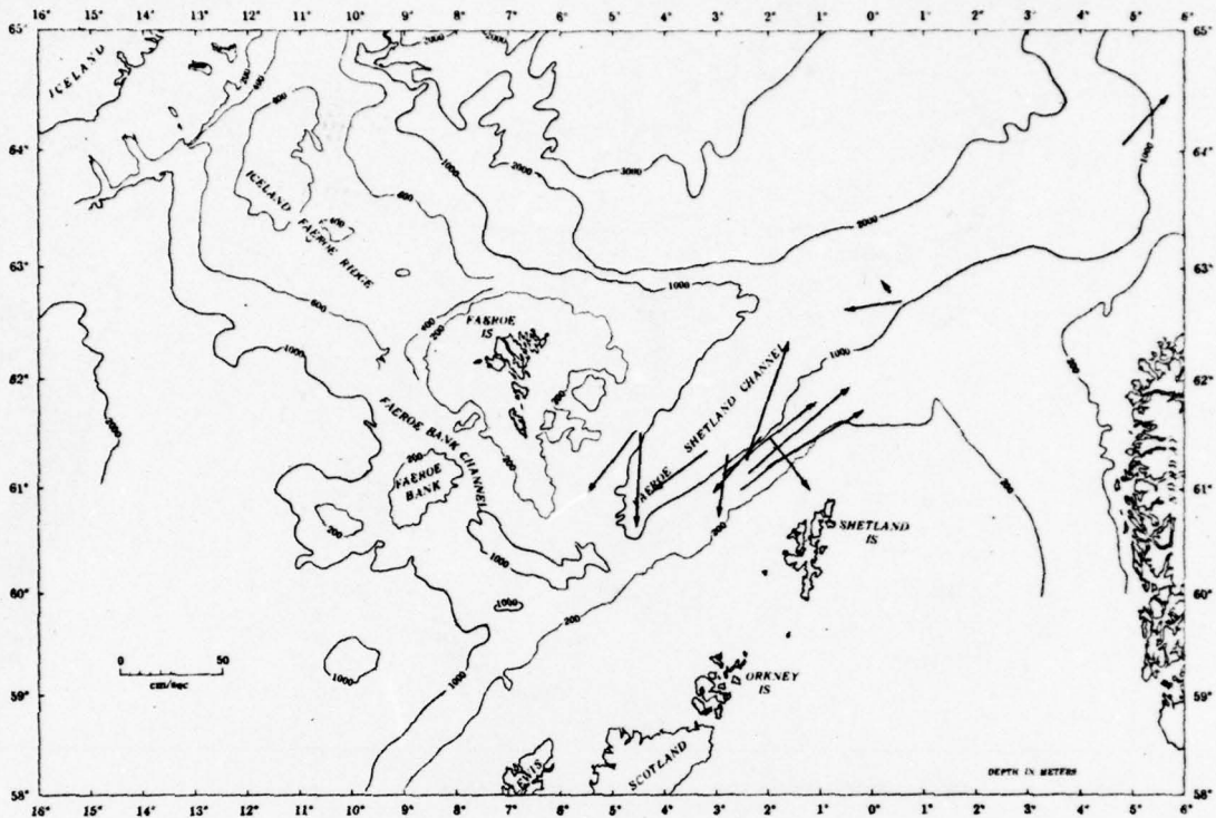
FIGURE 6 MAXIMUM VELOCITY VECTORS AT 400 METERS
