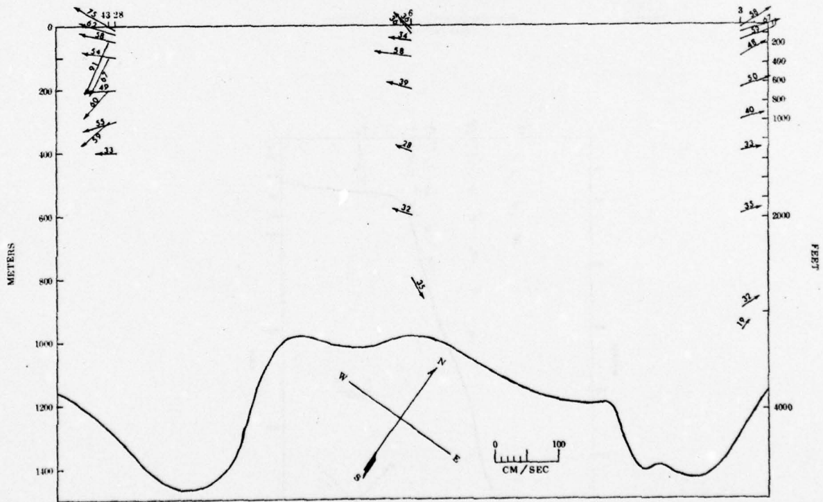
MAXIMUM OBSERVED VELOCITY VECTORS CROSS SECTION D
