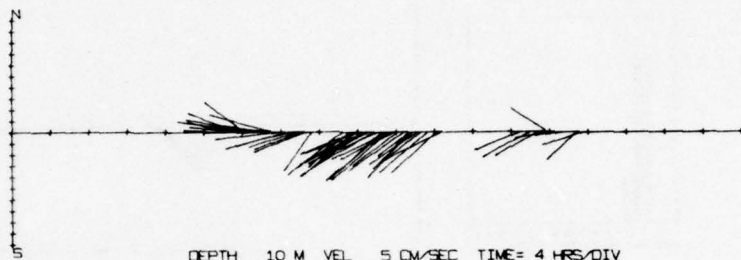
DEPTH 10 M VEL 5 CM/SEC TIME = 4 HRS/DIV
