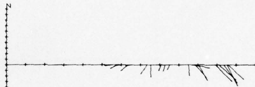
DEPTH 100 M VEL 5 CM/SEC TIME = 4 HRS/DIV
