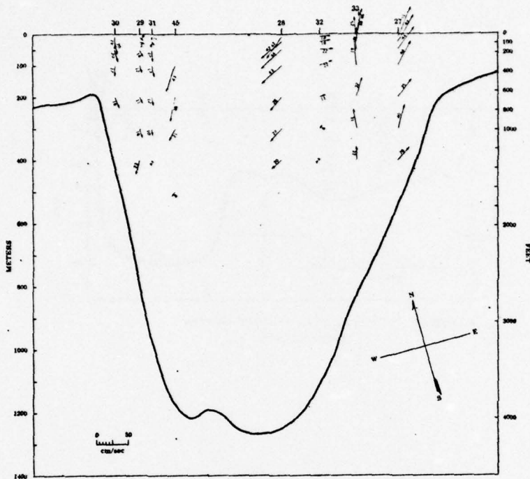
FIGURE 8 VECTIORIAL MEAN VELOCITY VECTORS CROSS-SECTION A
