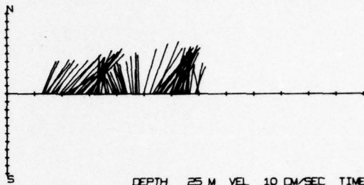
DEPTH 25 M VEL 10 CM/SEC TIME = 4 HRS/DIV
