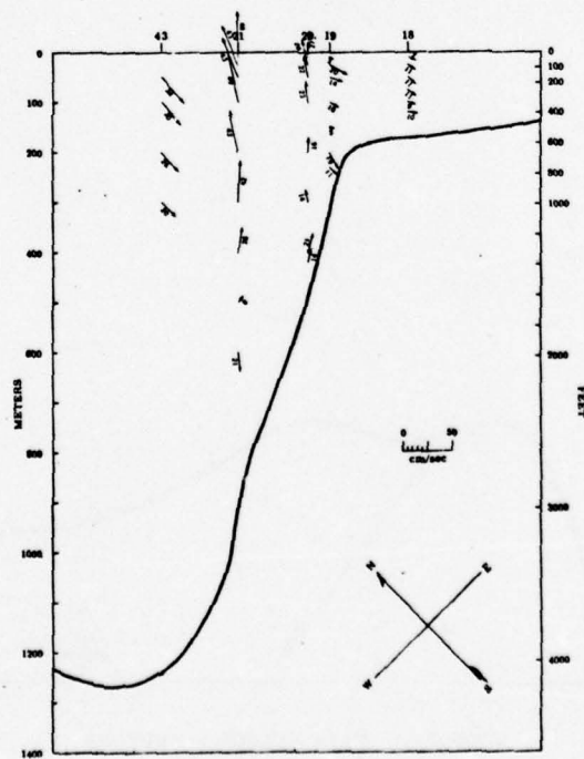
FIGURE 9 VECTIORIAL MEAN VELOCITY VECTORS CROSS-SECTION B
