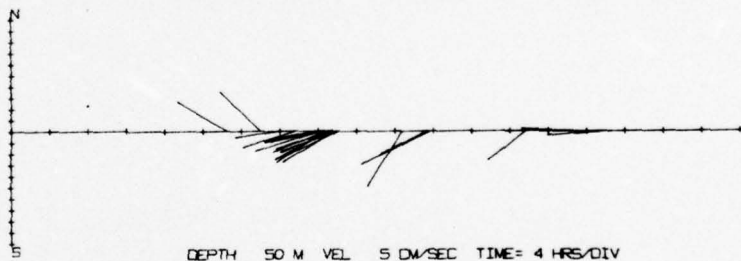
DEPTH 50 M VEL 5 CM/SEC TIME = 4 HRS/DIV
