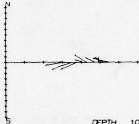
DEPTH 10 M VEL 5 CM/SEC TIME = 4 HRS/DIV
