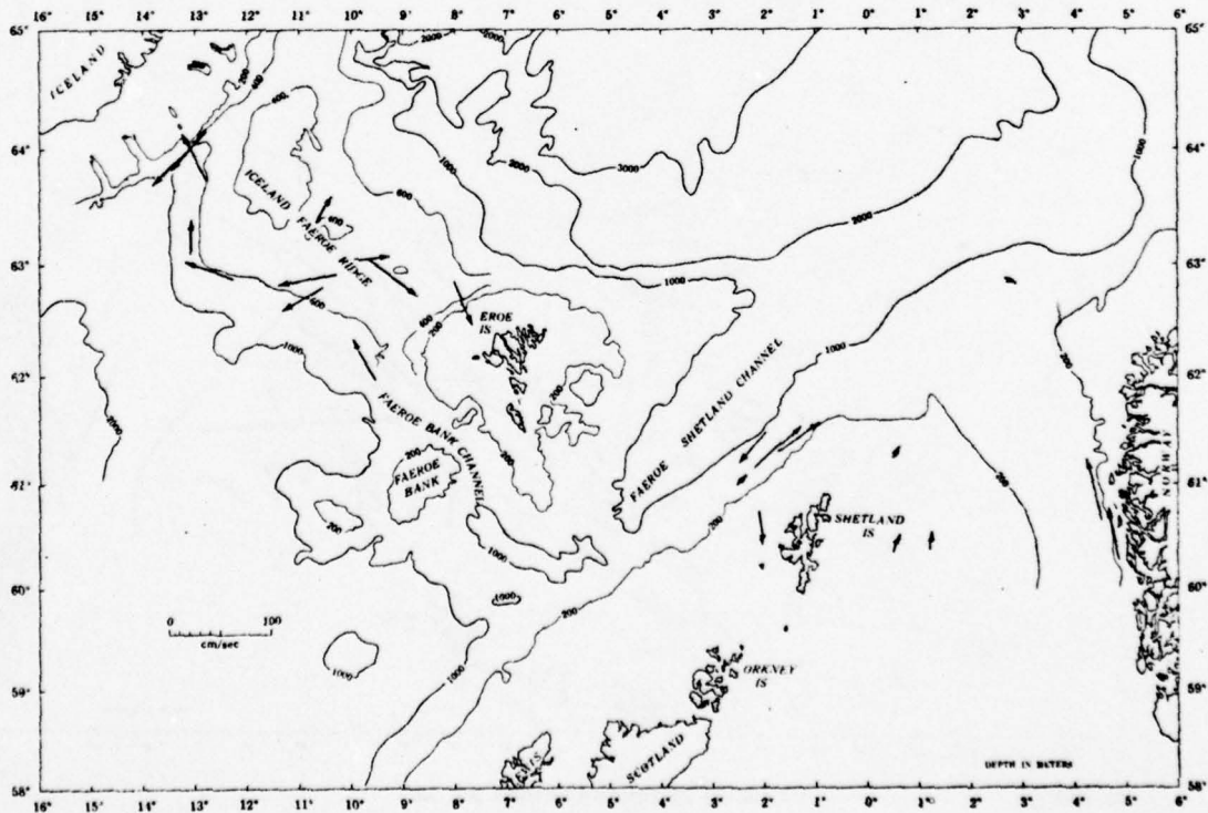
FIGURE 7 NEAR BOTTOM MAXIMUM VELOCITY VECTORS
