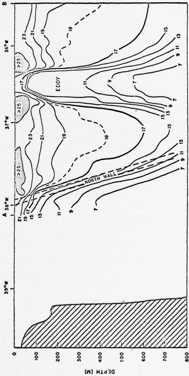
FIGURE 2. BATHY THERMOGRAPH SECTION (°C) 7-8 JUNE 1970
