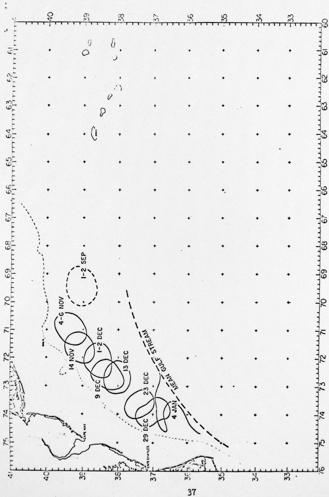
FIGURE 14. MOVEMENT AND RECAPTURE OF A-70-1 | SEPTEMBER 1970 - 4 JANUARY 1971 (15°C AT 200 M)
