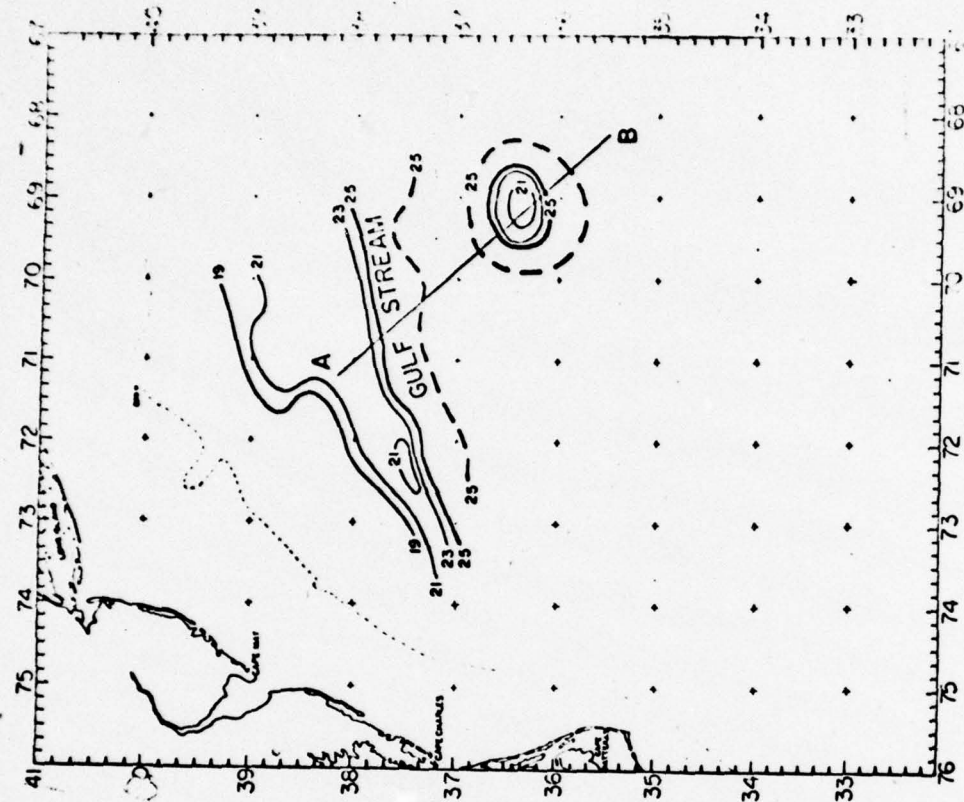
FIGURE 1d. SEA SURFACE TEMPERATURE ANALYSIS (°C) 8 JUNE 1970
