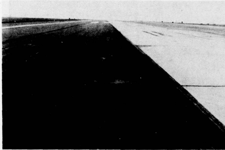
Figure 42. Medium Severity Longitudinal Crack.
