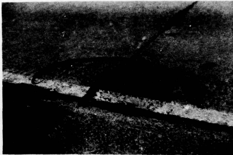
Figure 107. Pumping. (Note Fine Material on Surface That Has Been Pumped Out, Causing Corner Break.)
