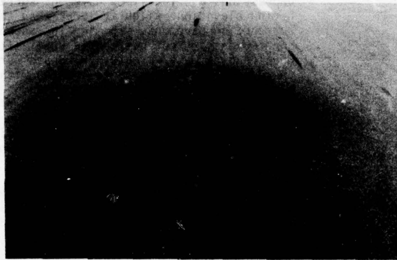
Figure 25. Low Severity Depression.
