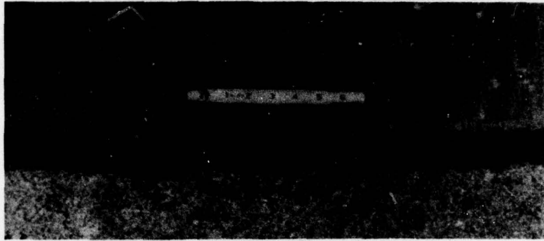
Figure 128. Low Severity Joint Spall.
