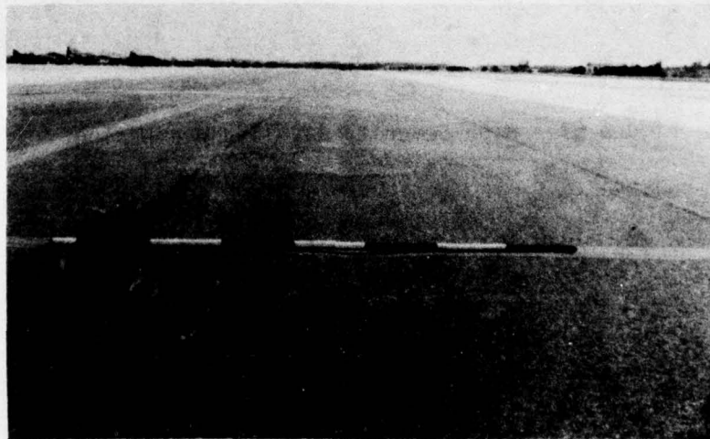
Figure 58. Light Severity Rutting.
