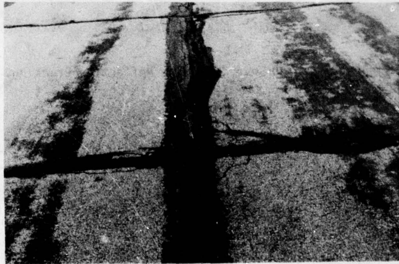
Figure 36. Medium Severity Joint Reflection Cracking.
