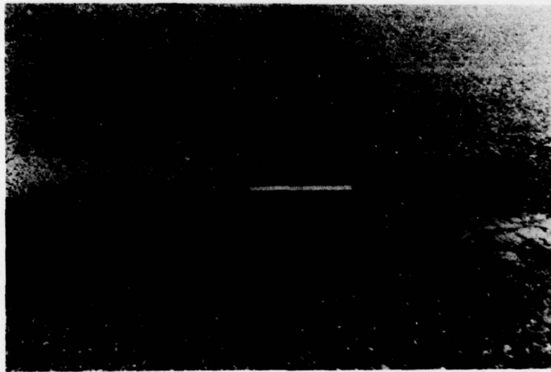
Figure 43. High Severity Longitudinal Crack.
