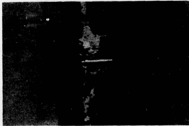
Figure 131. Medium Severity Joint Spall.
