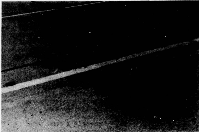
Figure 126. Shrinkage Cracks.
