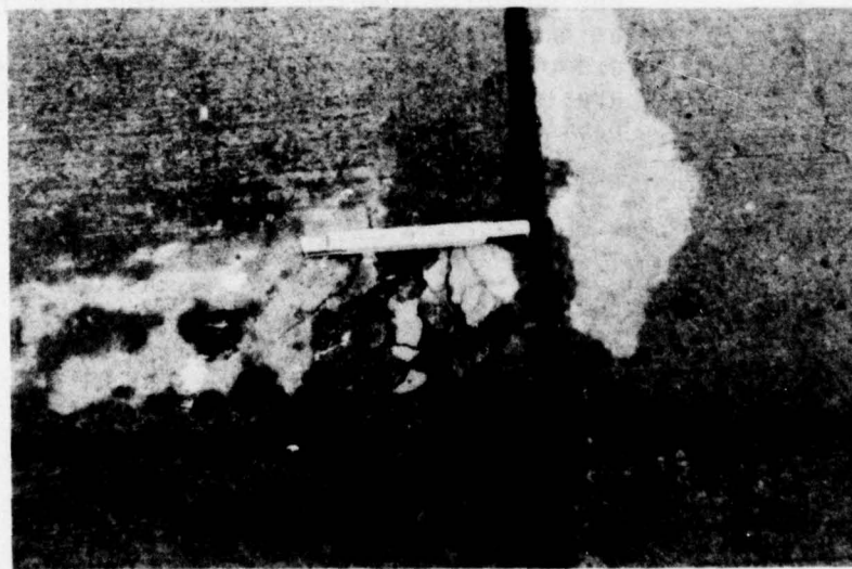
Figure 89. Medium Severity "D" Cracking.
