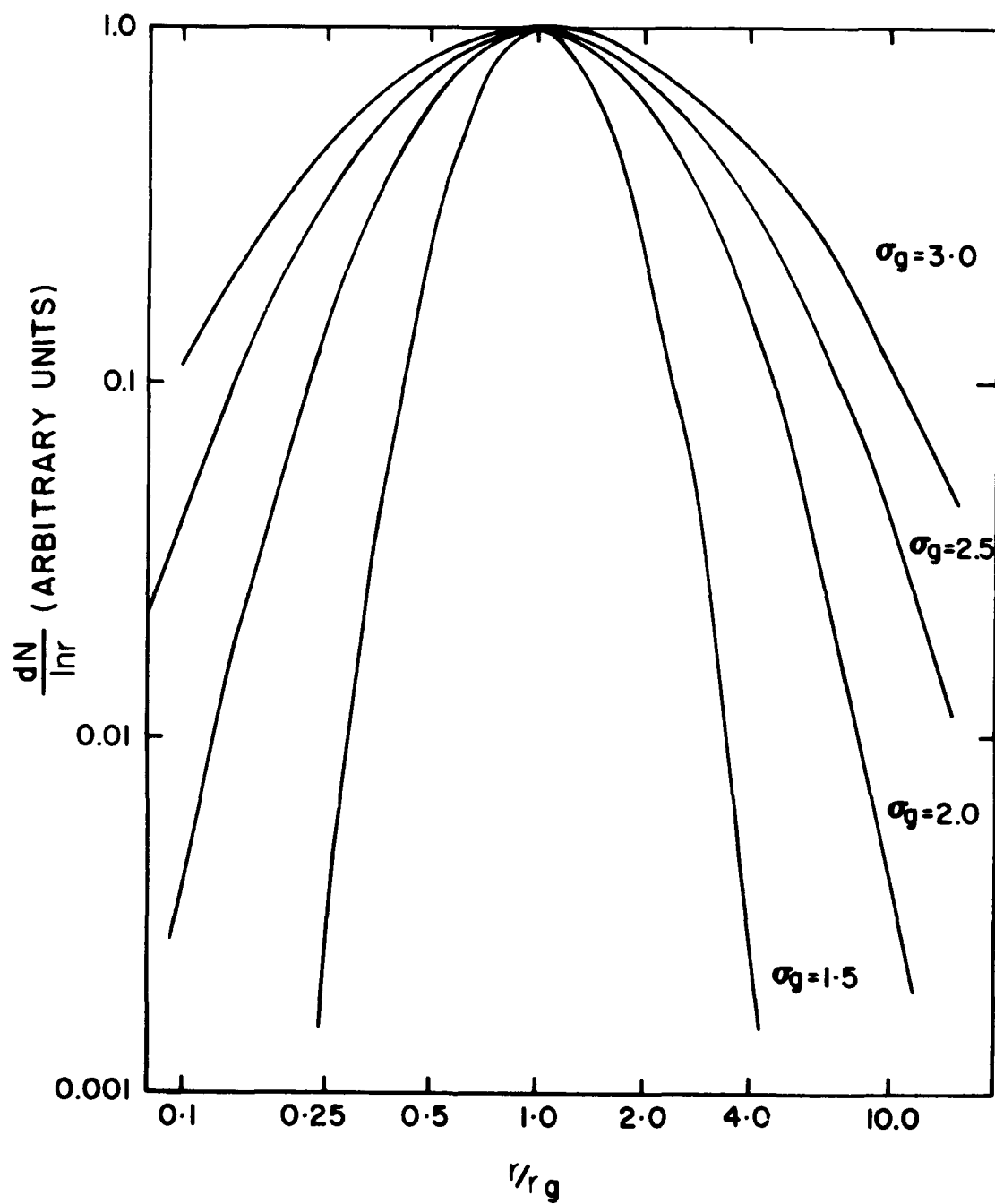
Figure 1. The lognormal distribution.
