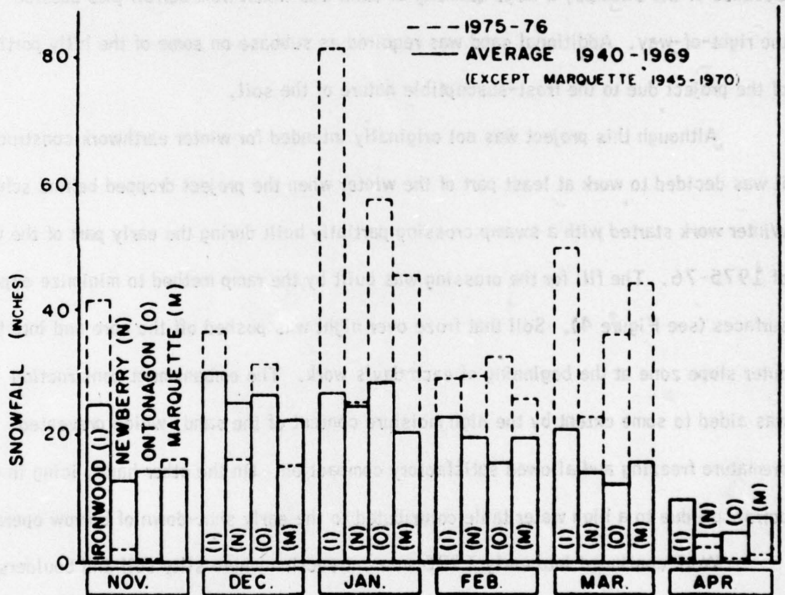
Figure 3 - Top - Average January Snowfall in Michigan's Upper Peninsula, inches, 1940-1969 Bottom - Monthly Snowfall at Four Stations
