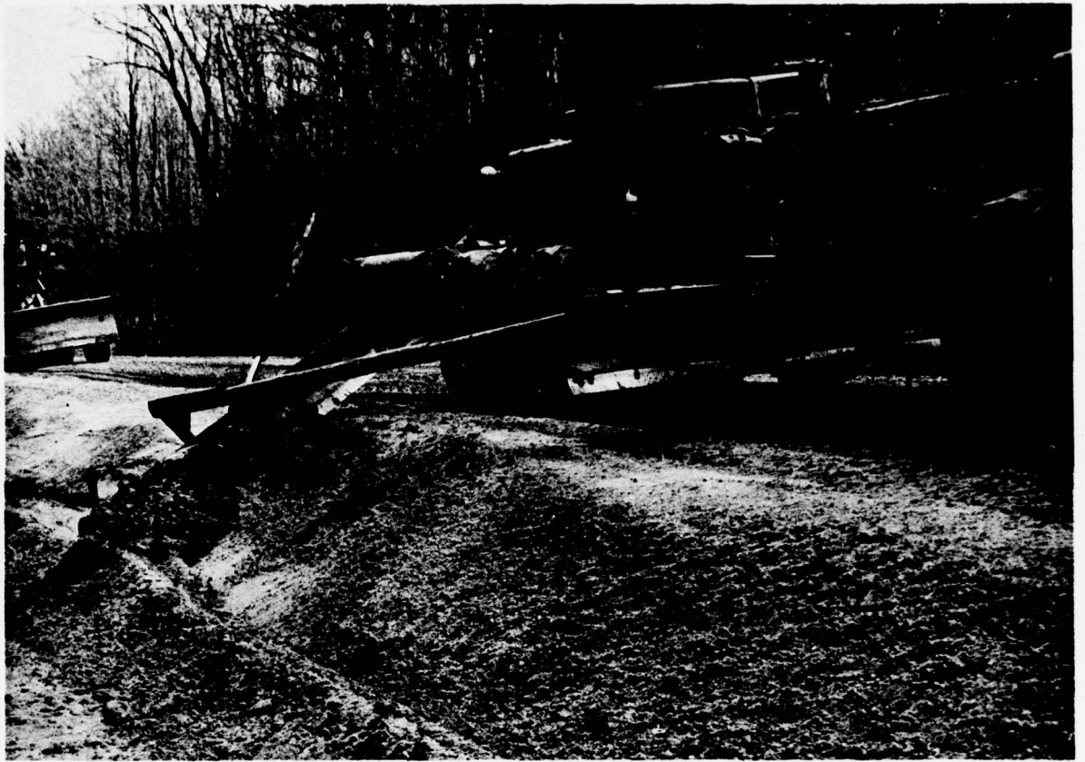
10. Ontonagon County. North Firesteel Road. Trimming and shaping of fill slopes after thawing is essentially complete. Grader with outrigger blade is leader in two-grader slope finishing team.
