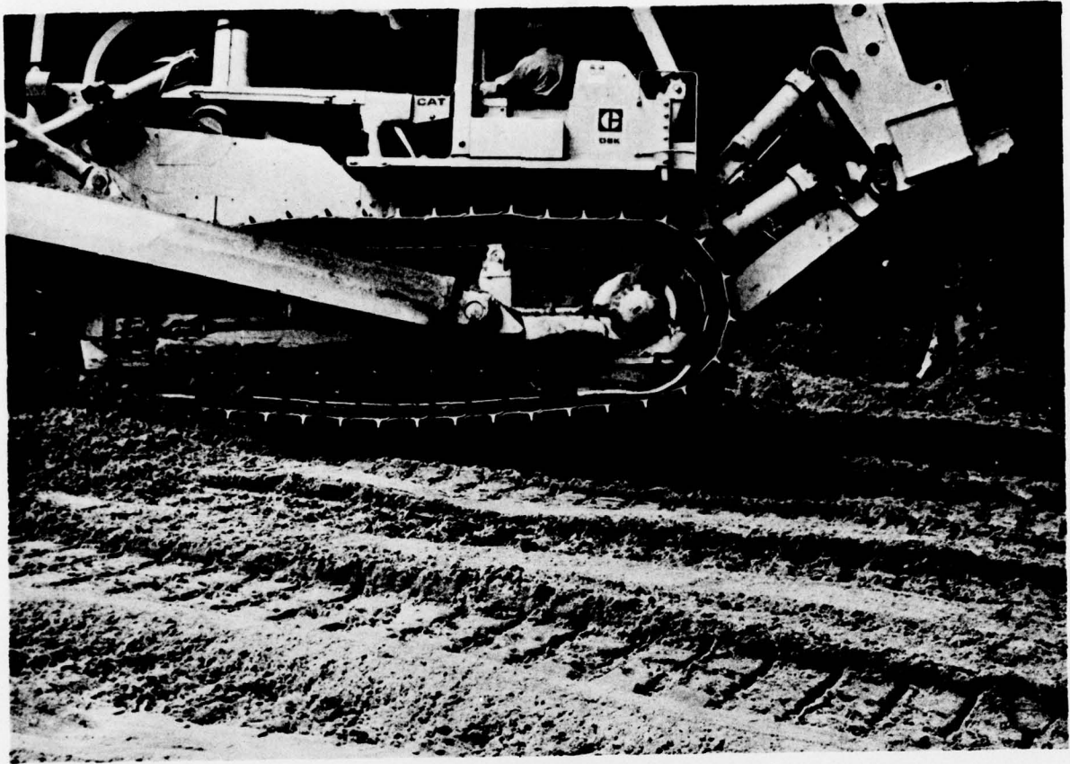
32. Marquette County. County Road 553. Bulldozer backfilling trench (see Photos 29, 30 and 31) and recompacting slope zone after all frozen soil had melted. Photo also shows ripper which was used to rip frozen soil for excavation by scrapers during previous winter.
