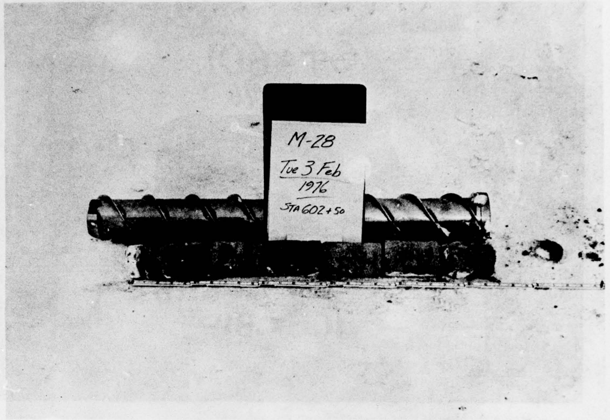
22. Alger County. State Road 28. Core of frozen sand taken from embankment constructed earlier in the winter. Top of core (left end in photo) includes hard packed snow resulting from construction traffic and snow clearing operations. Photo also shows core barrel used with powered drive unit for coring.
