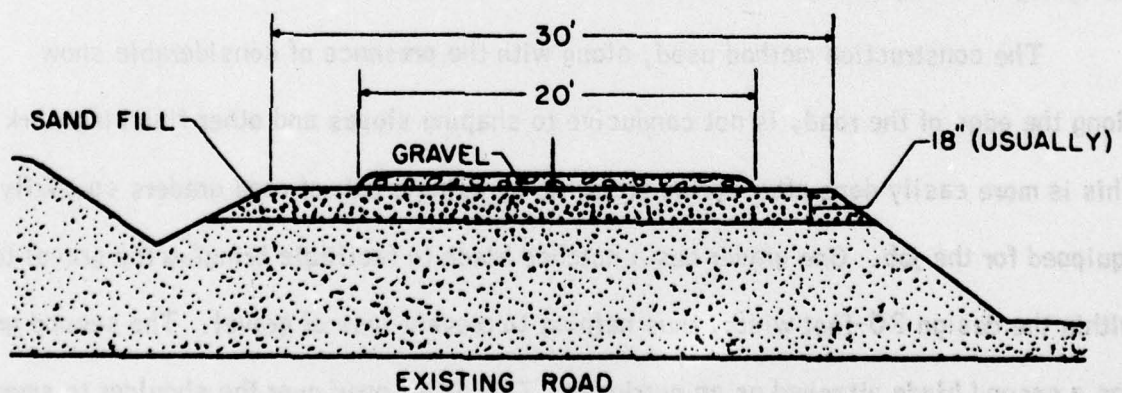
Figure 7 - Typical Section for Winter Fill Construction in Ontonagon County, Michigan 15
