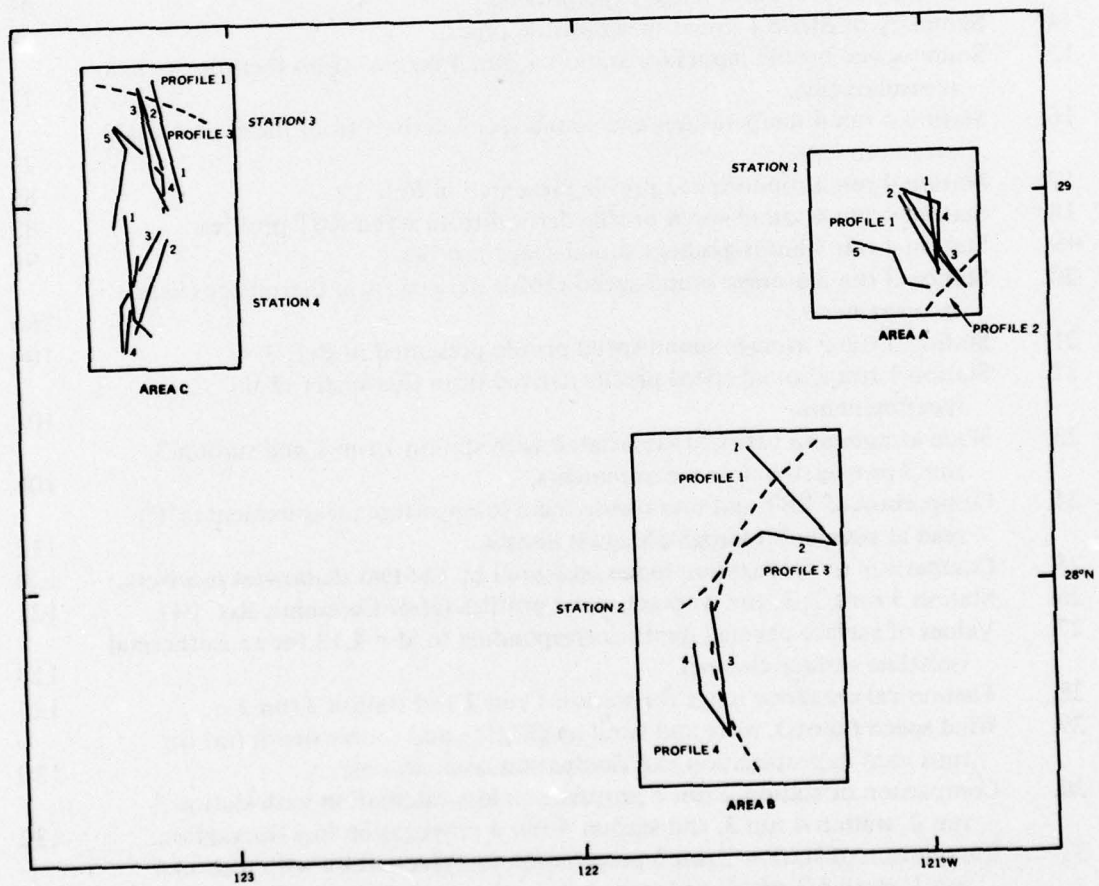
Figure 1. Location of experiments and sound-speed profile boundaries.
