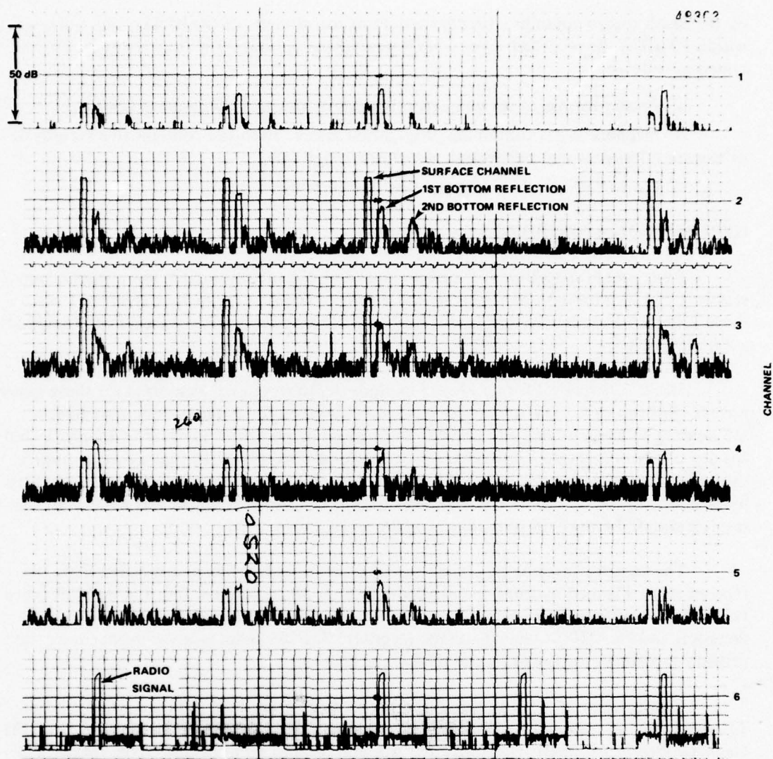
Figure 17. Sample Brush recorder record.
