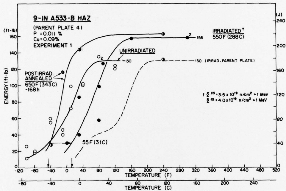
Fig. A9 - Notch ductility of HAZ 4 (Series 2) before and after irradiation to a low fluence. The notch ductility of the parent plate (WR orientation, Fig. A8) after irradiation is also indicated.
