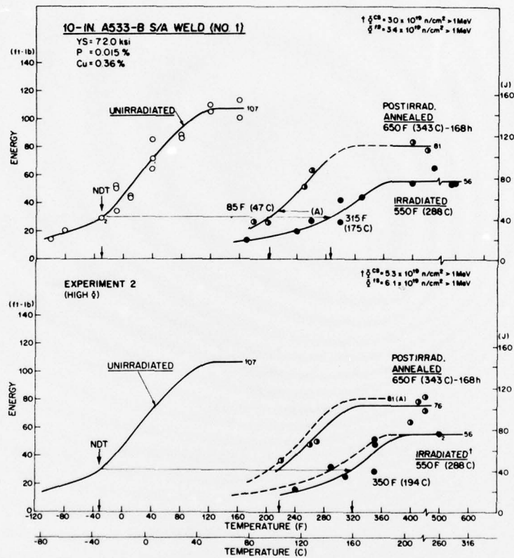
Fig. A4 - Notch ductility of weld 1 (Series 1) before and after irradiation.
