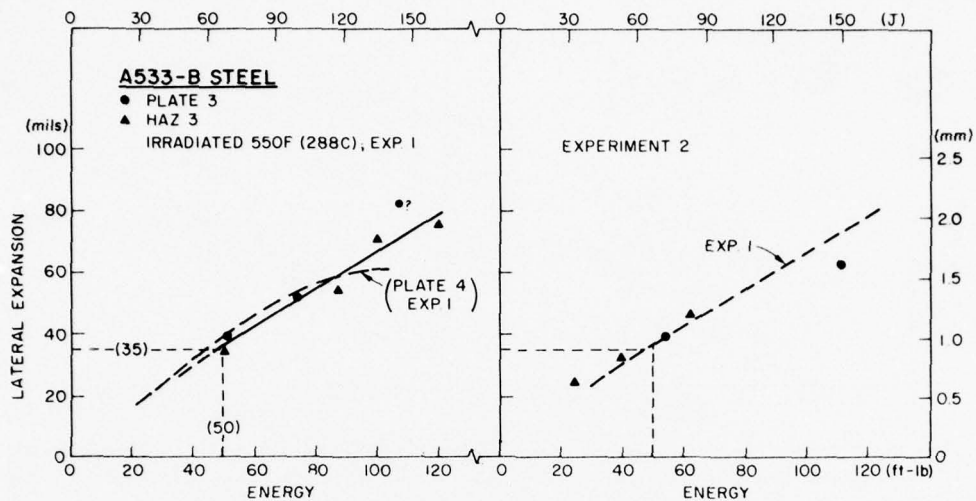
Fig. 10 - Charpy-V lateral expansion vs energy absorption trends observed for plate 3 and HAZ 3 (Series 2) after irradiation. In the left-hand graph the dashed curve reproduces the trend for plate 4 (Experiment 1) from Fig. 11.
