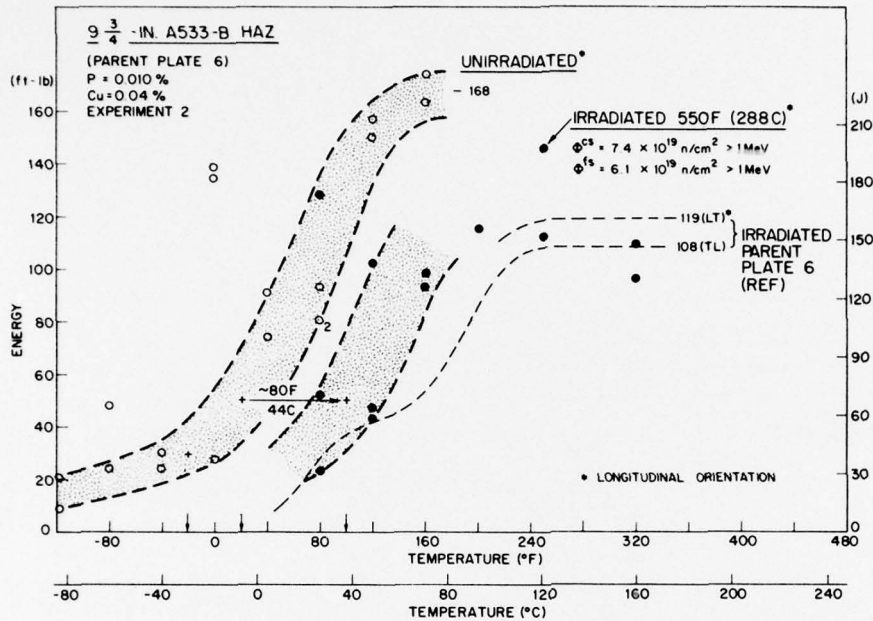
Fig. 5 - Notch ductility of HAZ 6 before and after irradiation. The notch ductility of the parent plate (LT and TL orientations, Fig. 4) after irradiation is also indicated.
