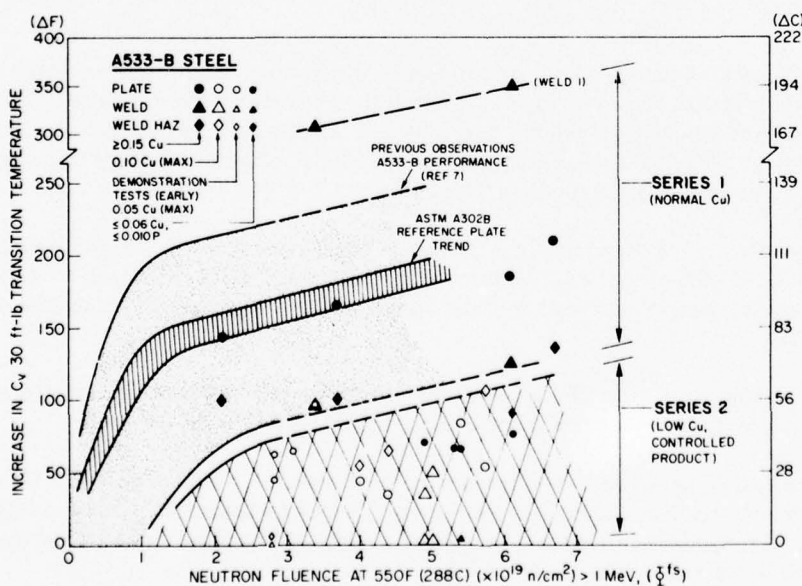
Fig. 14 - Summary of Charpy-V transition temperature observations for Series 3 materials (small filled symbols) superimposed on graph of Fig. 1. An entry (datum) for HAZ 5 was precluded by high data scatter. The results demonstrate comparable radiation resistance in materials with 0.06%Cu max and 0.10%Cu max contents, respectively representing best steelmaking practice vs current improved practice.
