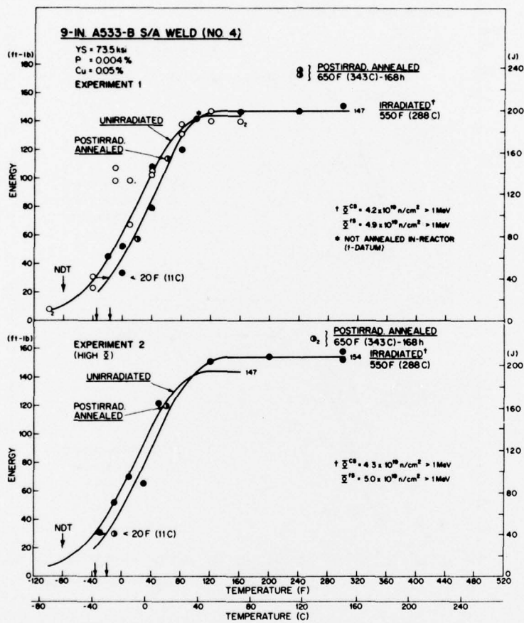
Fig. A11 - Notch ductility of weld 4 (Series 2) before and after irradiation. The low-fluence exposure included a midcycle 800°F (427°C) 5-1/2-hr anneal except for one specimen tested at 100°F (38°C).
