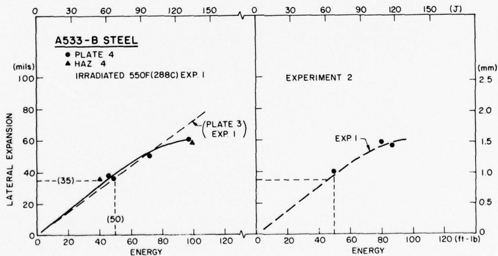
Fig. 11 - Charpy-V lateral expansion vs energy absorption trends observed for plate 4 and HAZ 4 (Series 2) after irradiation. The trend for plate 3 (Experiment 1) from Fig. 10 is also shown in the left-hand graph.
