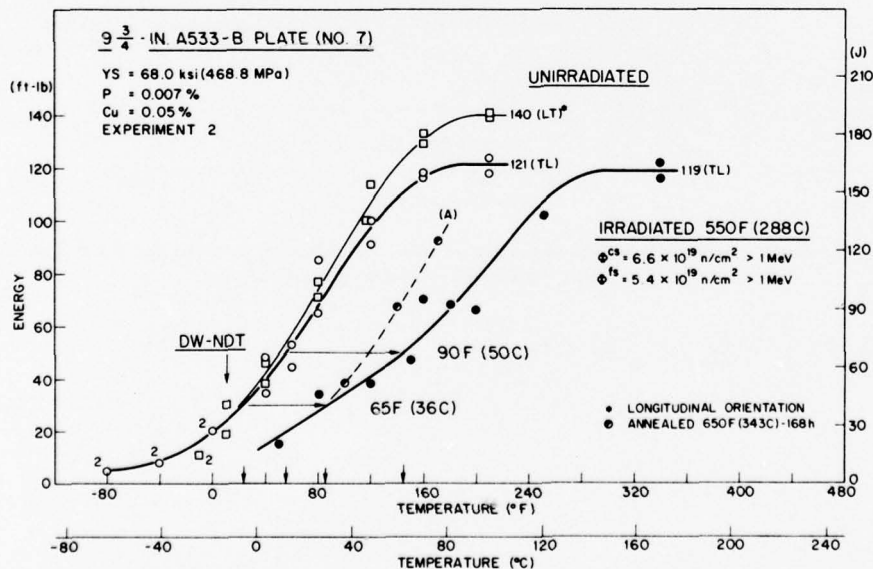
Fig. 6 - Notch ductility of plate 7 before and after irradiation. Limited data for the postirradiation annealed condition are also shown.
