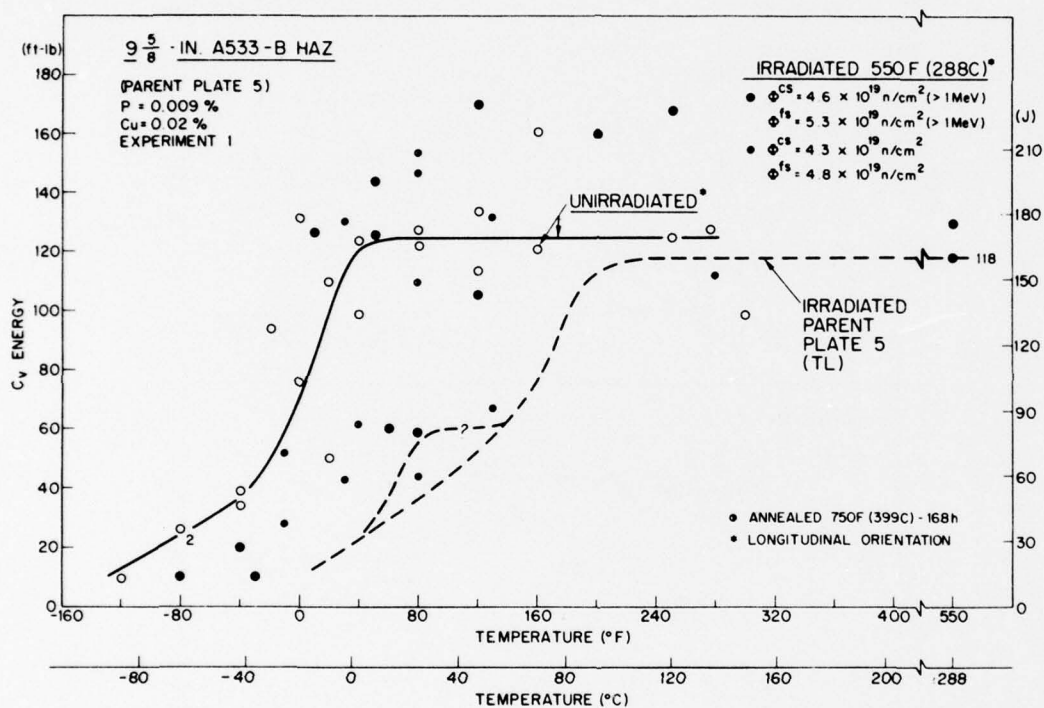
Fig. 3 - Notch ductility of HAZ 5 before and after irradiation. The notch ductility of the parent plate (TL orientation, Fig. 2) after irradiation is also indicated (dashed curve).
