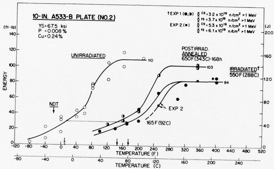
Fig. A3 - Notch ductility of plate 2 (Series 1) before and after irradiation to a low fluence. Limited data from a high-fluence experiment (small filled symbols) are also shown.
