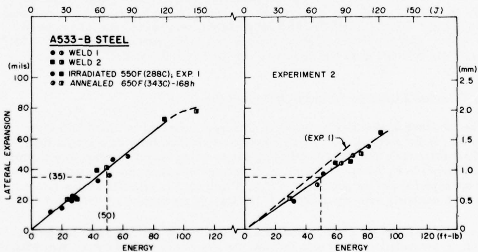
Fig. 9 - Charpy-V lateral expansion vs energy absorption trends observed for weld 1 and weld 2 (Series 1) after irradiation and after postirradiation heat treatment.
