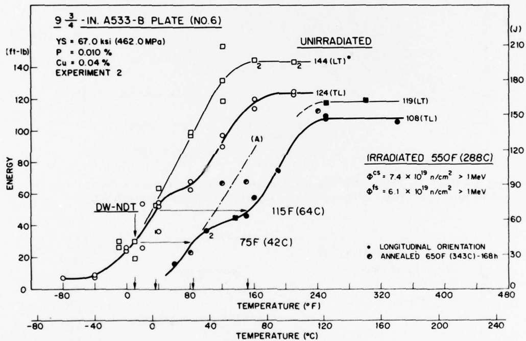
Fig. 4 - Notch ductility of plate 6 before and after irradiation. Limited data for the postirradiation annealed condition (half-filled symbols) are also shown.
