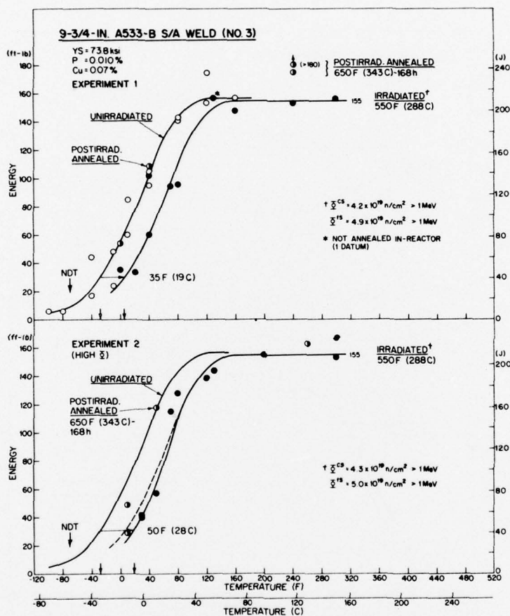
Fig. A10 - Notch ductility of weld 3 (Series 2) before and after irradiation. In this case, the low-fluence exposure included a midcycle 800°F (427°C) 5-1/2-hr anneal except for one specimen tested at 120°F (49°C).
