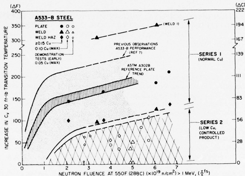
Fig. 1 - Summary of Charpy-V 40-J (30 ft-lb) transition-temperature changes with irradiation observed for Series 1 materials (large filled symbols) and Series 2 materials (large open symbols). A benefit to radiation-embrittlement resistance by a low copper content is clearly evident. Earlier determinations for extra-low copper content A533-B materials from commercial-scale demonstration tests are also given (small open symbols) [4].
