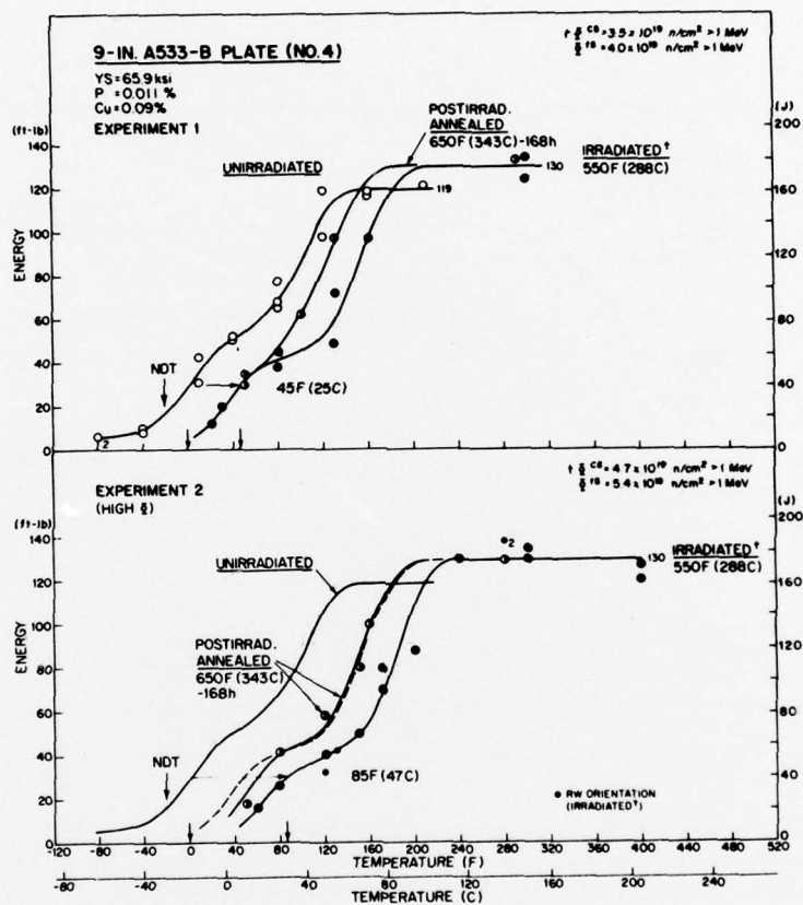
Fig. A8 - Notch ductility of plate 4 (Series 2) before and after irradiation.
