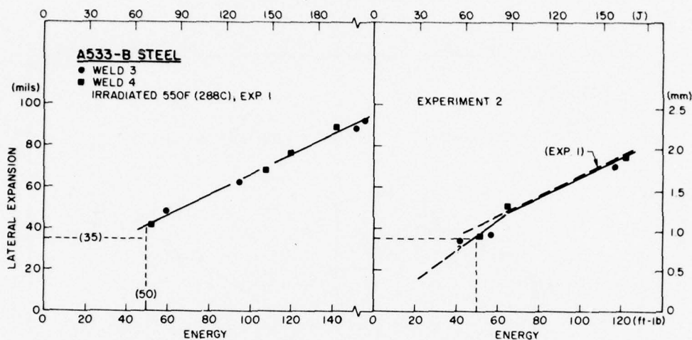
Fig. 12 - Charpy-V lateral expansion vs energy absorption trends observed for weld 3 and weld 4 after irradiation. Note the apparent inflection in the trend curve at approximately 88 J (65 ft-lb).
