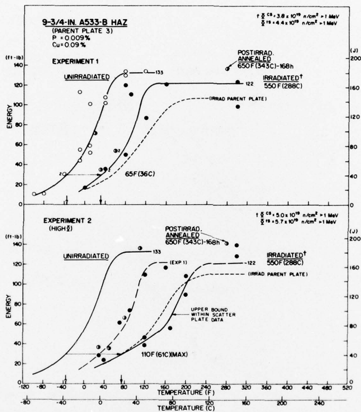
Fig. A7 - Notch ductility of HAZ 3 (Series 2) before and after irradiation. The notch ductility of the parent plate (WR orientation, Fig. A6) after irradiation is also indicated.
