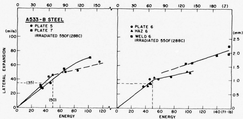
Fig. 13 - Charpy-V lateral expansion vs energy absorption trends observed for plate 5 and plate 7 (left-hand graph) and plate 6, HAZ 6, and weld 6 (right-hand graph) from Series 3 after irradiation. Note the inflection in the trend curves in the range of 68 to 82 J (50 to 60 ft-lb).
