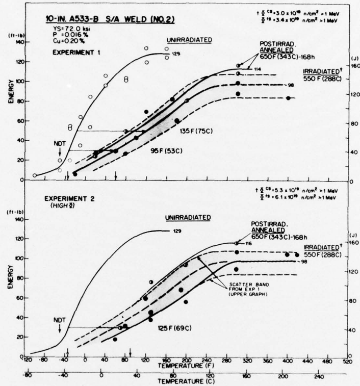
Fig. A5 - Notch ductility of weld 2 (Series 1) before and after irradiation.
