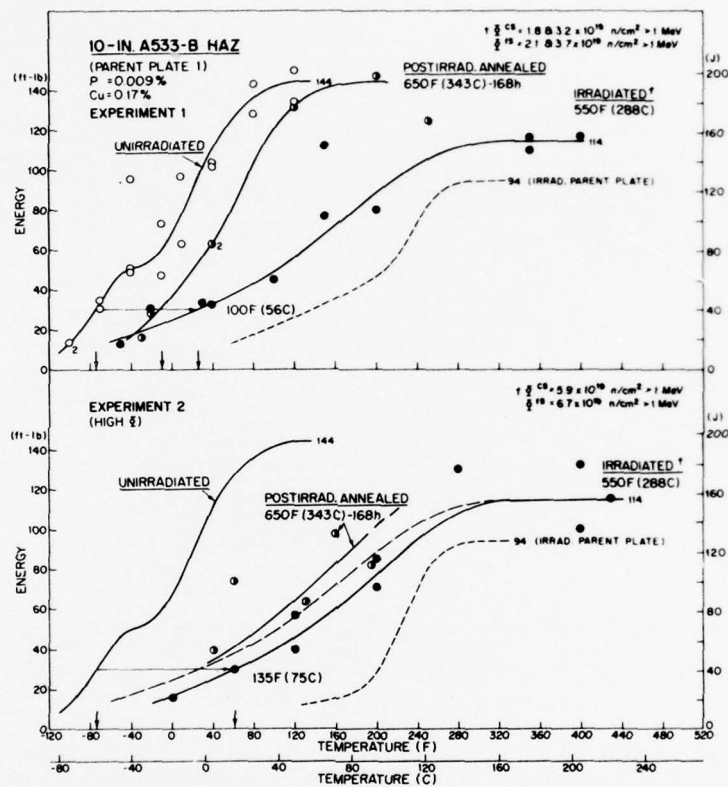
Fig. A2 - Notch ductility of HAZ 1 (Series 1) before and after irradiation. The notch ductility of the parent plate (WR orientation, Fig. A1) after irradiation is also indicated.
