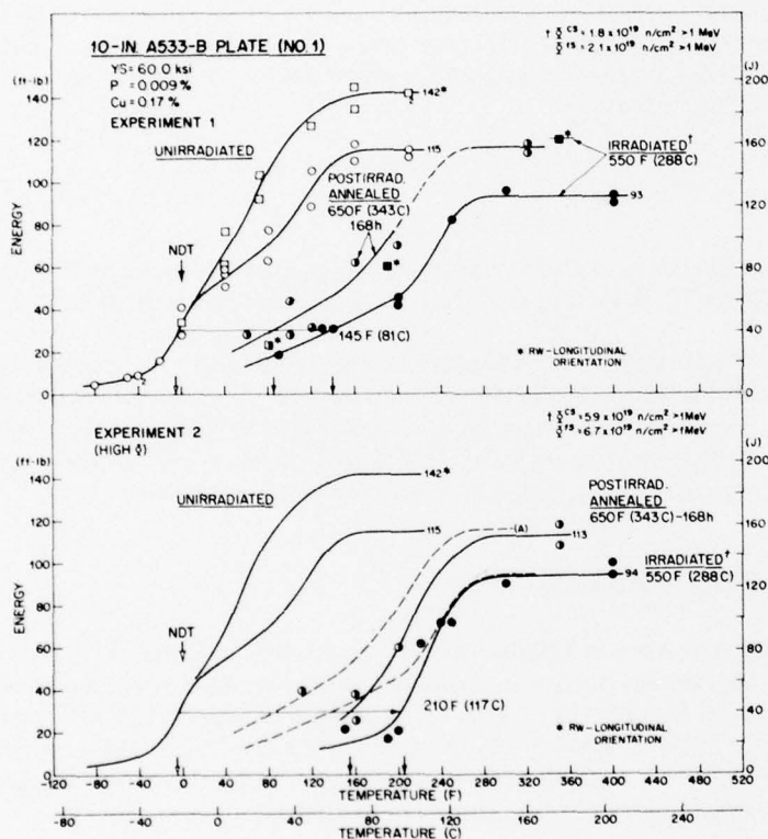
Fig. A1 - Notch ductility of plate 1 (Series 1) before and after 550°F (288°C) irradiation. In this figure and in Figs. A2 through A11, open and filled symbols refer to unirradiated and irradiated conditions respectively; half-filled symbols refer to the 650°F (343°C) postirradiation annealed condition. Also by convention results for the low-fluence and the high-fluence experiments are given in top and bottom graphs respectively. In some figures, curves for the irradiated and postirradiation annealed (A) condition in the top graph are repeated as dashed curves in the bottom graph for quick comparisons.
