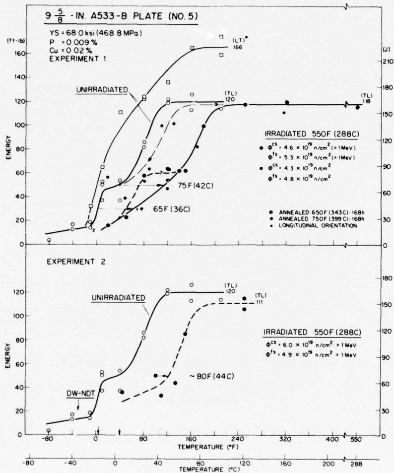
Fig. 2 - Notch ductility of plate 5 (Series 3) before and after 288°C (550°F) irradiation to two fluence levels. In this figure and in Figs. 3 through 7 open and filled symbols refer to unirradiated and irradiated conditions respectively.
