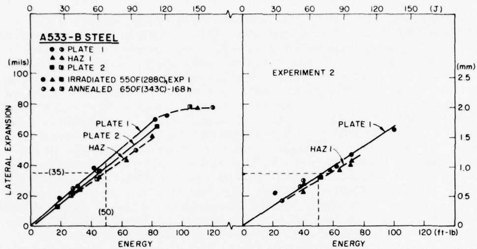
Fig. 8 - Charpy-V lateral expansion vs energy absorption trends observed for plate 1, HAZ 1, and plate 2 (Series 1) after irradiation and after postirradiation heat treatment. In this figure and in Figs. 9 through 12 "Experiment 2" refers to the high fluence condition.
