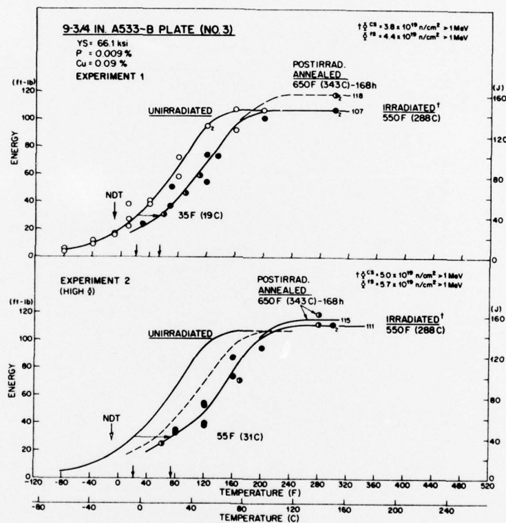
Fig. A6 - Notch ductility of plate 3 (Series 2) before and after irradiation. Note the anomalous increase in C_v upper shelf energy with postirradiation annealing.
