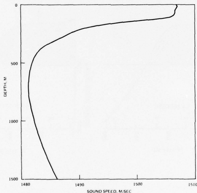
Figure 2. Station 4, run 1. Average sound-speed profile.
