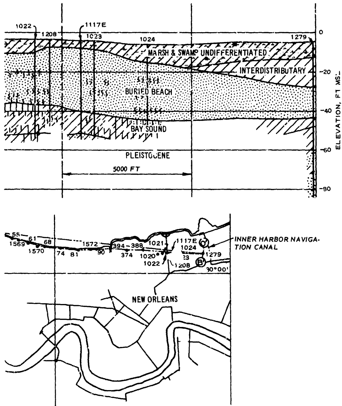
Figure 33. Geologic section (map inset) near Inner Harbor Navigation Canal, New Orleans, showing marsh and swamp deposits and interdistributary clays overlying buried beach sands (from Reference 13)
