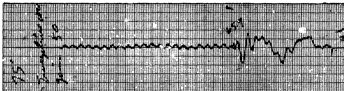
b. HAMMER STATION 75 FT FROM GEOPHONE, TRAVEL TIME = 65.9 MSEC
