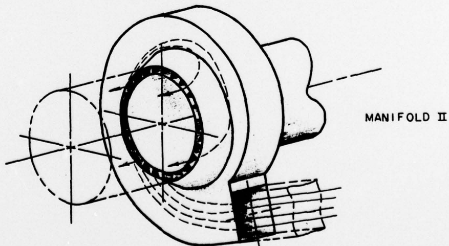
FIG. 2: MANIFOLD VARIATIONS
