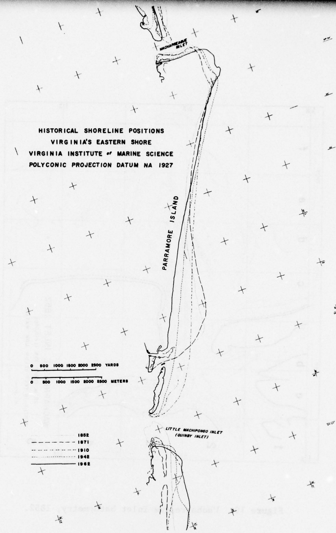
Figure 9. Historical shoreline positions (1852-1962) of Parramore Island.
