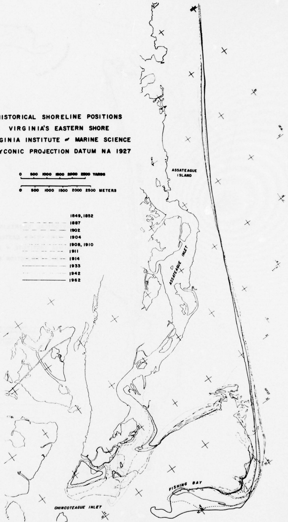
Figure 5. Historical shoreline positions (1852-1962) of lower Assateague Island.
