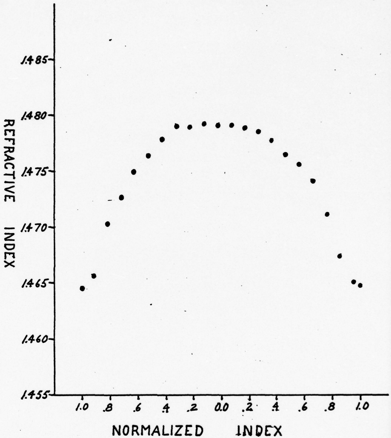
Fig. 9. The profile of a rod doped with Kawecki-Berylco \text{CsNO}_3 . The profile is moderately good in shape but the edges are too high. Rod 2892.
