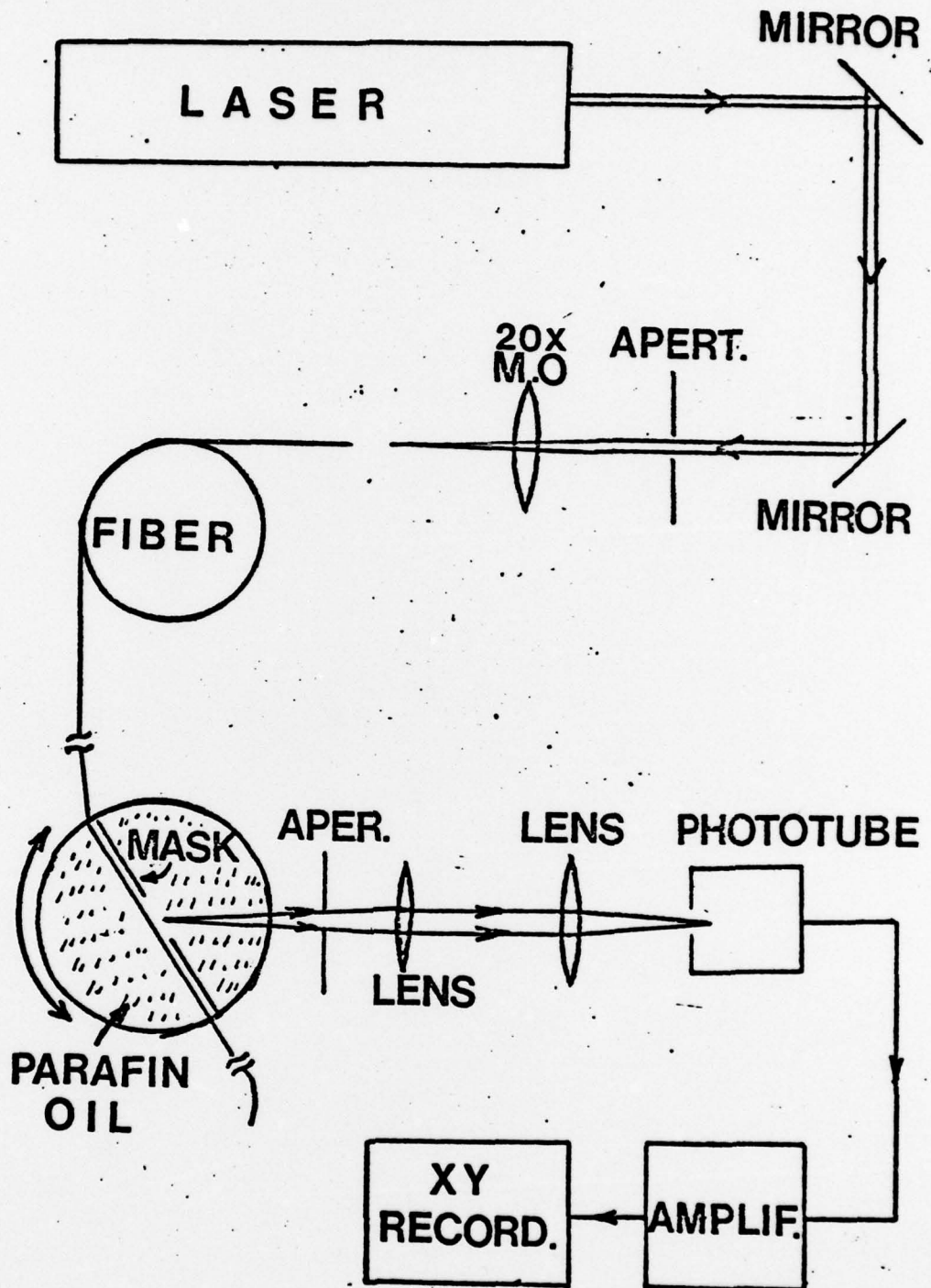
Figure 23. Schematic of the apparatus for measuring the angular distribution of scattered light.
