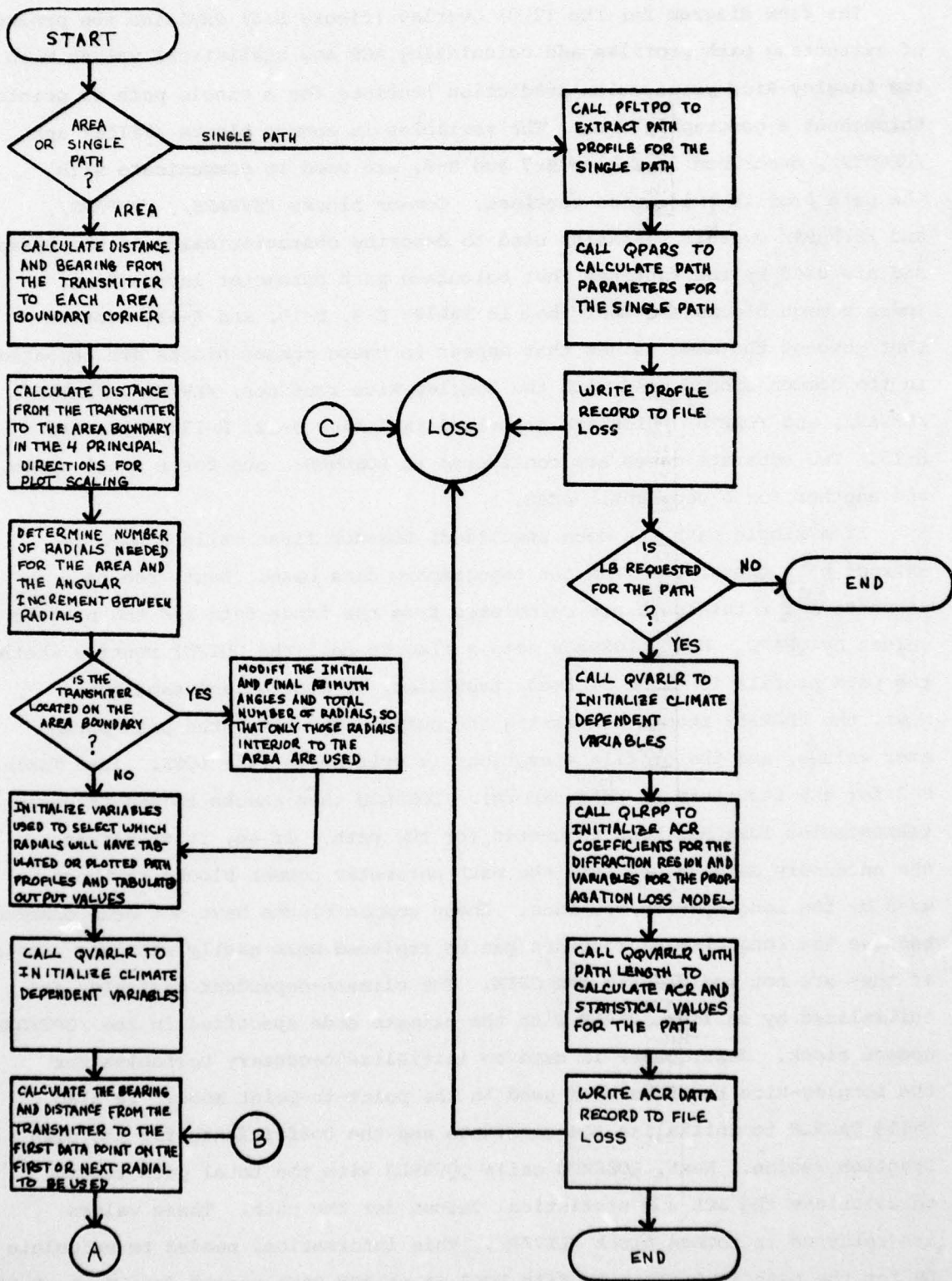
Figure B-4. Process diagram for overlay (2,0) - LOSSMOD.
