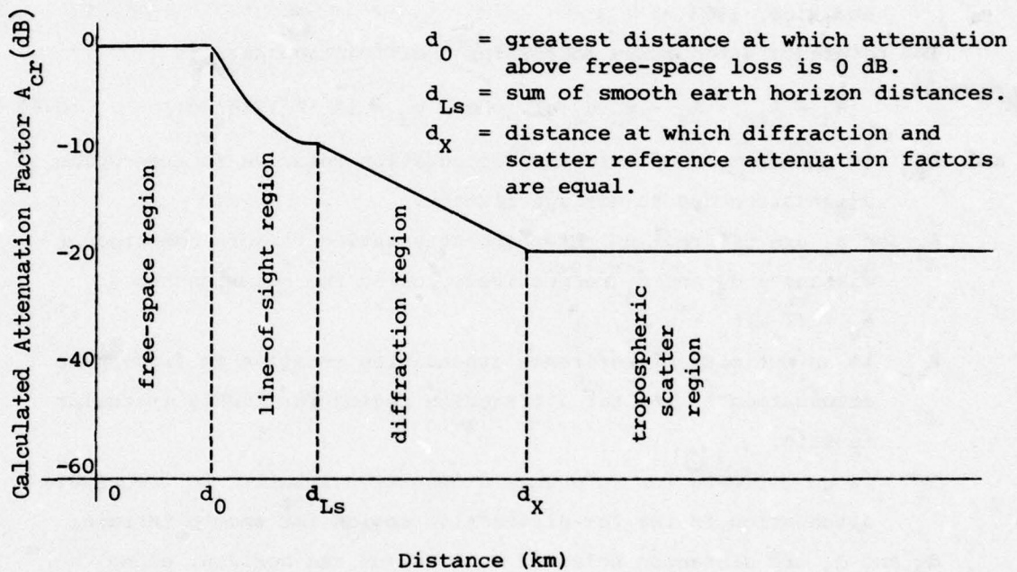
Figure C-1. Calculated attenuation factor A_{cr} versus path length for line-of-sight, diffraction, and tropospheric scatter regions.
