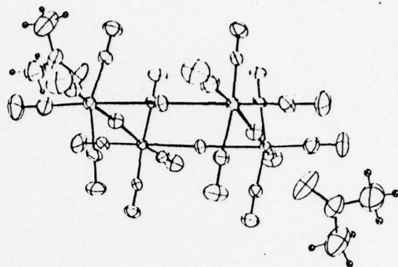
[\text{CdFe}(\text{CO})_4]_4
