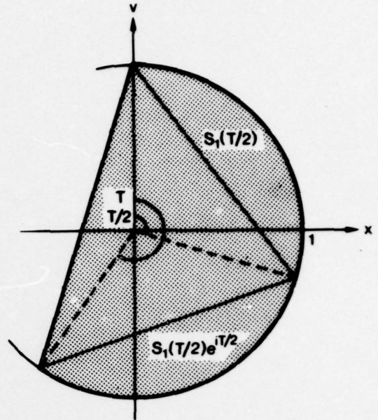
(b) \pi \leq T \leq 2\pi . Construction using S_1(T/2) and S_1(T/2)e^{iT/2}
