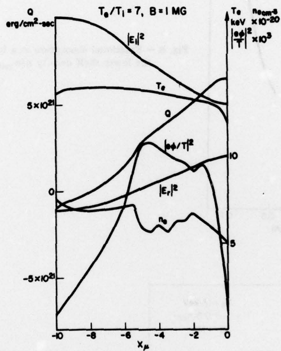
Fig. 8 — Typical solution for lower temperature ratio. Chopping behavior of n_e(x) and |\phi/T|^2(x) corresponds to shifting dominant unstable mode.
