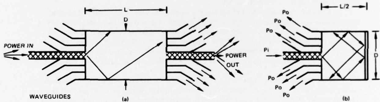
Figure 1. Coupler operation.
