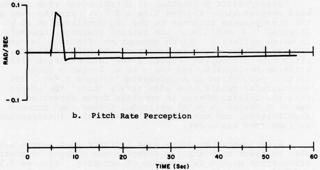
Figure 5.4 Model Response to .2rad Pitch Up Stimulus.
