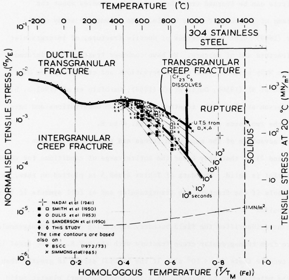
Fig. 4 A fracture map for type 304 stainless steel. It shows four mechanism fields. Contours of constant time-to-fracture ( t_f ) are shown. They are based on data from the sources listed on the figure.
