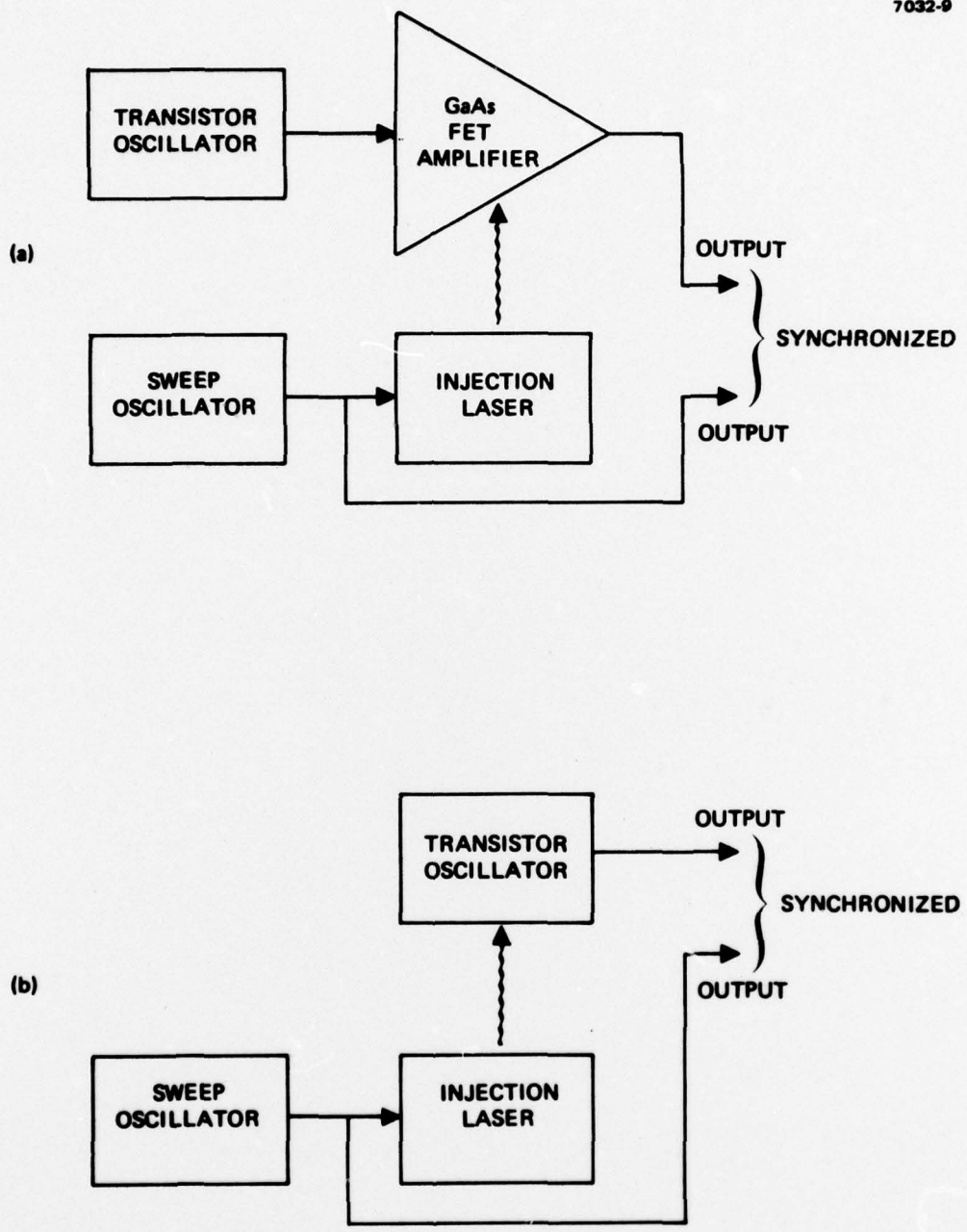
Figure 9. Schematics of two optical injection locking schemes.
