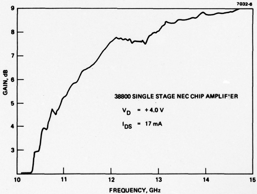
Figure 6. Gain versus frequency plot of a single-stage GaAs FET amplifier.
