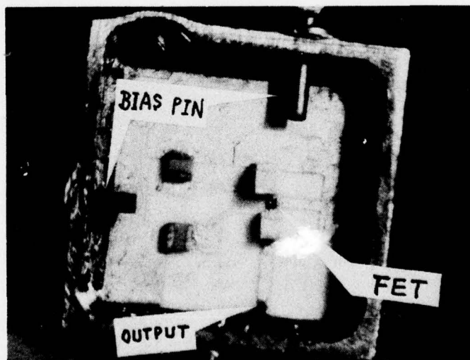
Figure 3. Photograph of the completed GaAs FET oscillator module.
