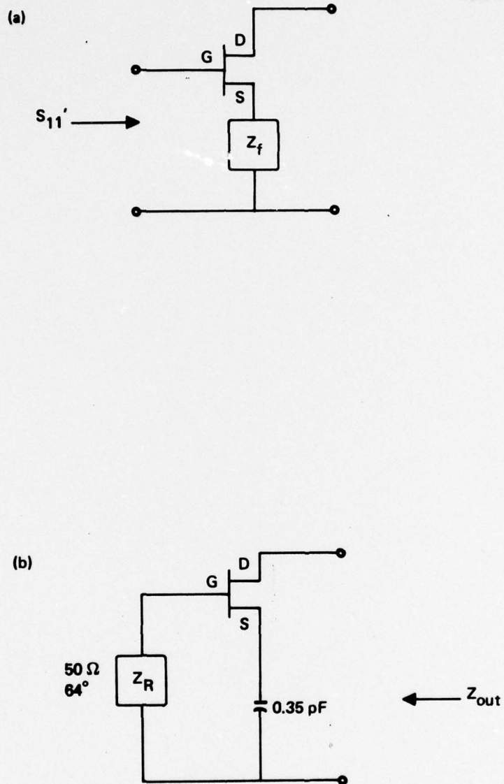
Figure 1. Design of a GaAs FET common source oscillator with series feedback element.
