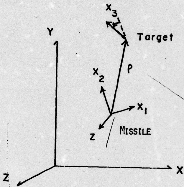
Fig. 1 Geometry for a Two-Dimensional Intercept System
