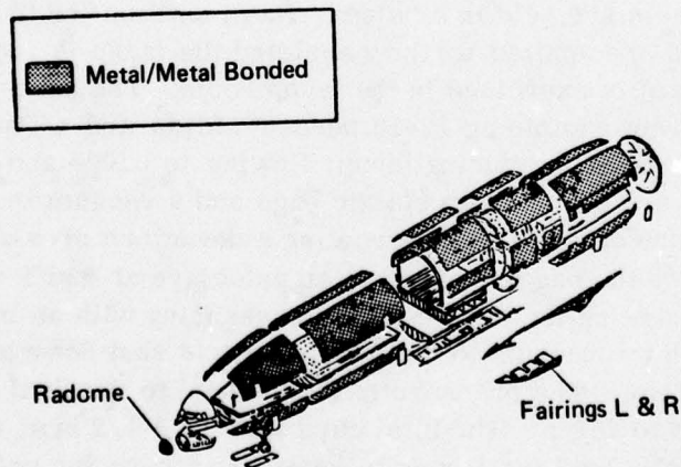
Figure 1. Structural Bonding-Fuselage
