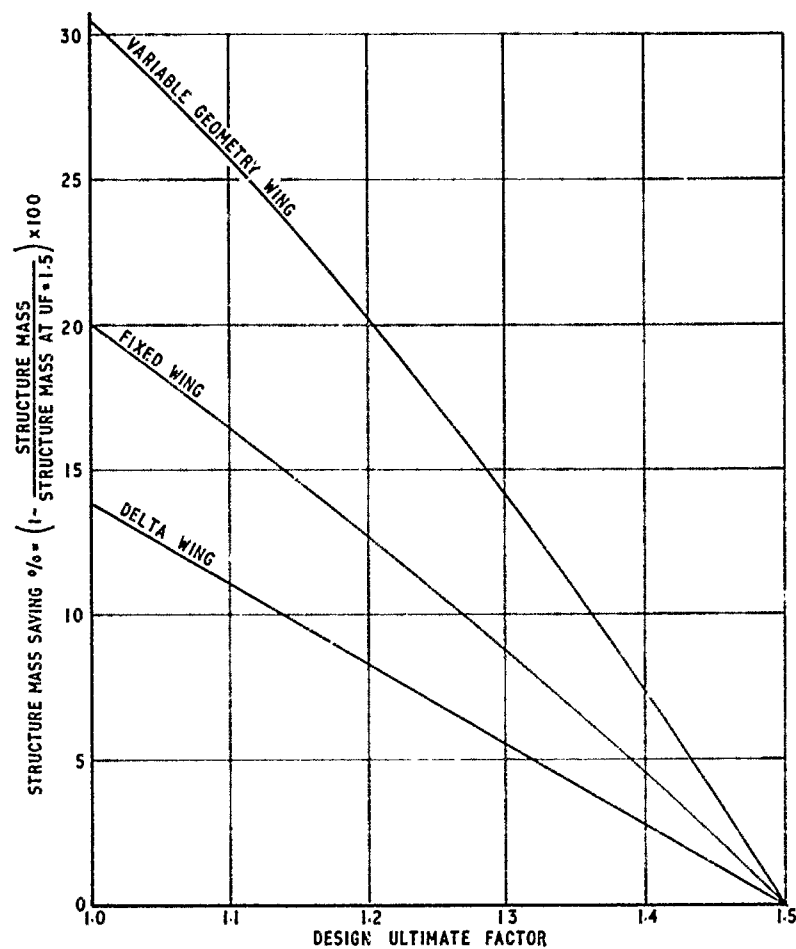
FIG.6 SAVINGS IN STRUCTURE MASS FOR VARIATIONS IN ULTIMATE FACTOR(FULLY RE-SIZED A/C)
