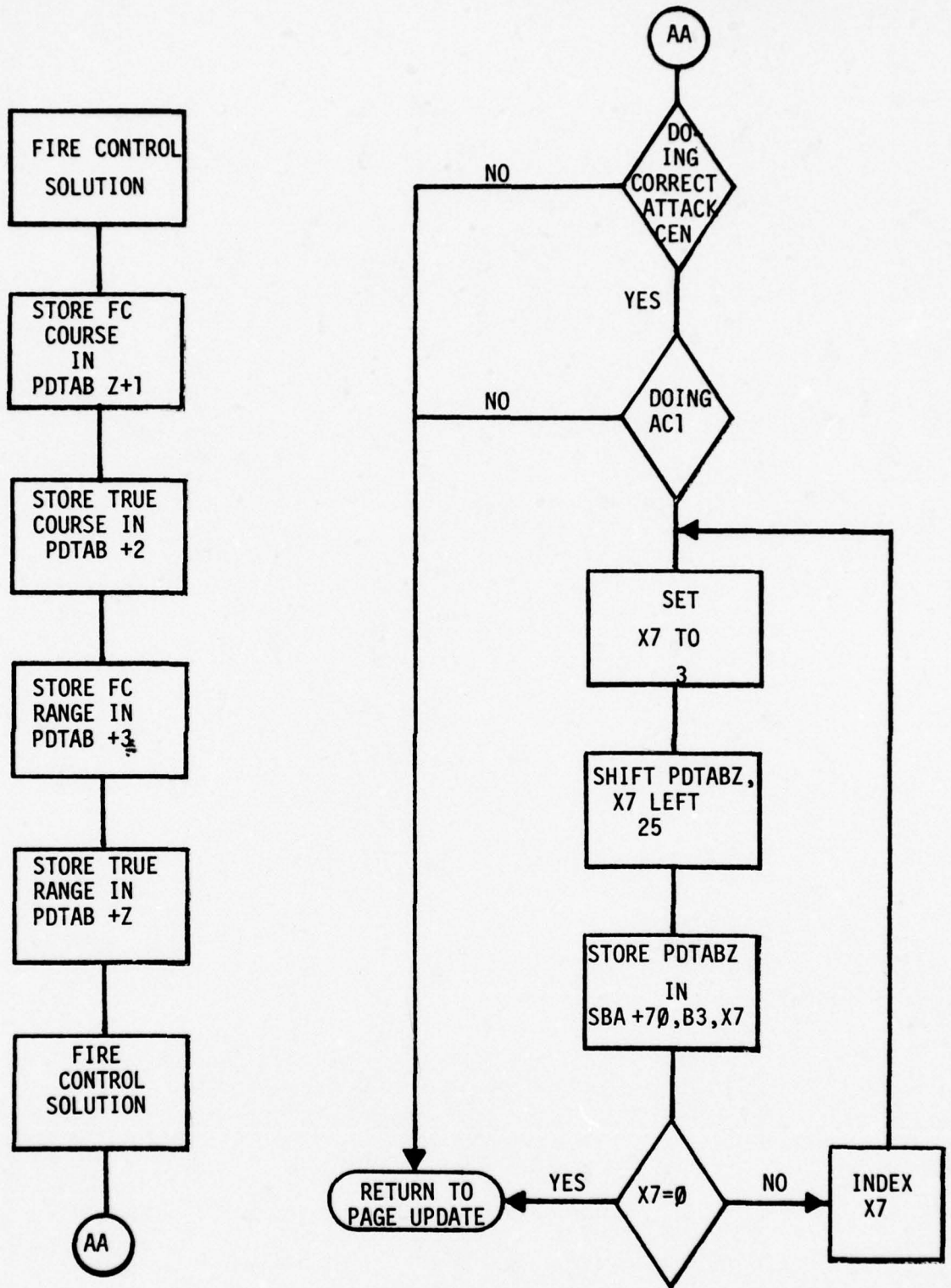
Figure C-3. Prob. det. data acquisition routine.
