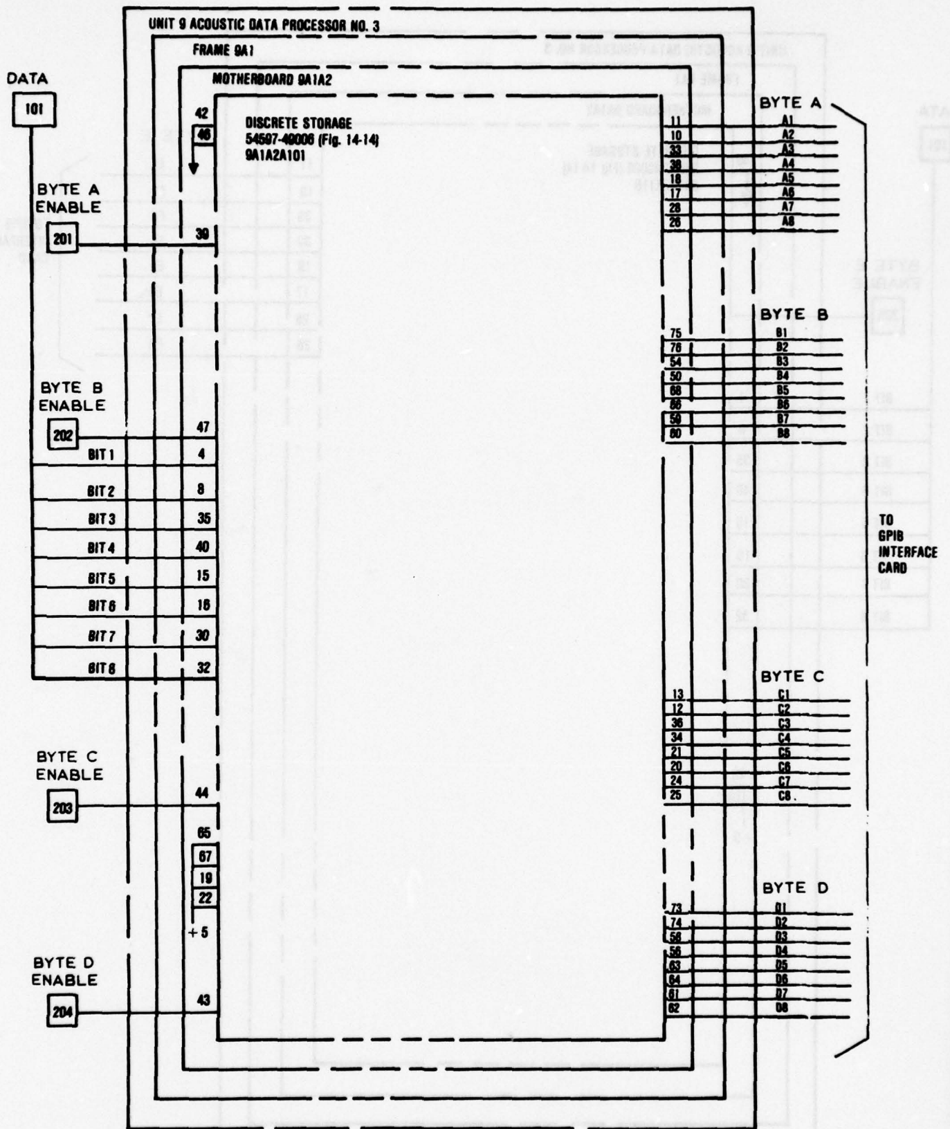
Figure B-4. First discrete storage card connections.
