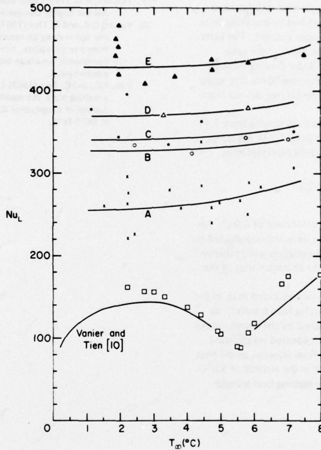
Figure 6. Comparison of present data with those from free convection studies.
