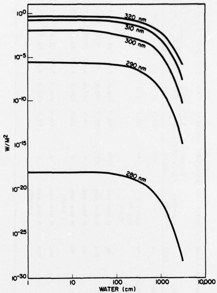
Fig. 1 — Penetration of UV-B into distilled water, calculated on the basis of incident light at 90° and the ozone concentration at 0.32 atm. cm.
