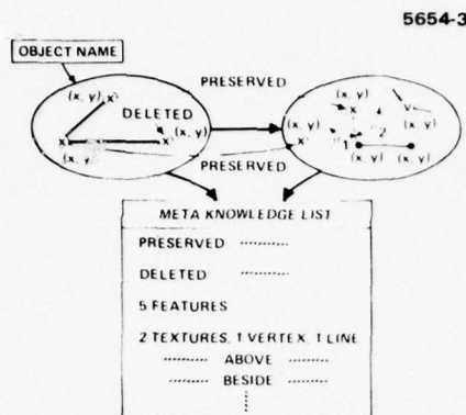
Figure 37. Data structure.
