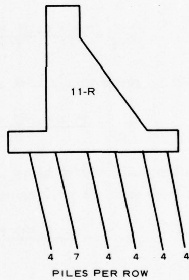
b. Piles battered outward
