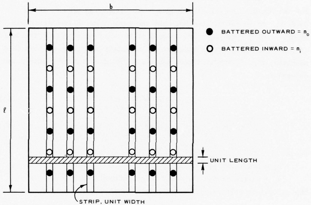
Fig. 6. Schematic representation of monolith
