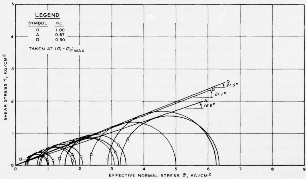
Figure 59. Mohr's diagrams and strength envelopes based on effective stresses taken at (\sigma_1 - \sigma_3)_{\text{max}} for EABPL clay
