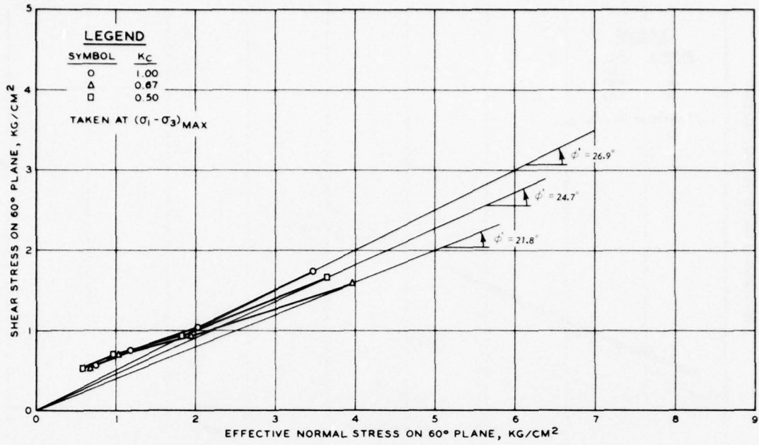
Figure 60. Strength envelopes based on effective stresses on 60-deg plane taken at (\sigma_1 - \sigma_3)_{max} for Buckshot clay
