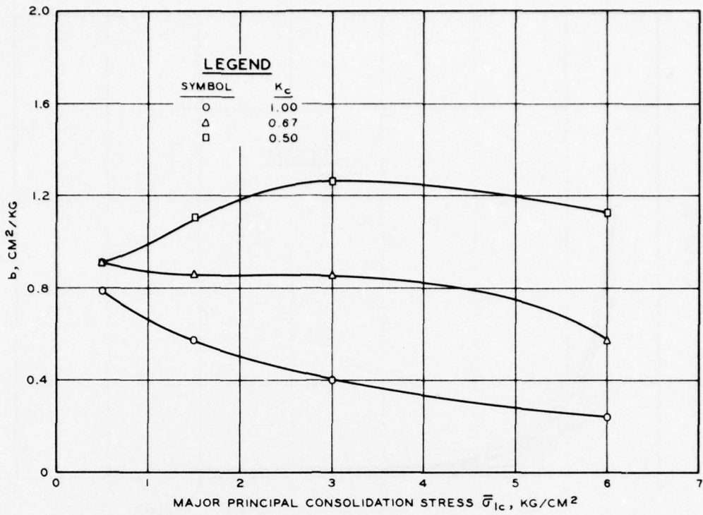
Figure 75. b parameter versus \bar{\sigma}_{1c} for Buckshot clay
