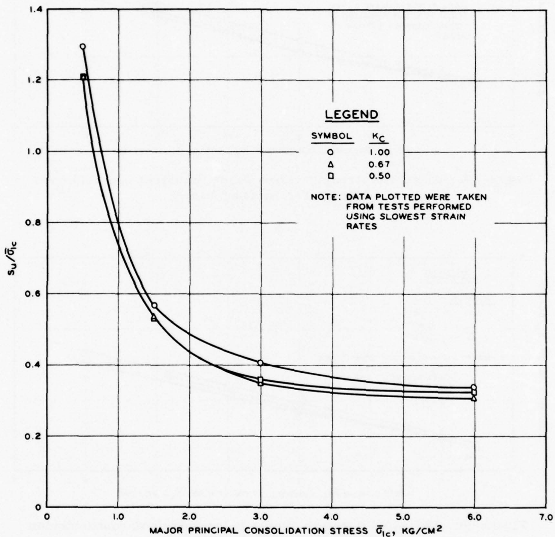
Figure 31. s_u/\bar{\sigma}_{1c} versus major principal consolidation stress for Buckshot clay
