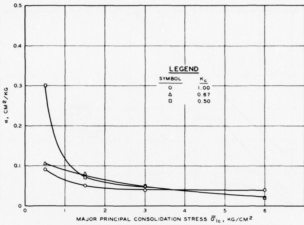
Figure 71. a parameter versus \bar{\sigma}_{lc} for Buckshot clay
