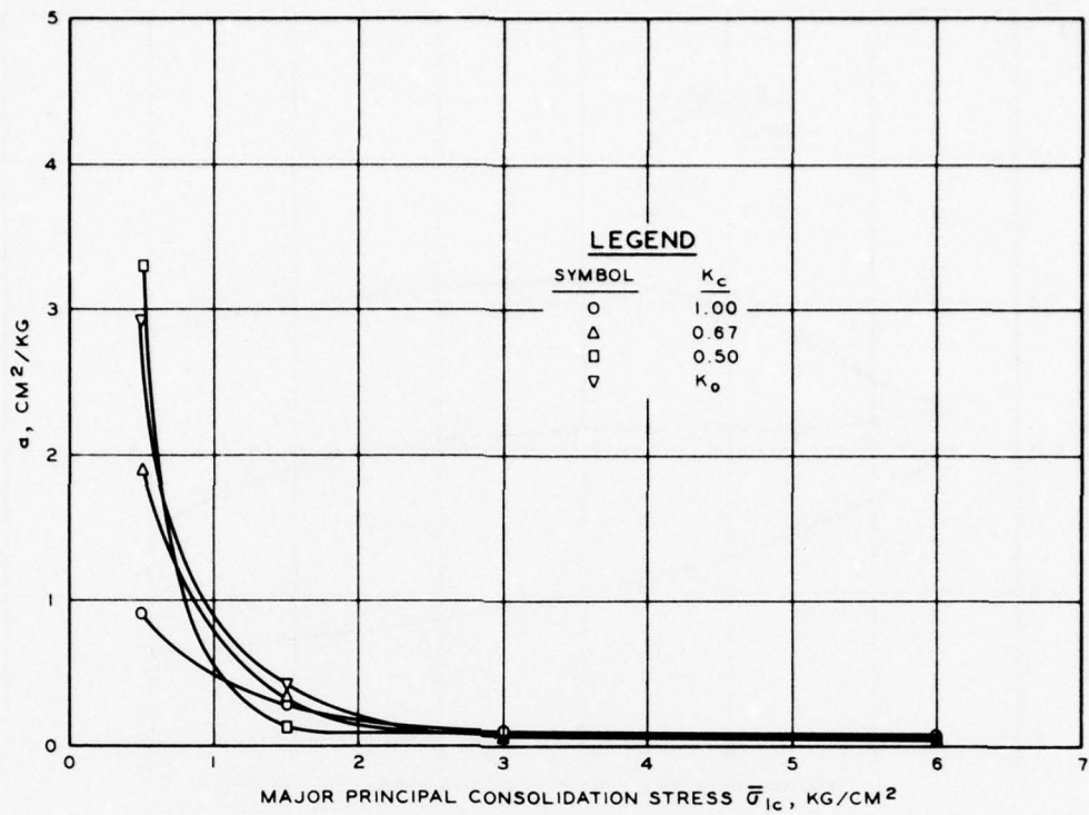
Figure 73. a parameter versus \bar{\sigma}_{lc} for EABPL clay
