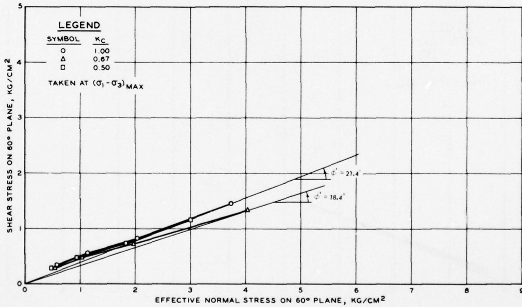
Figure 61. Strength envelopes based on effective stresses on 60-deg plane taken at (\sigma_1 - \sigma_3)_{max} for EABPL clay
