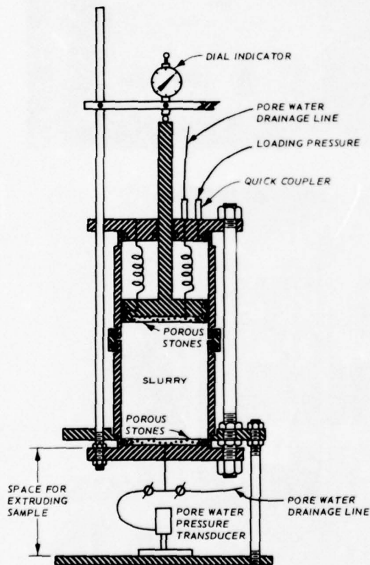
Figure 4. Slurry consolidometer
