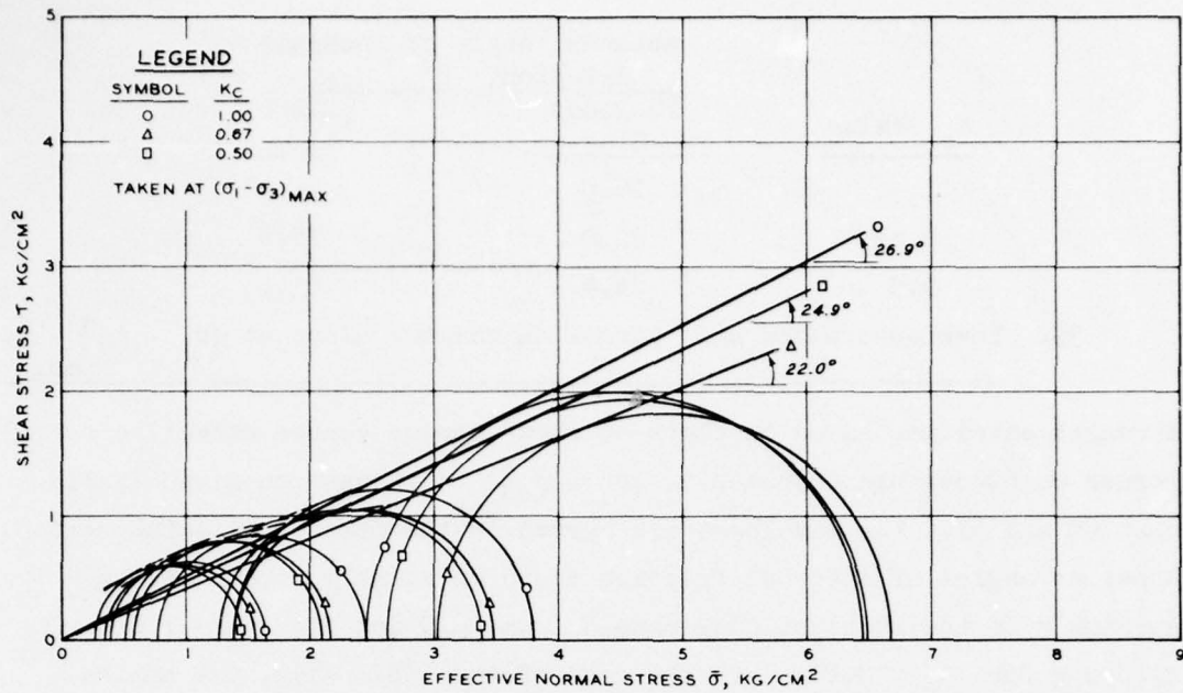
Figure 58. Mohr's diagrams and strength envelopes based on effective stresses taken at (\sigma_1 - \sigma_3)_{\text{max}} for Buckshot clay
