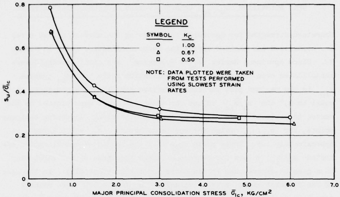
Figure 32. s_u/\bar{\sigma}_{1c} versus major principal consolidation stress for EABPL clay
