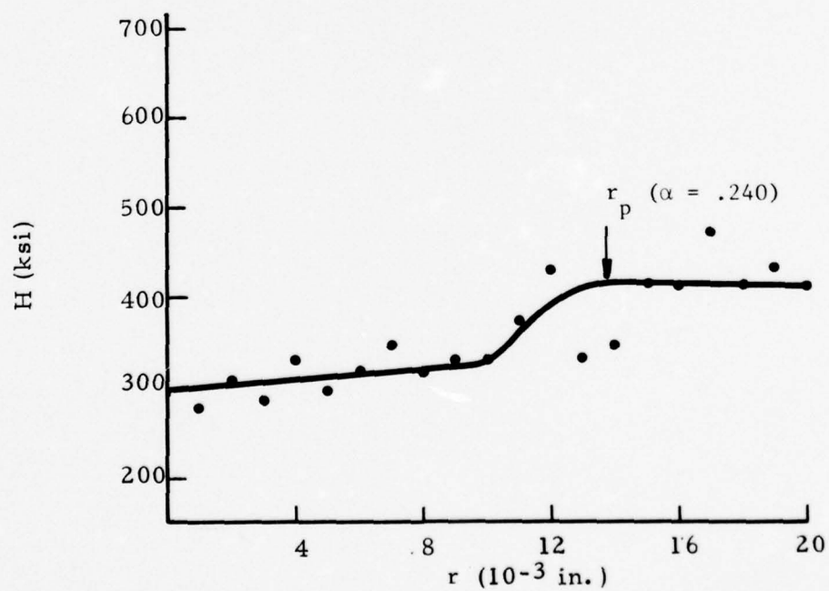
(b) Microhardness Profiles Perpendicular to Crack Plane
