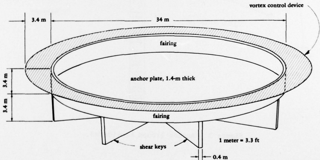
Figure 5. Oblique view of free-fall-emplaced deadweight anchor.
