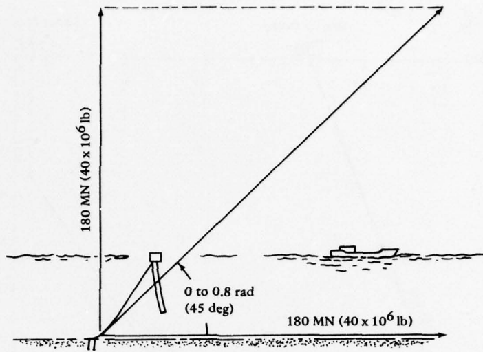
Figure 2. Anchor loadings, Gulf Stream environment, Phase I.
