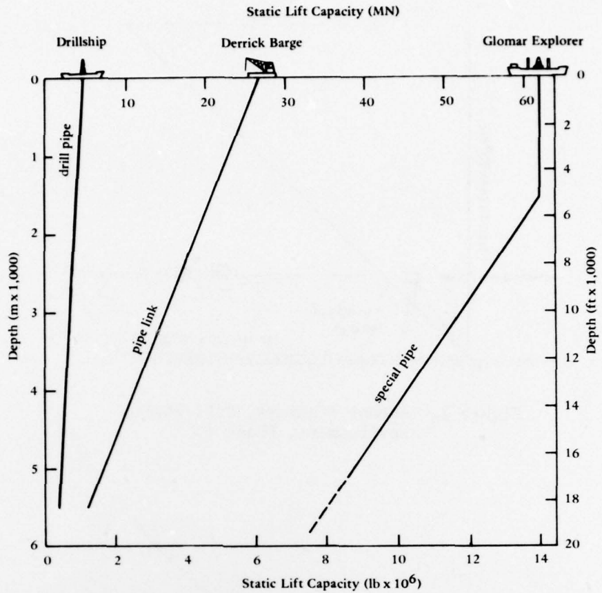
Figure 4. State of the art in heavy-lift vessels.
