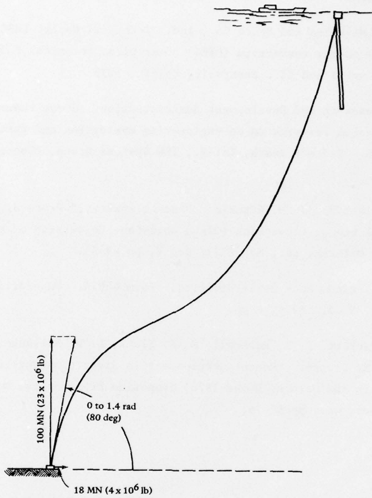
Figure 1. Anchor loadings, deep ocean environment, Phase I.
