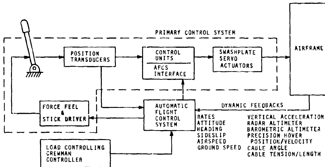
Figure 1. Selected HLH Flight Control System Configuration.
