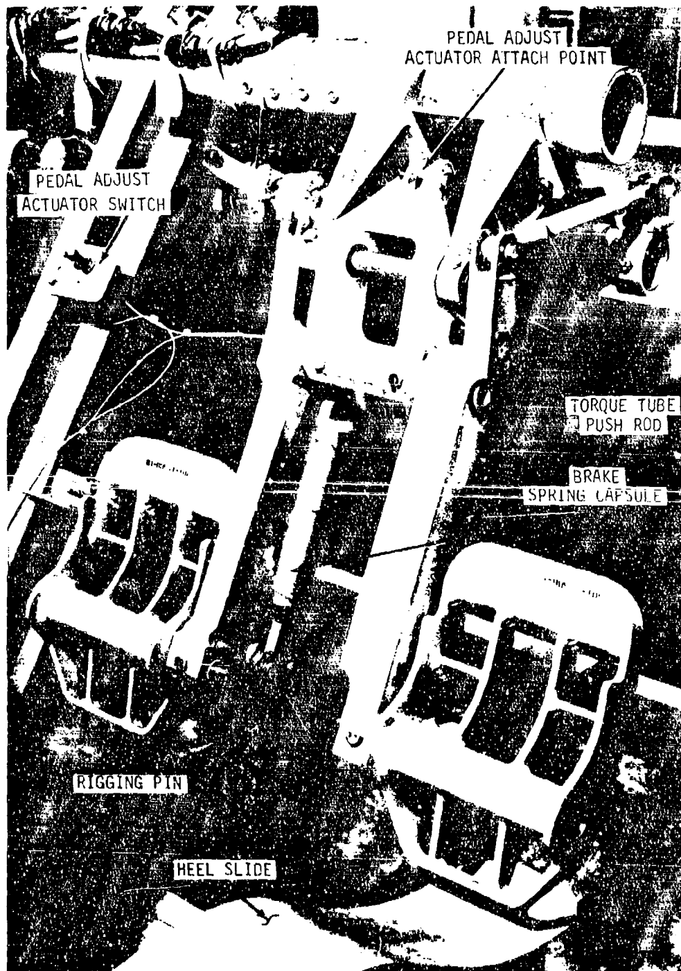
Figure 44. Directional Pedals Adjust and Heel Slides.
