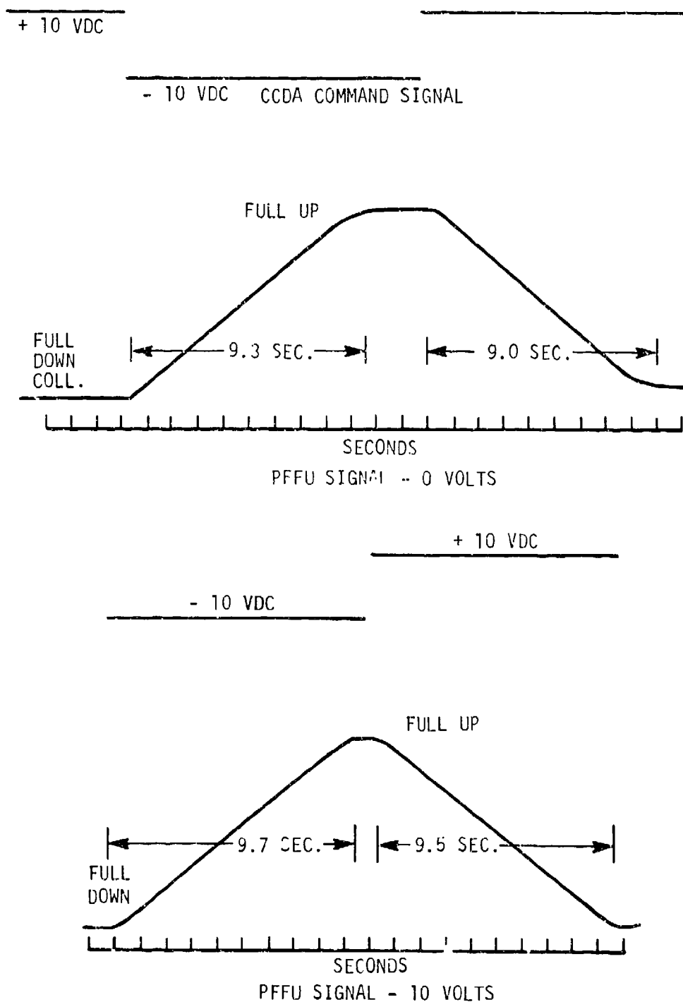
Figure 53. Typical Data, CCDA Drive.
