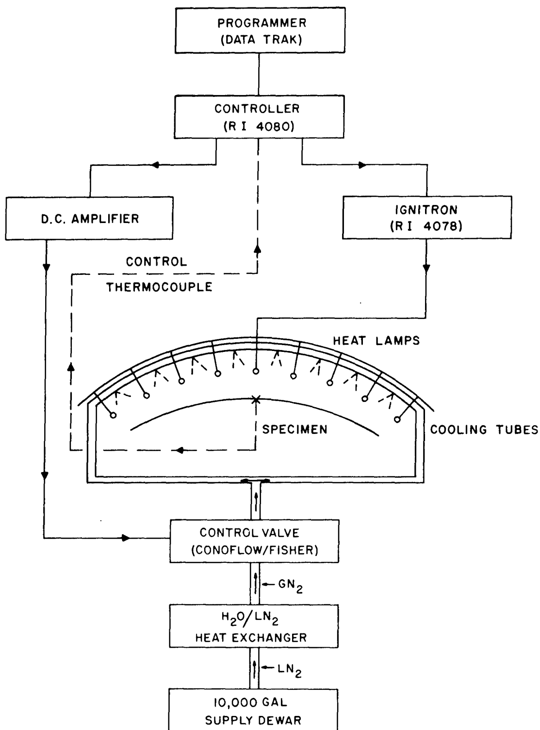
Figure 13. Surface Temperature Control Block Diagram
