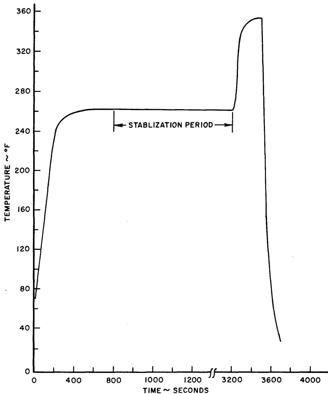
Figure 10. Condition IV, Thermal Profile
