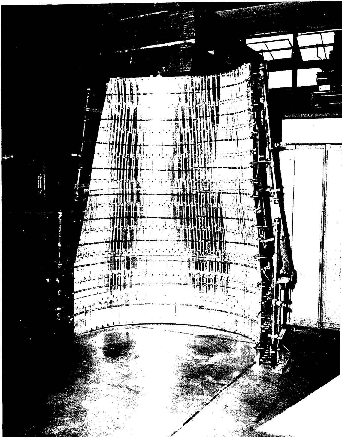
Figure 12. Reflector - Showing Quartz Lamps and Stainless Steel Cooling Tubes
