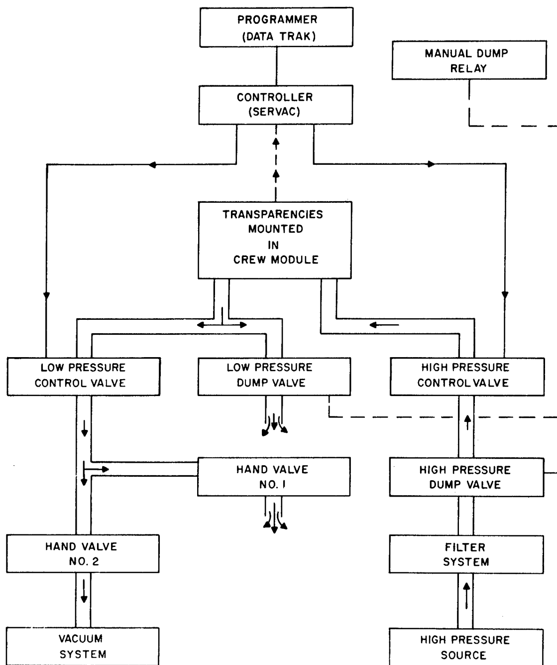
Figure 14. Internal Pressure Control System Block Diagram
