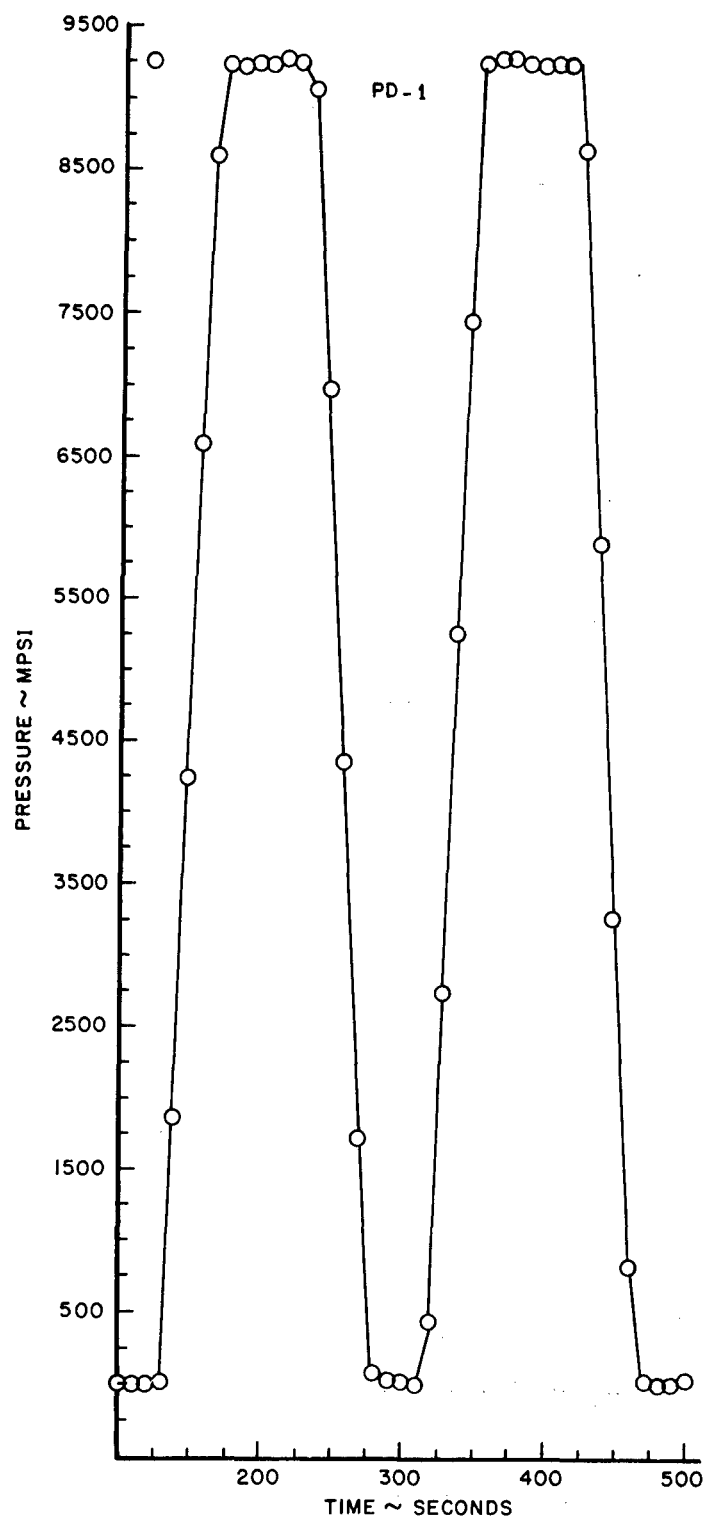
Figure 28. Typical Pressure Response for Condition I
