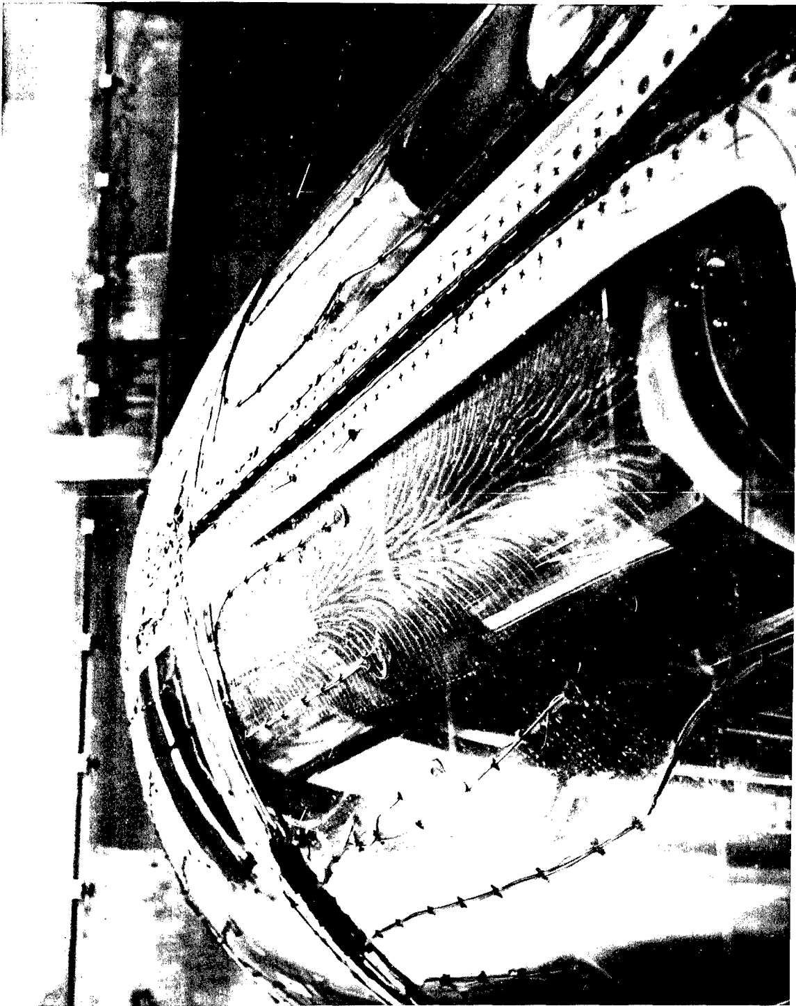
Figure 21. Leaf Shaped Delamination of the Right Windshield Interlayer at the End of the Third Lifetime of Testing
