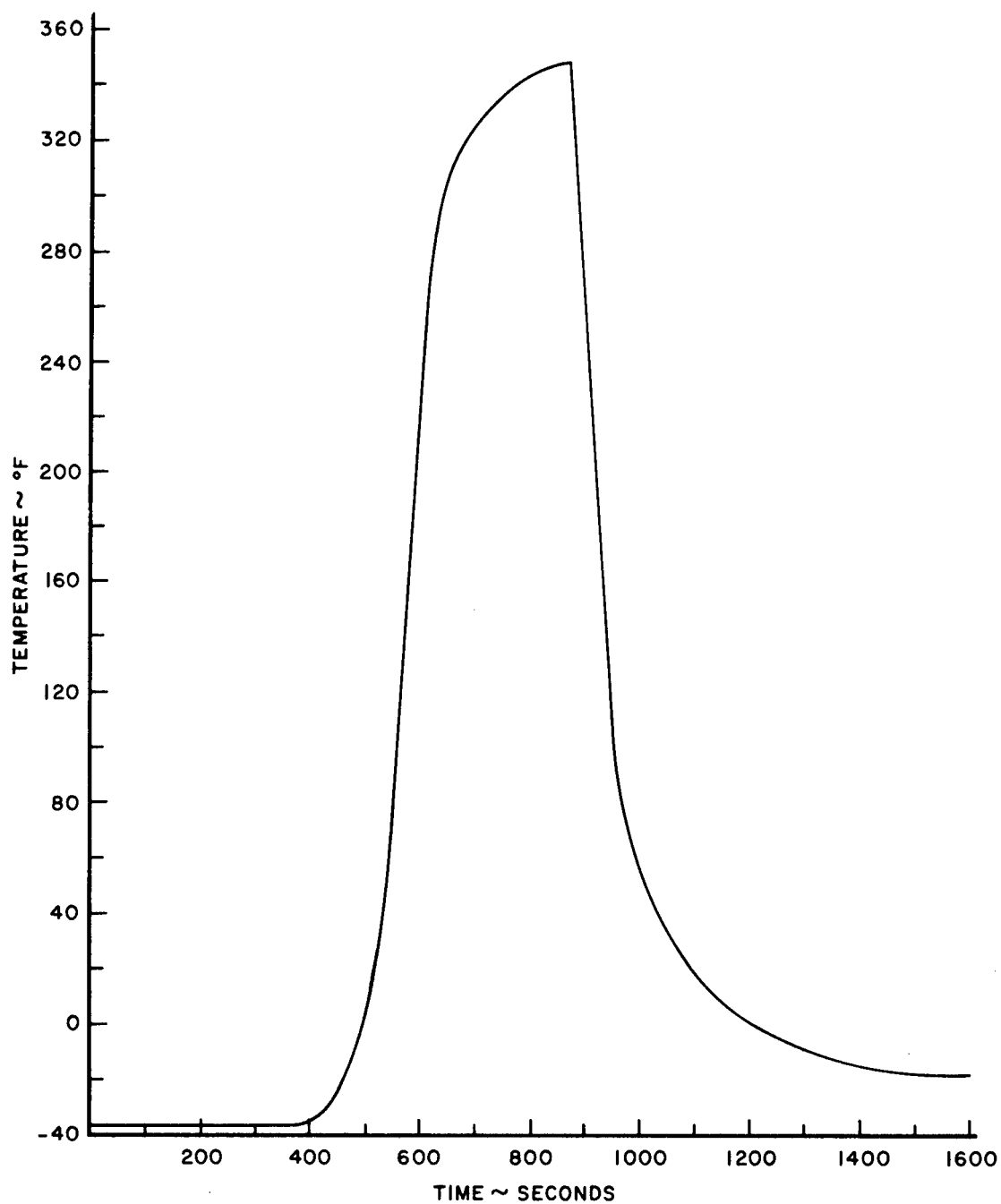
Figure 8. Condition II, Thermal Profile
