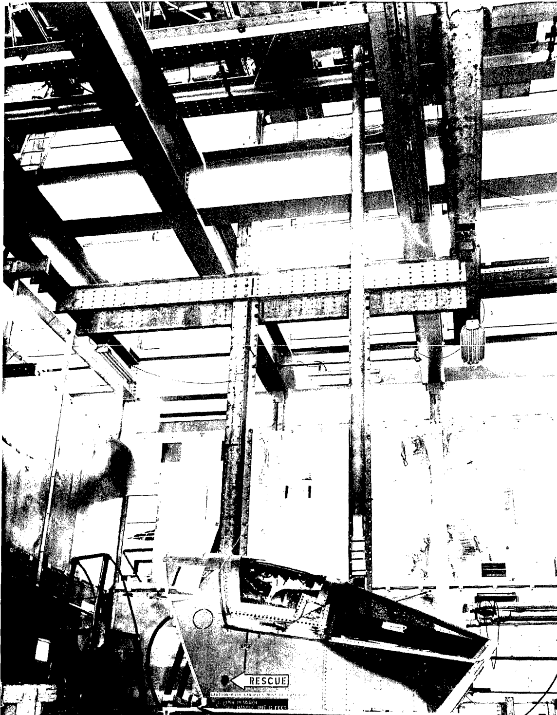
Figure 5. Test Set-Up for Blunt Object Impact Test
