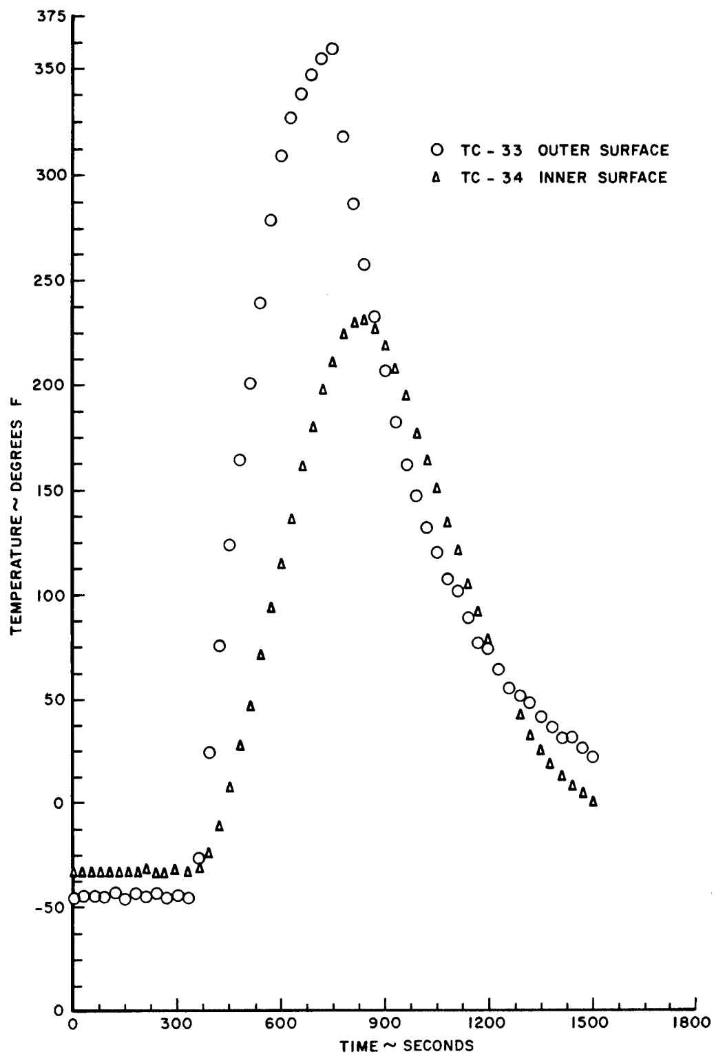
Figure 24. Typical Temperature Response of Inner and Outer Surfaces of the Transparencies for Condition II
