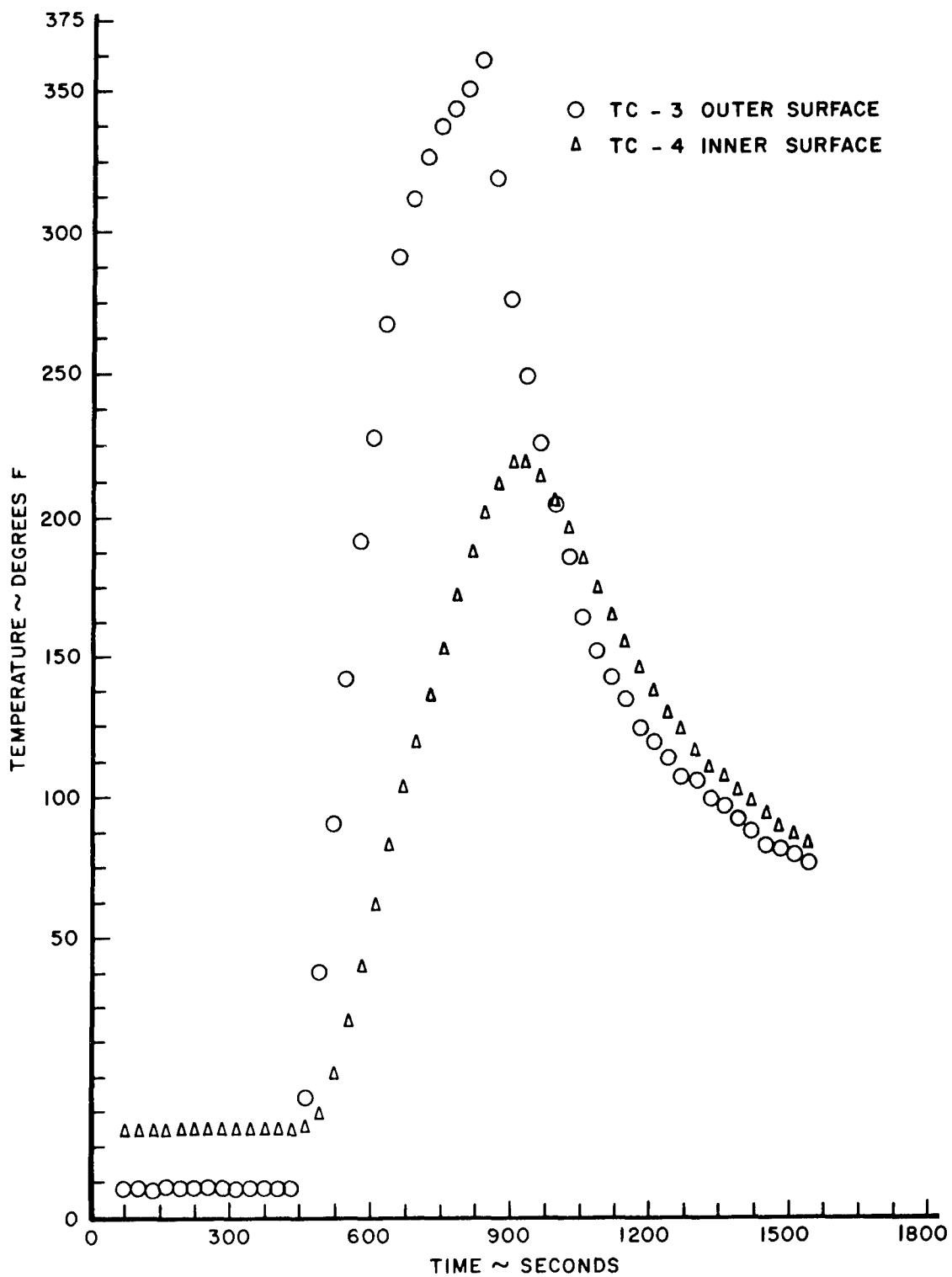
Figure 25. Typical Temperature Response of Inner and Outer Surfaces of the Transparencies for Condition II
