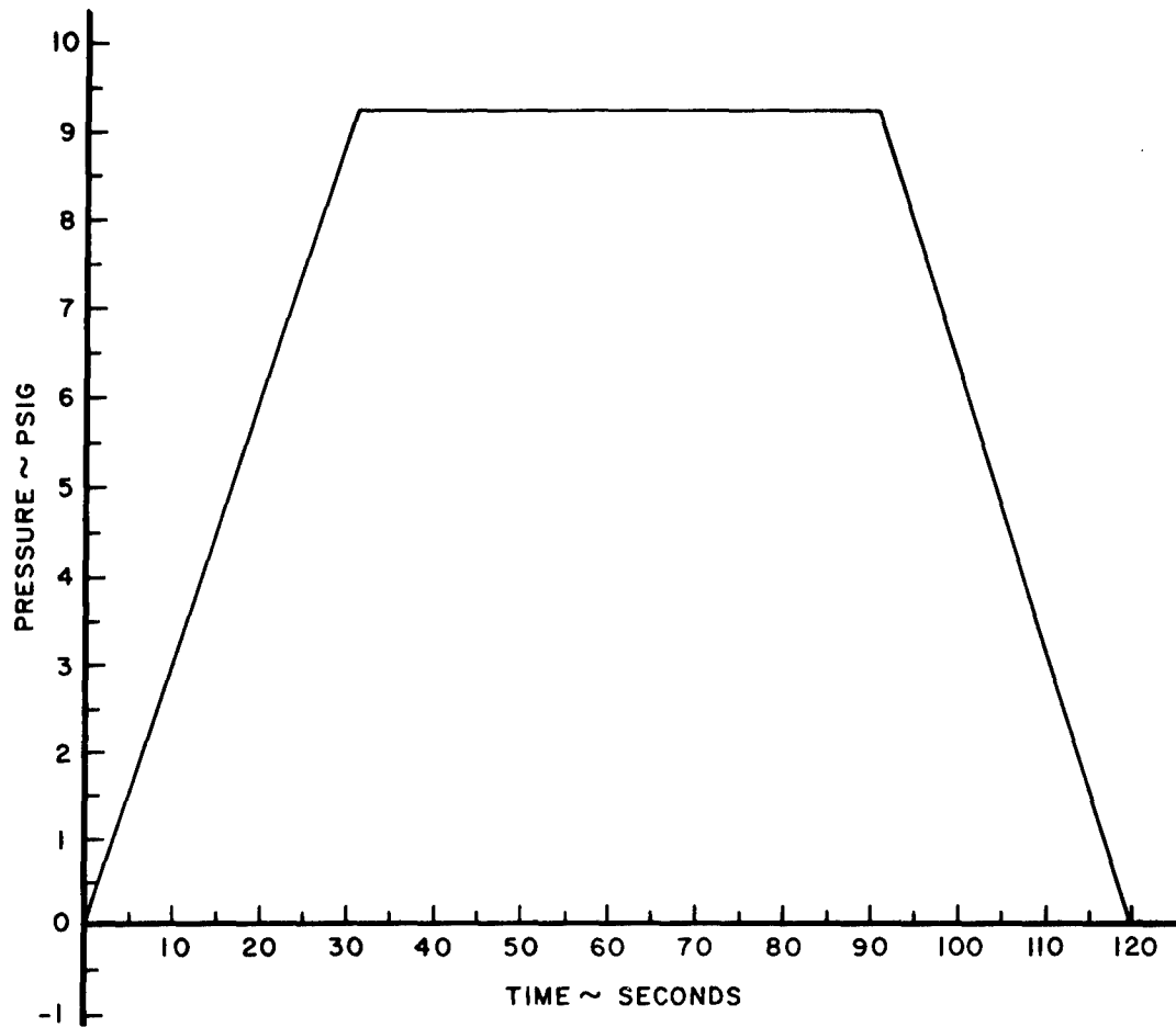
Figure 7. Condition I, Pressure Profile
