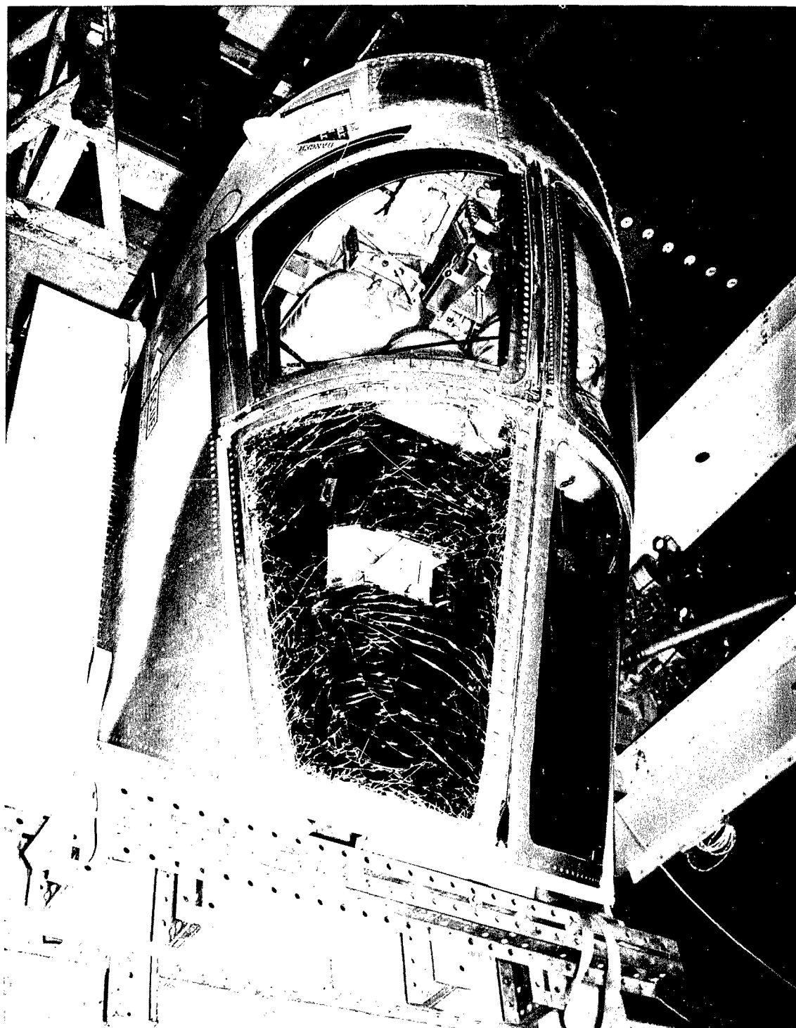
Figure 1. Ship-Set of Debonded Transparencies with the Outer Laminate of Right Windshield Crazed in Edge Member Repair Procedure, Installed in Crew Module
