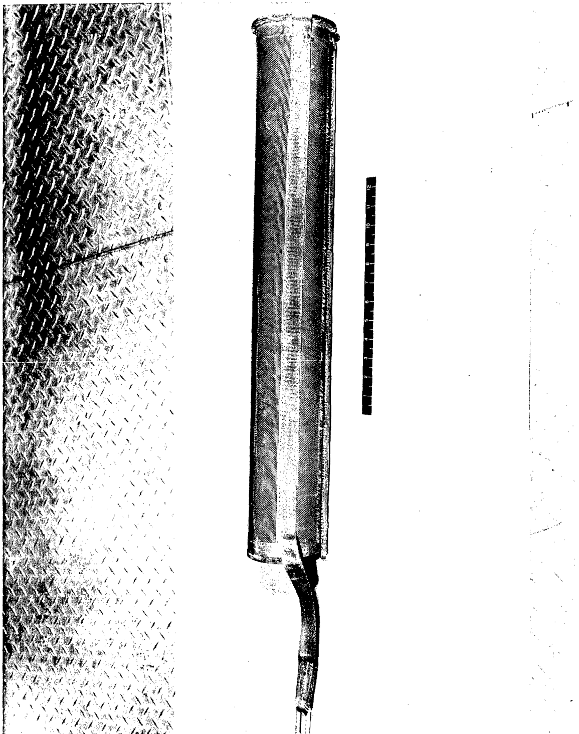
Figure 6. "Bird" Used in Blunt Object Impact Test
