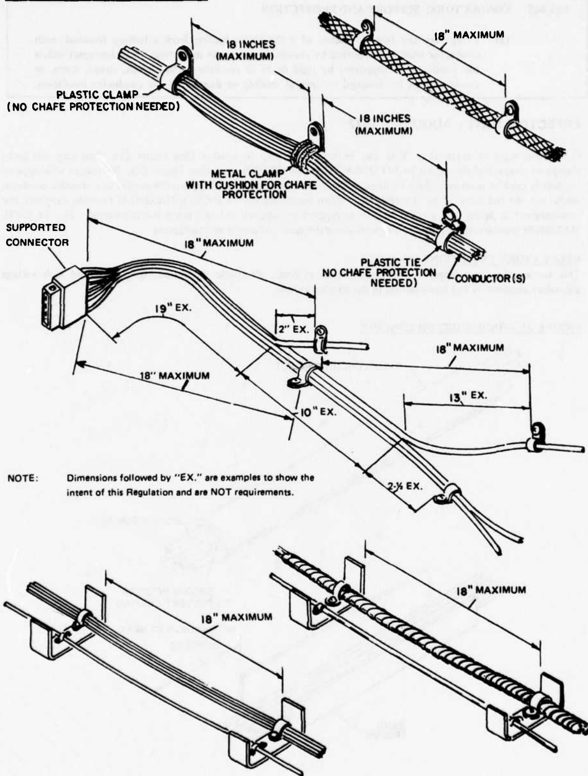
FIGURE 22 – CONDUCTOR SUPPORT
