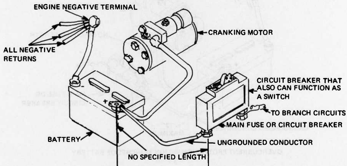
OVERCURRENT PROTECTION WITH SWITCH
