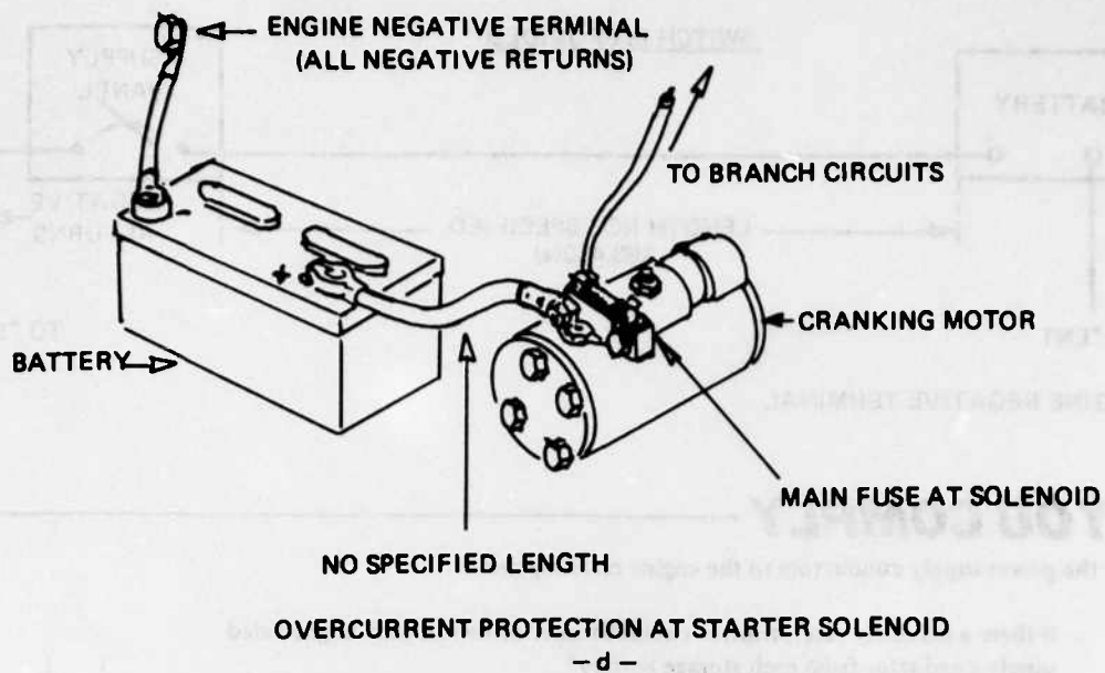
FIGURE 40 -- TYPICAL SUPPLY CIRCUITS
