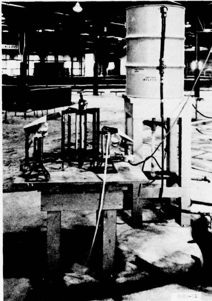
Figure 14. Section of vertical plunger wave generator
