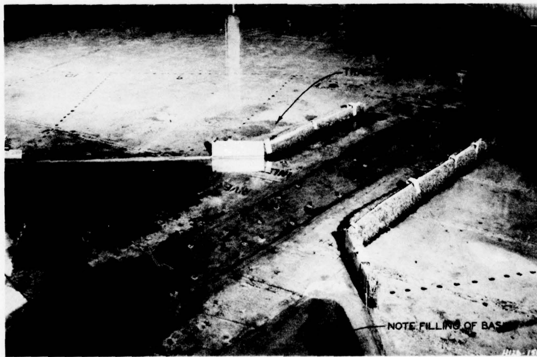
Figure 42. Post test 16 (Littoral Drift Injection Test)
