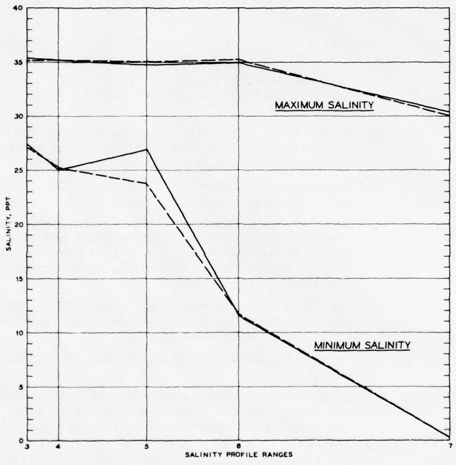
Figure 47. Bottom salinity profiles
