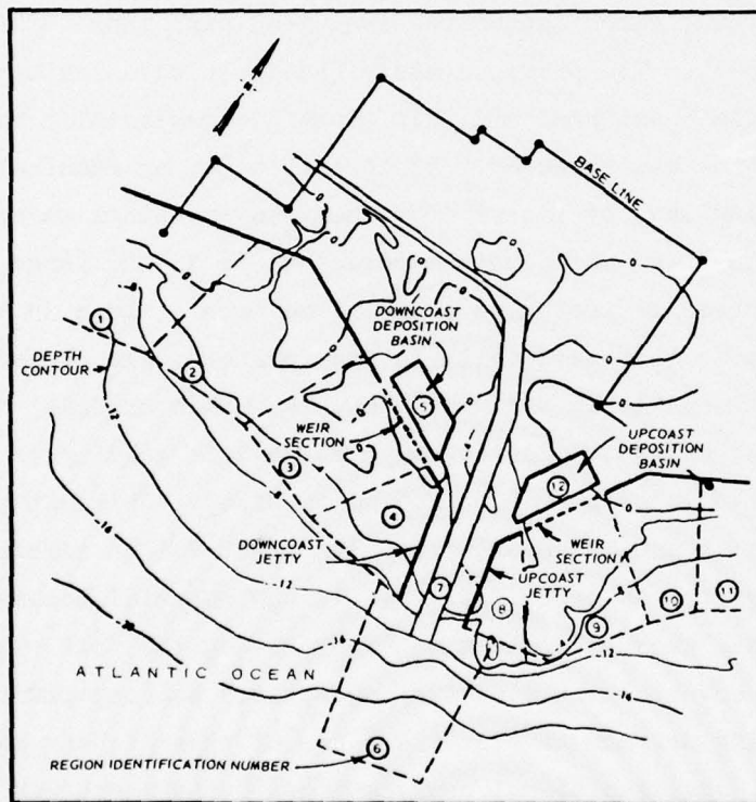
Figure 40. Location of model sediment regions
