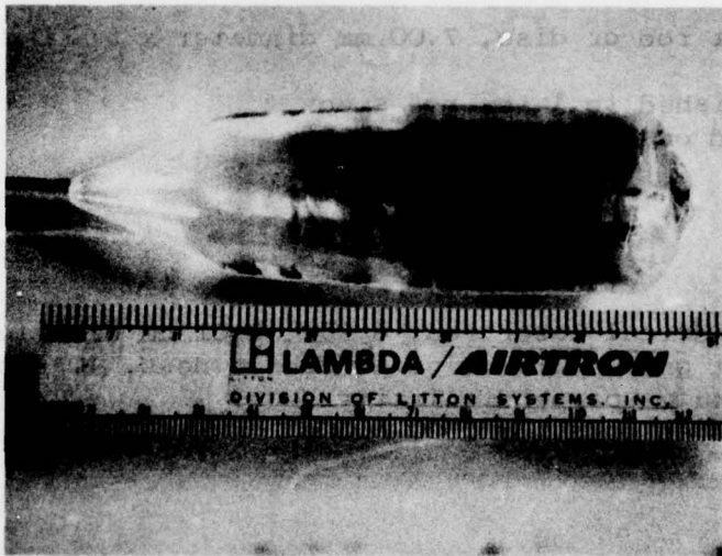
Figure 4. Grown boules of YAG:Ce (a) 0.05% Ce (b) 0.5% Ce
