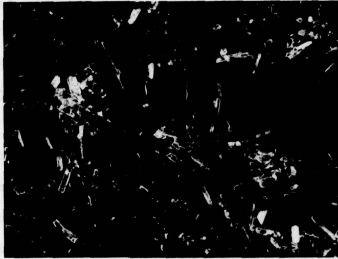
Figure 5. Flux grown GdVO_4:Pr crystals.
