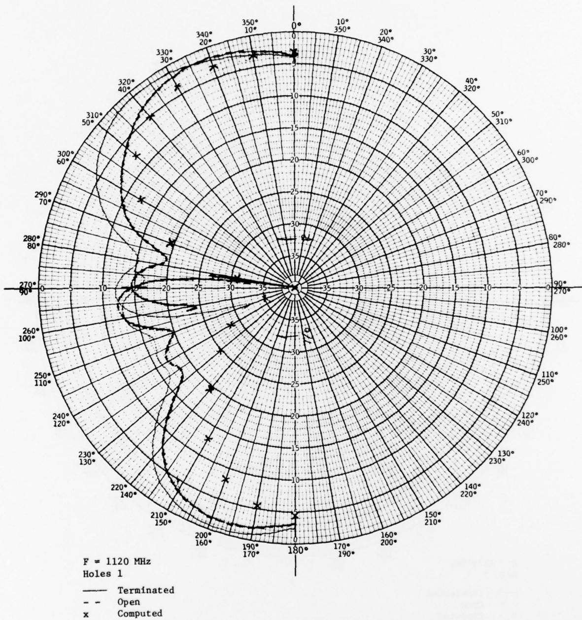
Figure 30. Four Antenna Vertical Pattern \approx 0.5\lambda Spacing.
