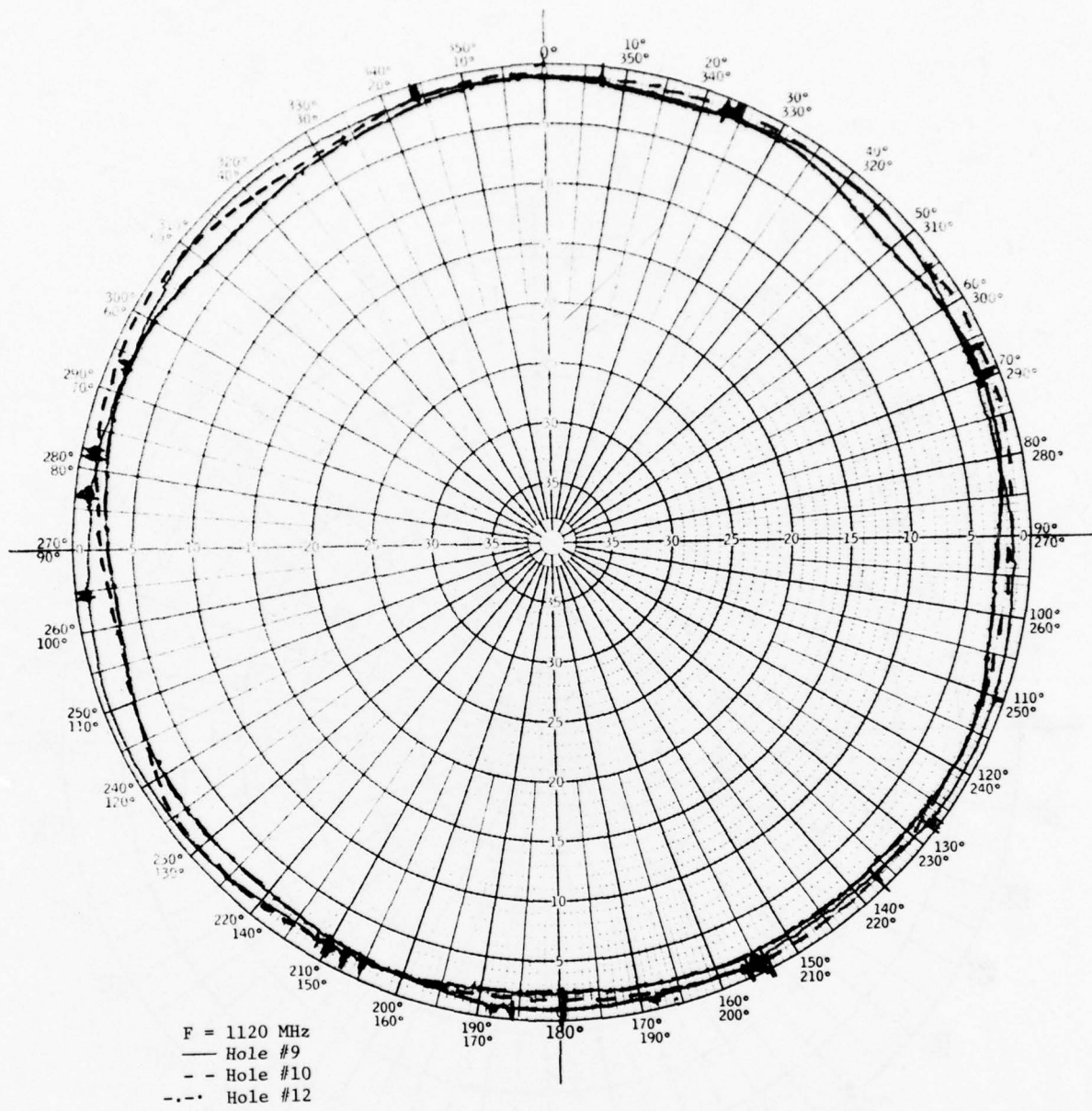
Figure 11. Effect of Mounting Antenna Off-Center.
