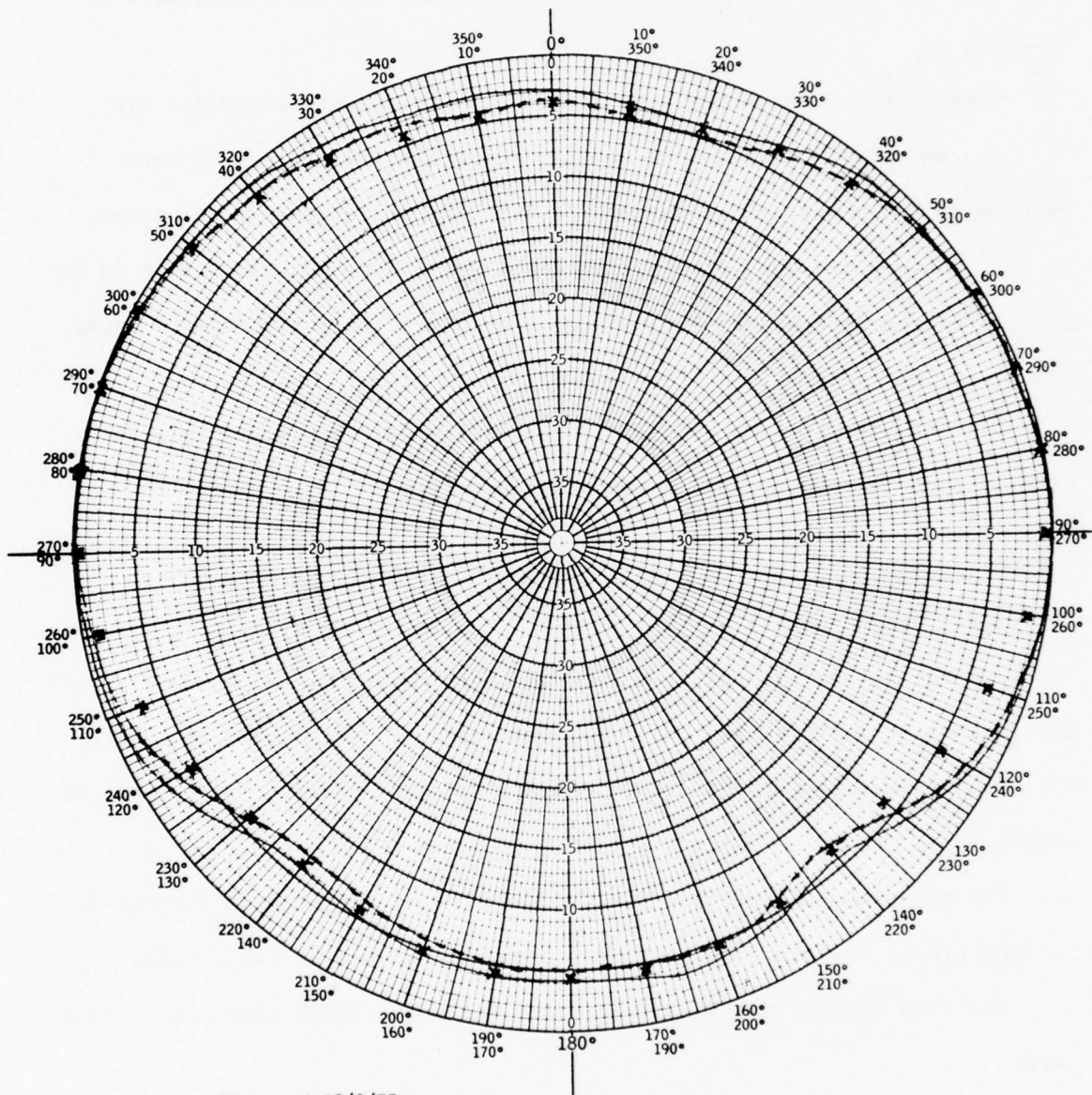
Figure 27. Measurement at Two Different Dates - Two Antenna Horizontal Pattern \sim 0.5\lambda Separation.
