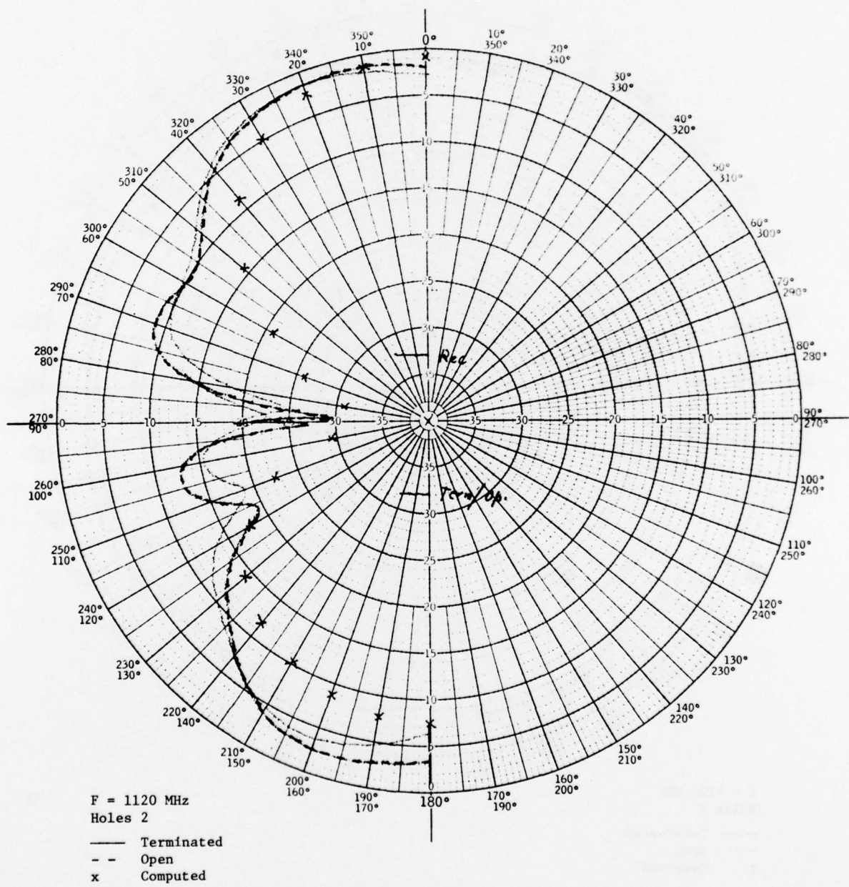
Figure 32. Four Antenna Vertical Pattern \sim 0.75\lambda Spacing.
