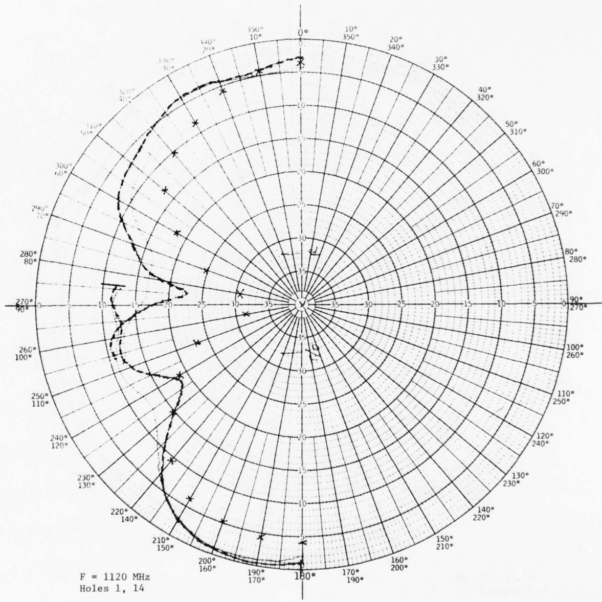
Figure 26. Two Antenna Vertical Pattern \sim 2.0\lambda Spacing.
