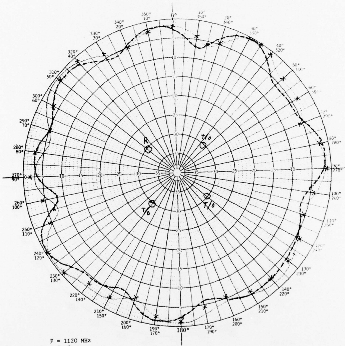
Figure 37. Four Antenna Horizontal Pattern \sim 1.5\lambda Spacing.
