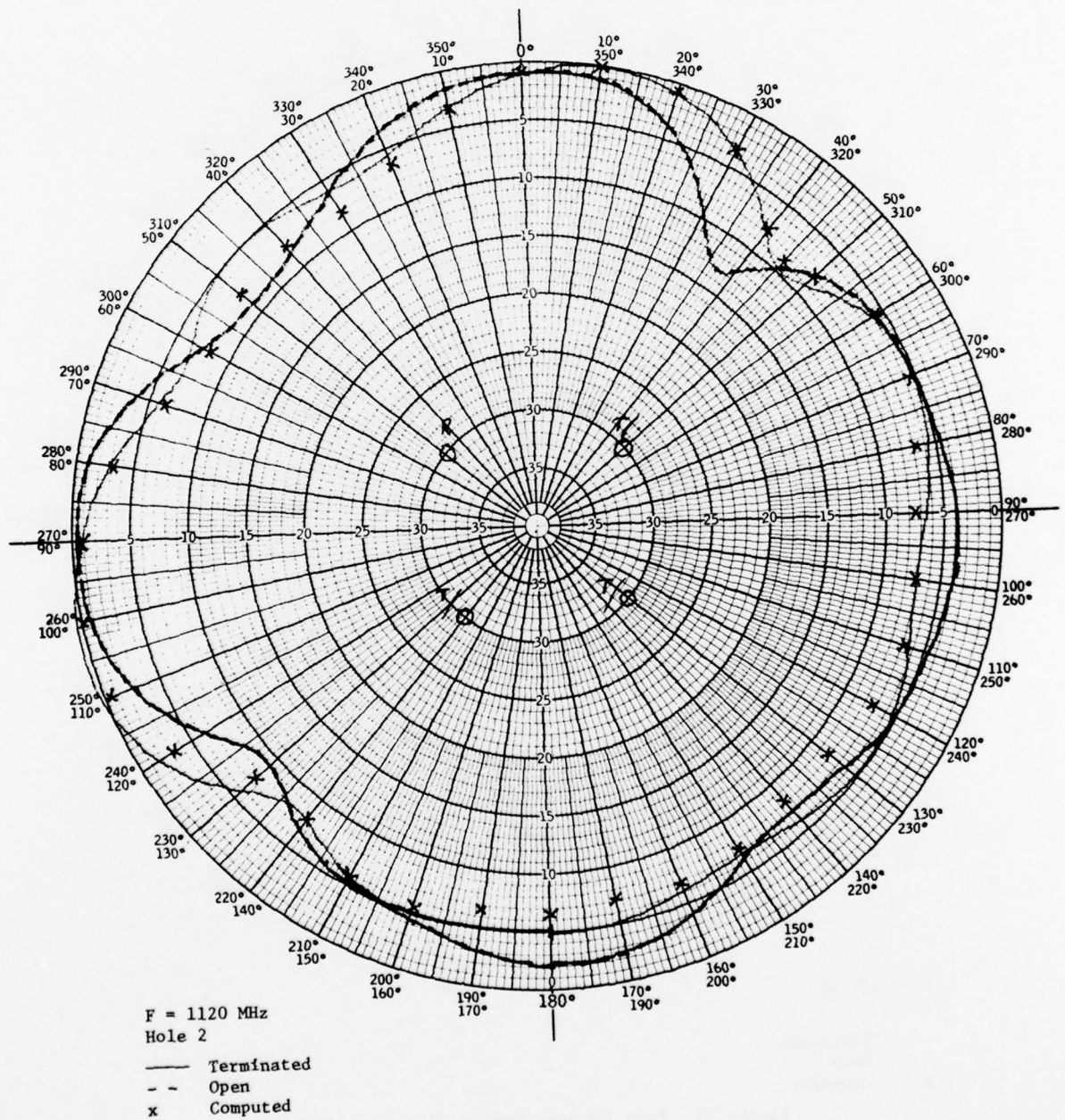
Figure 31. Four Antenna Horizontal Pattern \sim 0.75\lambda Spacing.
