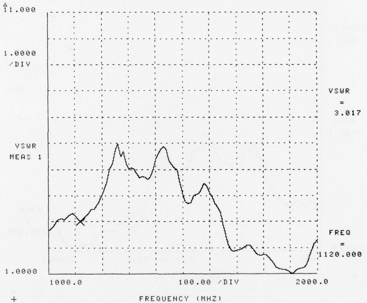
Figure 6. Antenna 10 VSWR Plot.
