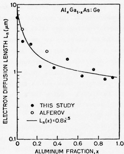
Fig. 4.4. ELECTRON DIFFUSION LENGTH VS Al CONCENTRATION x IN (p)Al_xGa_{1-x}As:Ge SINGLE CRYSTALS.
