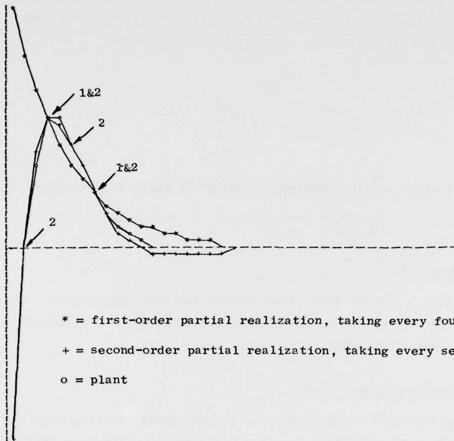
Fig. 1.1. IMPULSE RESPONSES VS FIRST- AND SECOND-ORDER REALIZATIONS. Arrows indicate sample instants where the impulse responses of the plant coincide with that of the model (first order, second order, or both are indicated by the numbers at the arrows).
