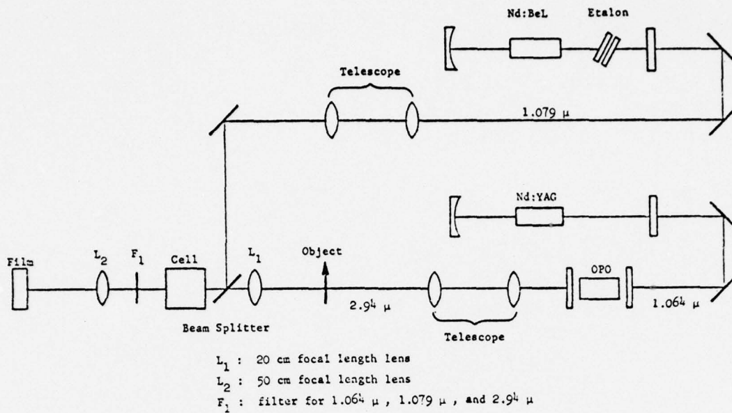
Fig. 6.2. EXPERIMENTAL SETUP.
