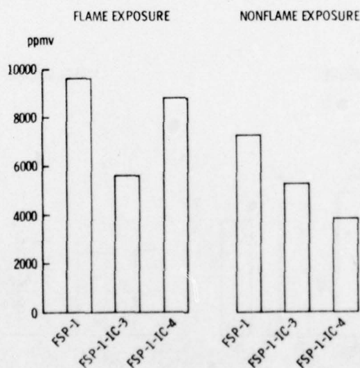
Figure 23. The Effect of Intumescent Coatings on Maximum Hydrocarbons Concentrations Developed from 1/4-in.-Thick Samples of FSP-1
