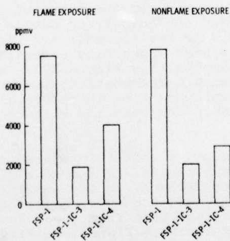
Figure 19. The Effect of Intumescent Coatings on Maximum HCl Concentrations Developed from 1/4-in.-Thick Samples of FSP-1
