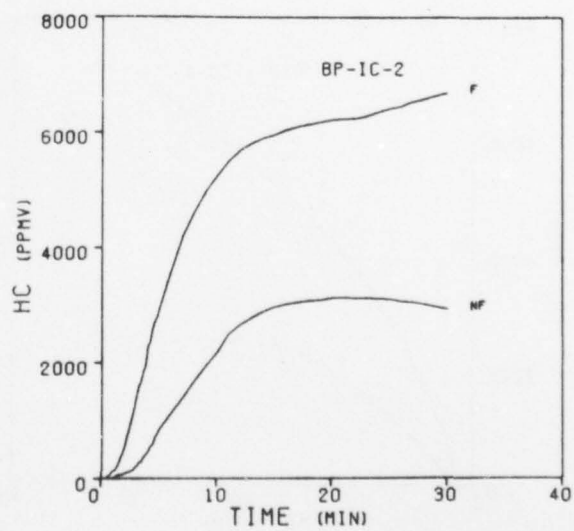
Figure 49. Hydrocarbons Concentrations During the Burning of BP-IC Compositions
