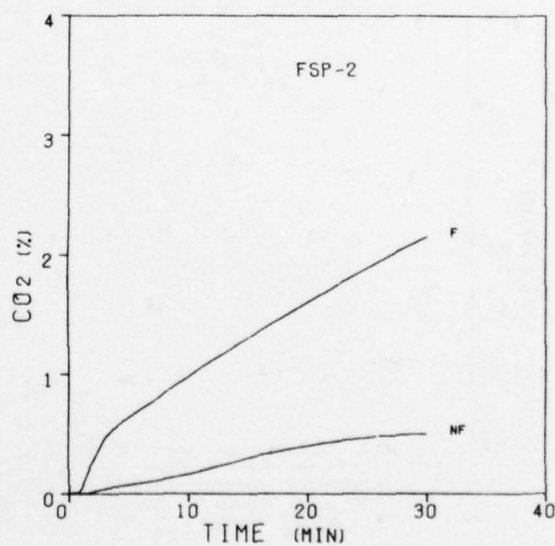
Figure 33. Carbon Dioxide Concentrations During the Burning of PVC Compositions
