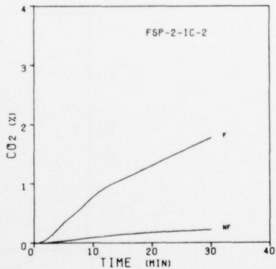
Figure 43. Carbon Dioxide Concentrations During the Burning of FSP-2-IC Compositions
