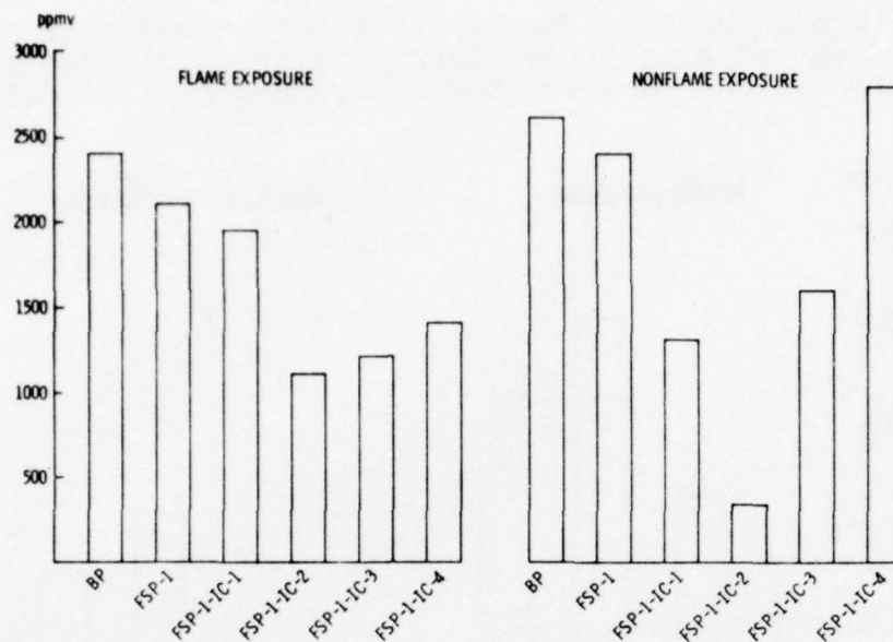
Figure 18. The Effect of Intumescent Coatings on Maximum HCl Concentrations Developed from 1/16-in.-Thick Samples of FSP-1
