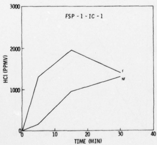
Figure 54. HCl Concentrations During the Burning of FSP-1-IC Compositions
