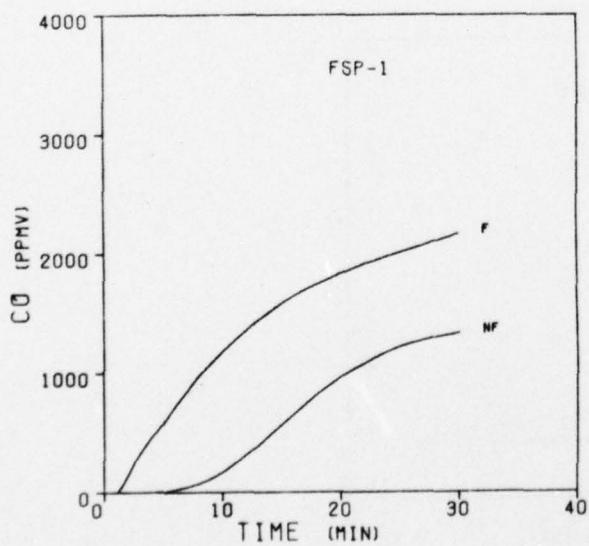
Figure 32. Carbon Monoxide Concentrations During the Burning of PVC Compositions
