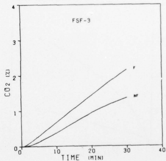
Figure 57. Carbon Dioxide Concentrations During the Burning of Experimental Neoprene Foam Compositions
