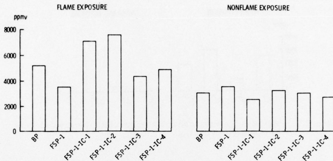
Figure 20. The Effect of Intumescent Coatings on Maximum Hydrocarbons Concentrations Developed from 1/16-in.-Thick Samples of FSP-1
