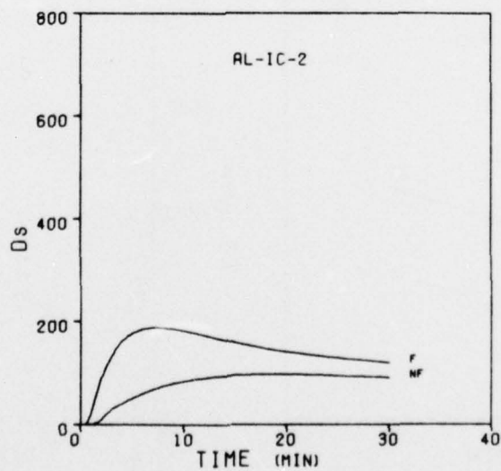
Figure 31. Smoke Optical Densities During the Exposure of Al-IC Compositions
