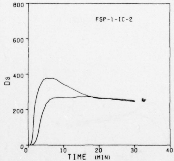
Figure 29. Smoke Optical Densities During the Burning of FSP-1-IC Compositions
