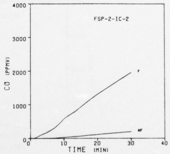
Figure 39. Carbon Monoxide Concentrations During the Burning of FSP-2-IC Compositions
