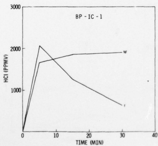
Figure 53. HCl Concentrations During the Burning of BP-IC Compositions
