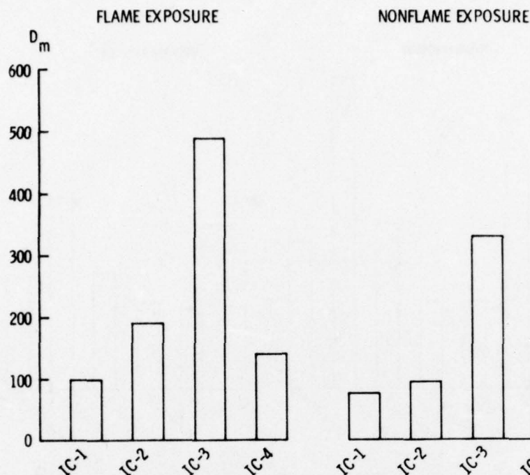
Figure 8. Maximum Smoke Optical Densities Generated from Intumescent Coatings, Applied Onto Aluminum Foil
