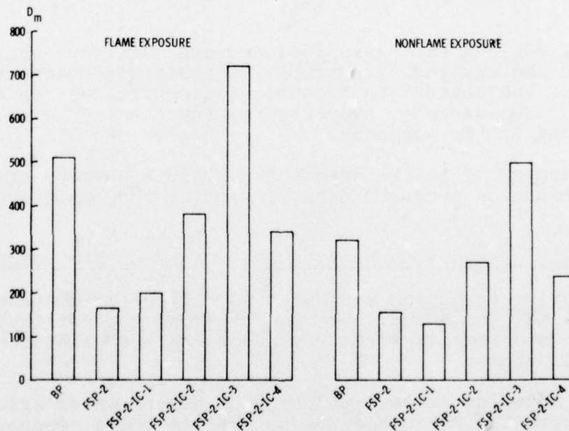
Figure 7. The Effect of Intumescent Coatings on Smoke Formation from 1/16-in.-Thick Samples of FSP-2
