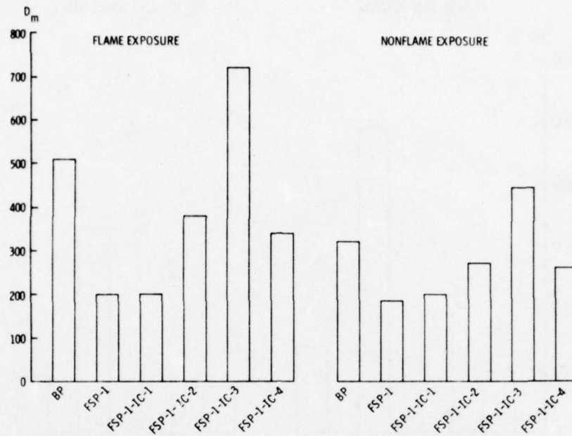
Figure 6. The Effect of Intumescent Coatings on Smoke Formation from 1/16-in.-Thick Samples of FSP-1
