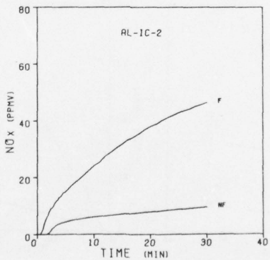
Figure 48. NO x Concentrations during the Exposure of Al-IC Compositions
