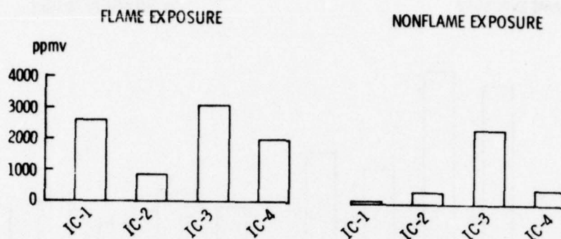
Figure 22. Maximum Hydrocarbons Concentrations Generated from Intumescent Coatings
