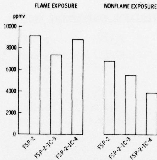
Figure 24. The Effect of Intumescent Coatings on Maximum Hydrocarbons Concentrations Developed from 1/4-in.-Thick Samples of FSP-2
