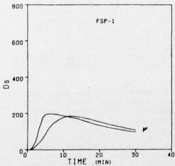
Figure 4. Smoke Optical Densities During the Burning of 1/16-in.-Thick Samples of PVC Compositions in the NBS-Aminco Chamber
