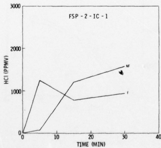
Figure 55. HCl Concentrations During the Burning of FSP-2-IC Compositions
