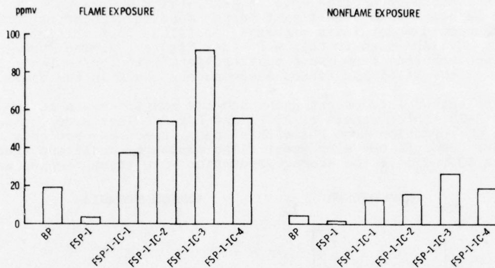
Figure 15. The Effect of Intumescent Coatings on Maximum NO x Concentrations Developed from 1/16-in.-Thick Samples of FSP-1
