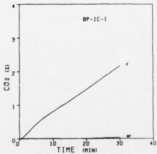
Figure 41. Carbon Dioxide Concentrations During the Burning of BP-IC Compositions
