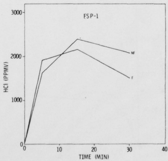
Figure 36. HCl Concentrations During the Burning of PVC Compositions
