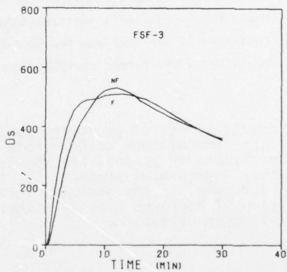
Figure 27. Smoke Optical Densities During the Burning of Experimental Neoprene Foam Compositions
