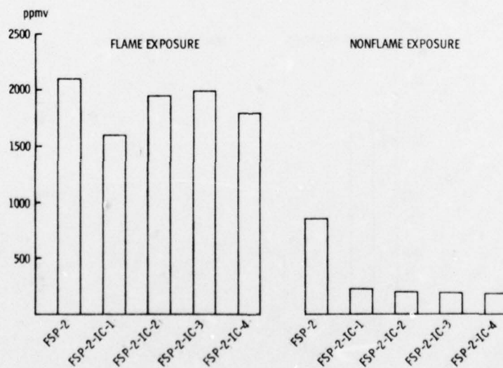
Figure 11. The Effect of Intumescent Coatings on Maximum CO Concentrations Developed from 1/16-in.-Thick Samples of FSP-2
