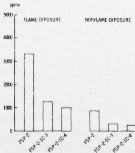
Figure 13. The Effect of Intumescent Coatings on Maximum CO Concentrations Developed from 1/4-in.-Thick Samples of FSP-2
