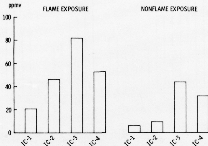
Figure 17. Maximum \text{NO}_x Concentrations Generated from Intumescent Coatings
