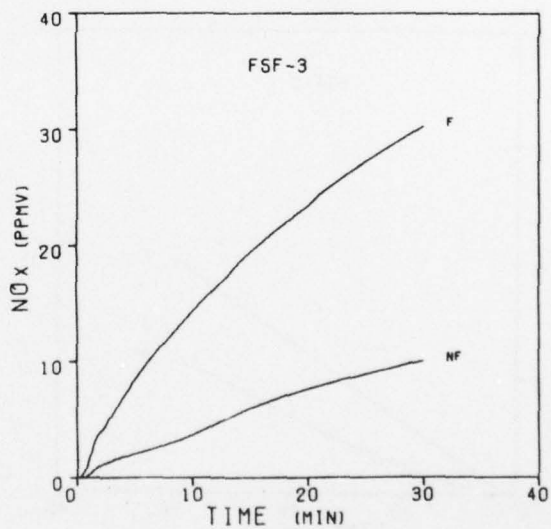
Figure 58. NO x Concentrations During the Burning of Experimental Neoprene Foam Compositions
