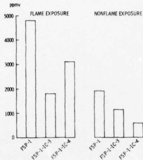
Figure 12. The Effect of Intumescent Coatings on Maximum CO Concentrations Developed from 1/4-in.-Thick Samples of FSP-1
