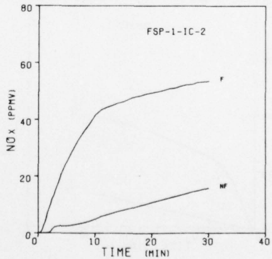
Figure 46. NO x Concentrations During the Burning of FSP-1-IC Compositions
