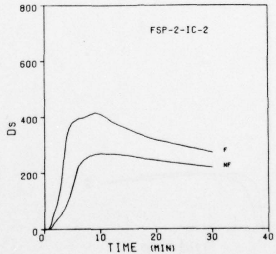
Figure 30. Smoke Optical Densities During the Burning of FSP-2-IC Compositions
