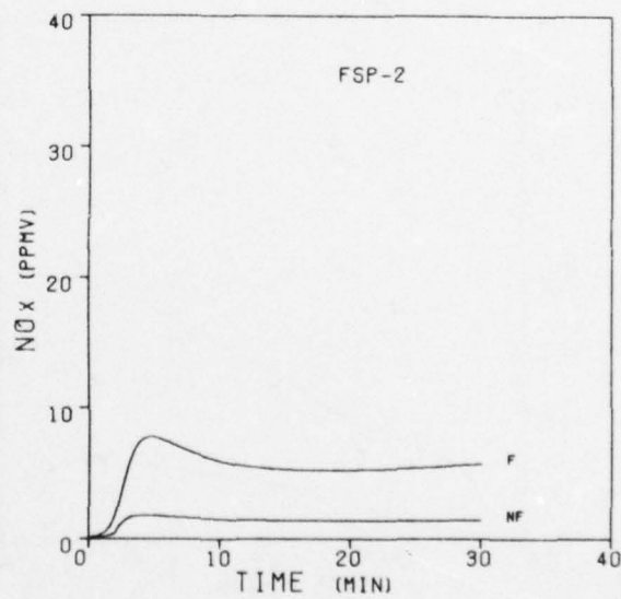
Figure 34. NO x Concentrations During the Burning of PVC Compositions
