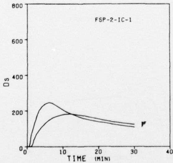
Figure 30. Smoke Optical Densities During the Burning of FSP-2-IC Compositions
