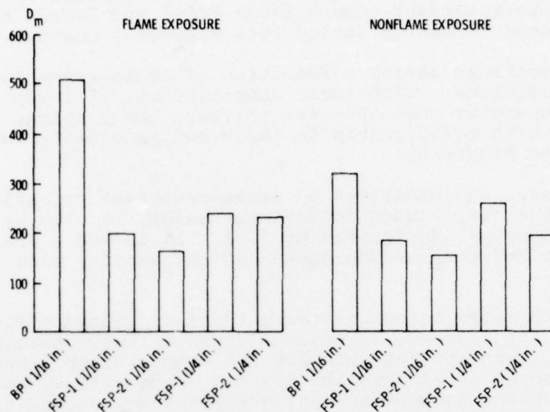
Figure 5. Maximum Specific Smoke Optical Densities of FSP Compositions
