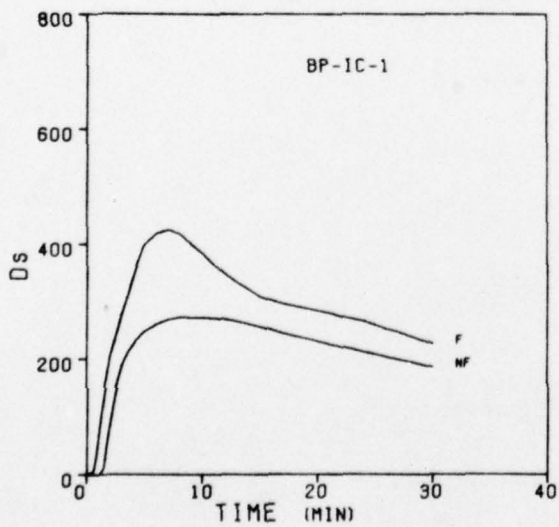
Figure 28. Smoke Optical Densities During the Burning of BP-IC Compositions
