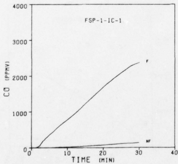
Figure 38. Carbon Monoxide Concentrations During the Burning of FSP-1-IC Compositions
