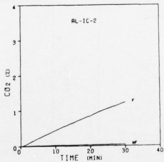
Figure 44. Carbon Dioxide Concentrations During the Exposure of Al-IC Compositions
