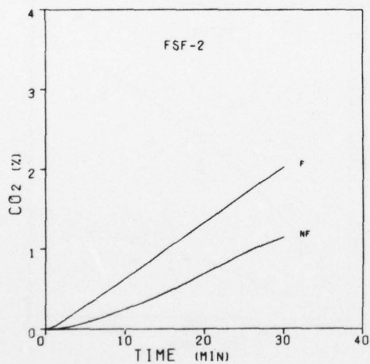
Figure 57. Carbon Dioxide Concentrations During the Burning of Experimental Neoprene Foam Compositions
