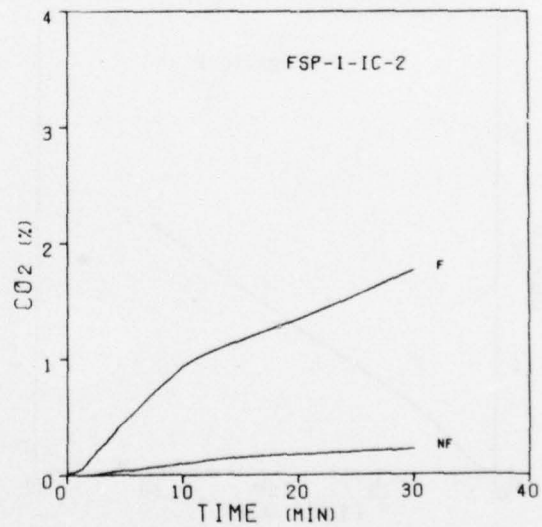
Figure 42. Carbon Dioxide Concentrations During the Burning of FSP-1-IC Compositions
