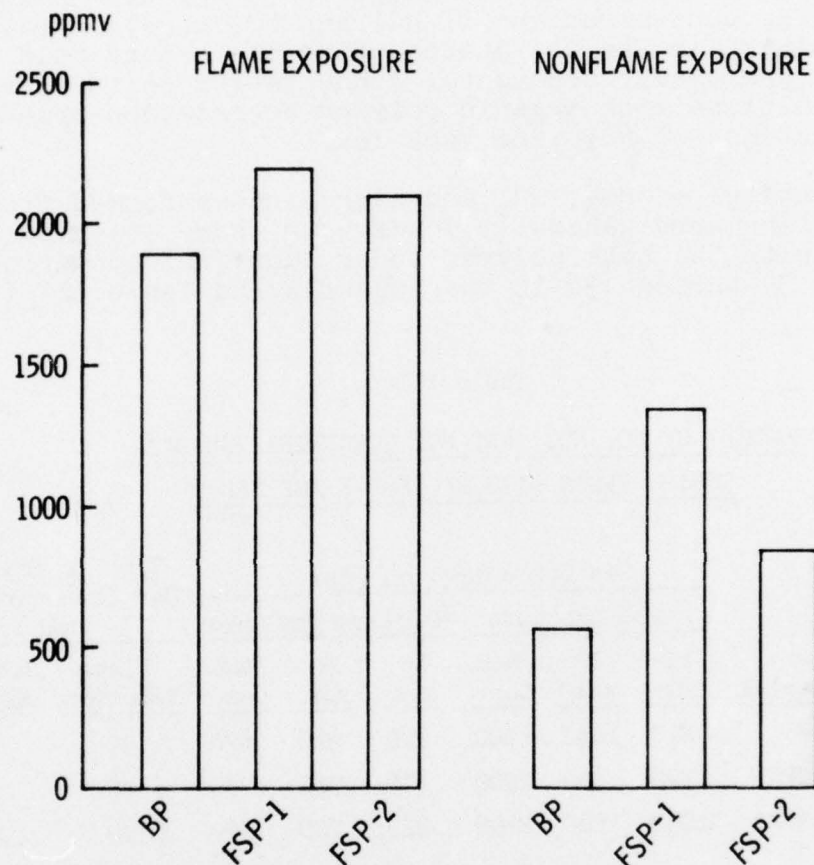
Figure 9. Maximum CO Concentrations Generated From BP and From the FSP Compositions
