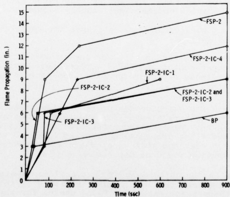
Figure 26. Flame Propagation by FSP-2 Compositions
