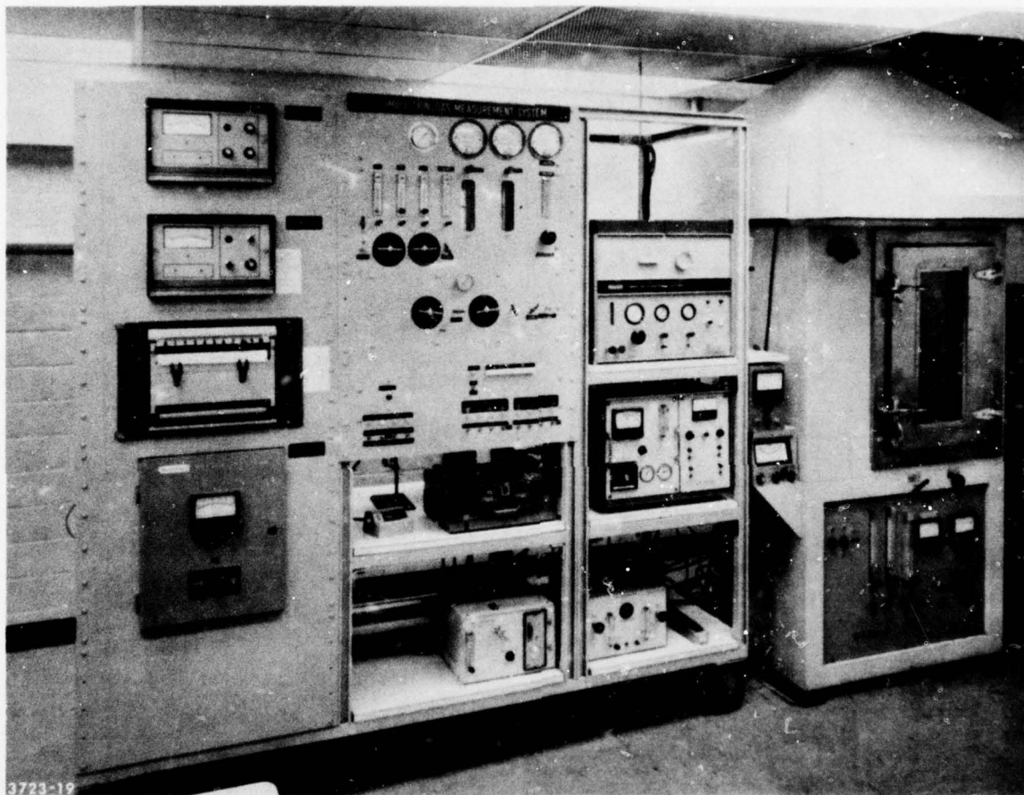
Figure 1. Apparatus for Gaseous Combustion Products and Smoke Optical Density Measurement
