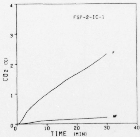
Figure 43. Carbon Dioxide Concentrations During the Burning of FSP-2-IC Compositions
