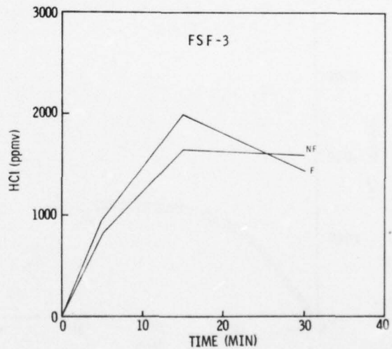
Figure 60. HCl Concentrations During the Burning of Experimental Neoprene Foam Compositions
