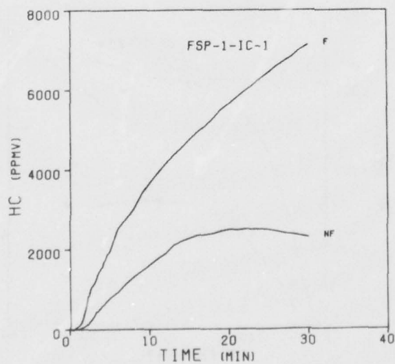
Figure 50. Hydrocarbons Concentrations During the Burning of FSP-1-IC Compositions
