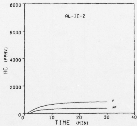
Figure 52. Hydrocarbons Concentrations During the Exposure of Al-IC Compositions
