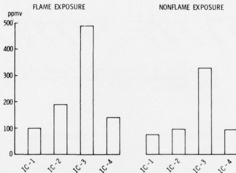
Figure 14. Maximum CO Concentrations Generated From Intumescent Coatings
