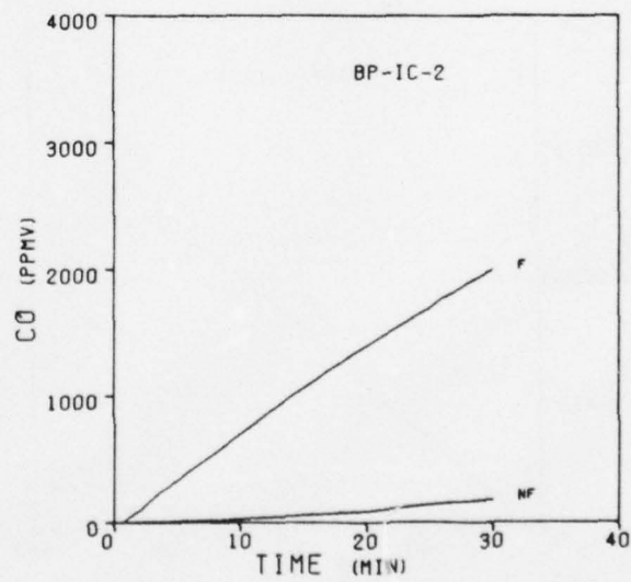
Figure 37. Carbon Monoxide Concentrations During the Burning of BP-IC Compositions
