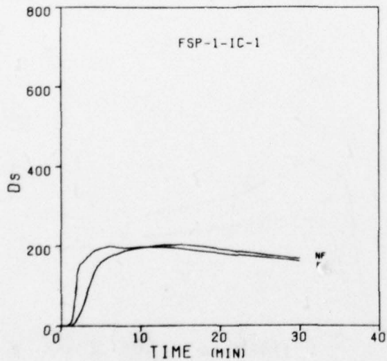
Figure 29. Smoke Optical Densities During the Burning of FSP-1-IC Compositions
