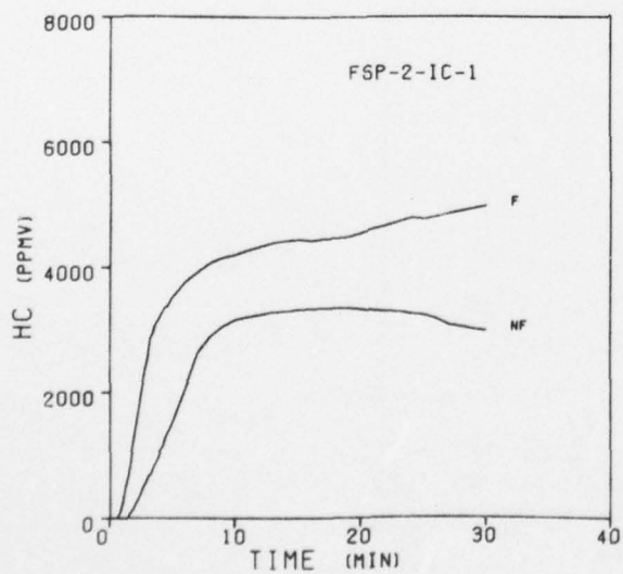
Figure 51. Hydrocarbons Concentrations During the Burning of FSP-2-IC Compositions
