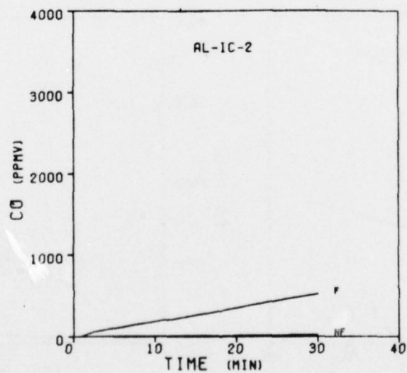
Figure 40. Carbon Monoxide Concentrations During the Exposure of Al-IC Compositions
