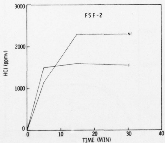
Figure 60. HCl Concentrations During the Burning of Experimental Neoprene Foam Compositions
