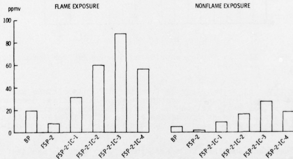
Figure 16. The Effect of Intumescent Coatings on Maximum NO x Concentrations Developed from 1/16-in.-Thick Samples of FSP-2
