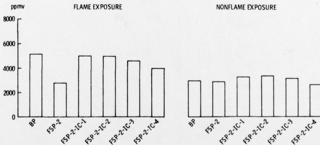
Figure 21. The Effect of Intumescent Coatings on Maximum Hydrocarbons Concentrations Developed from 1/16-in.-Thick Samples of FSP-2
