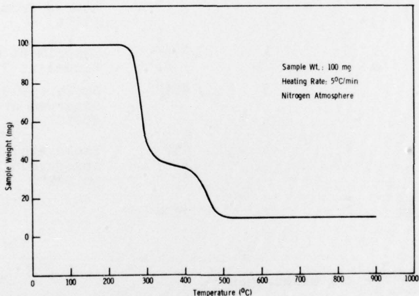
Figure 3. Thermogram of Polyvinyl Chloride (Opalon 650) Degradation
