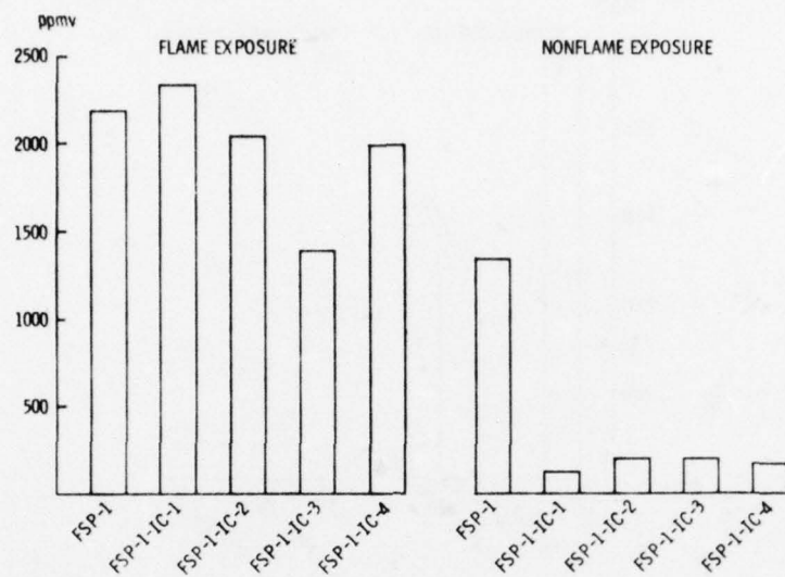
Figure 10. The Effect of Intumescent Coatings on Maximum CO Concentrations Developed from 1/16-in.-Thick Samples of FSP-1
