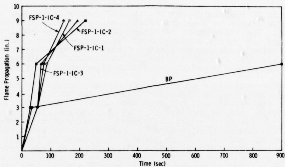
Figure 25. Flame Propagation by FSP-1 Compositions
