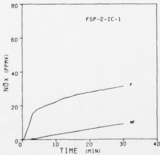
Figure 47. \text{NO}_x Concentrations During the Burning of FSP-2-IC Compositions
