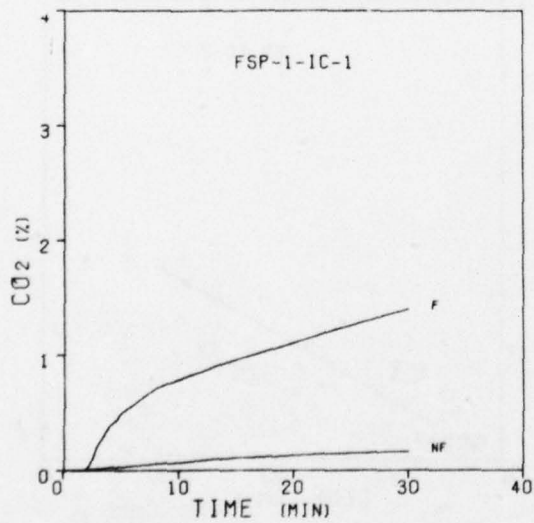
Figure 42. Carbon Dioxide Concentrations During the Burning of FSP-1-IC Compositions
