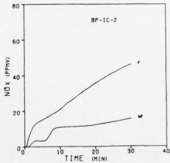
Figure 45. NO x Concentrations During the Burning of BP-IC Compositions
