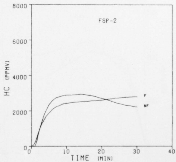
Figure 35. Hydrocarbons Concentrations During the Burning of PVC Compositions
