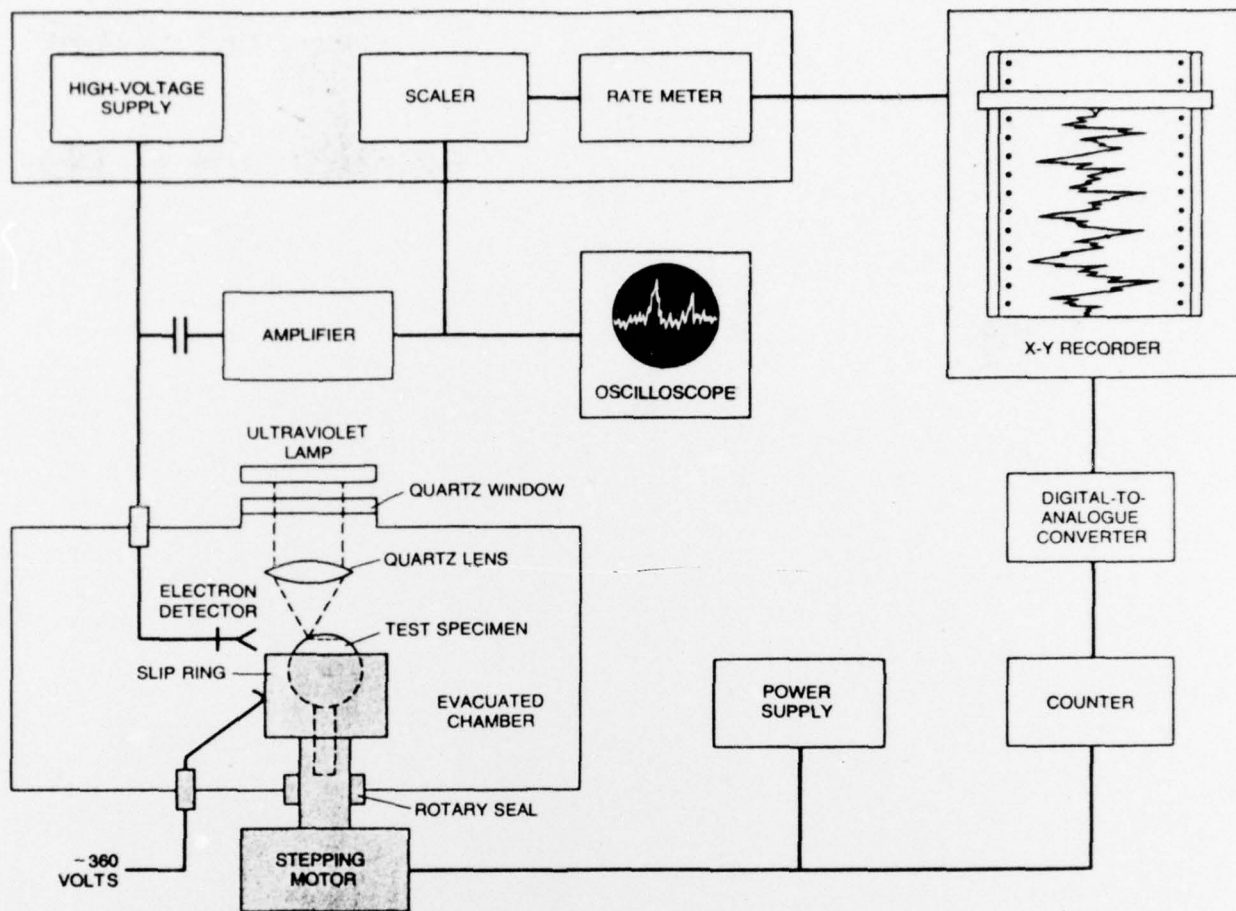
EXO-ELECTRON EMISSION from bearing balls was measured and recorded with this apparatus in the author's laboratory at the Massachusetts Institute of Technology. After being removed from the device shown on the opposite page balls are cleaned and mounted in a
