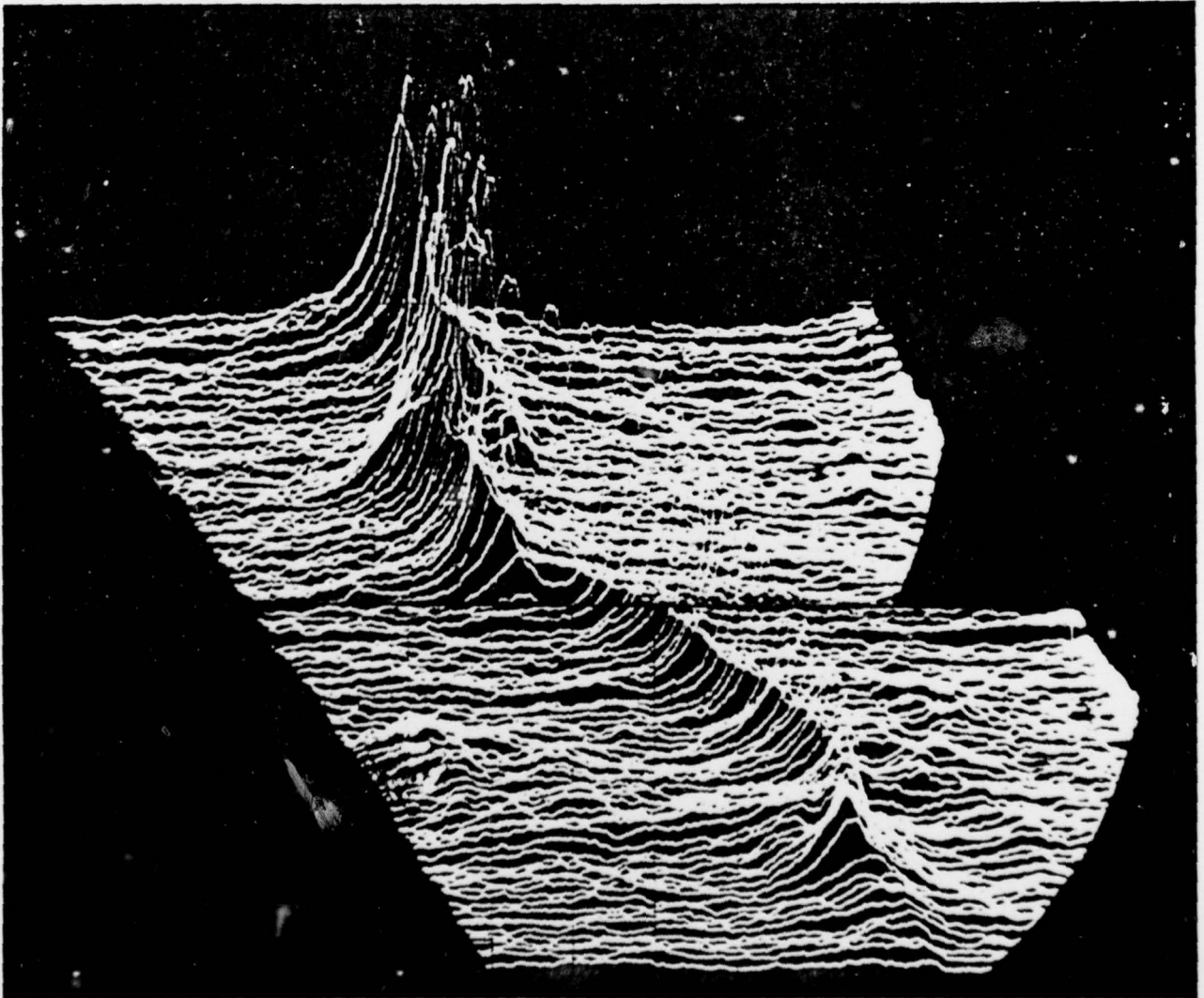
EXOELECTRON IMAGE of the fatigue crack shown optically on the opposite page provides information that is both more graphic and potentially more useful. In general the fresher the surface is, the more exoelectrons are emitted. The exoelectron image shown here was made by scanning the aluminum surface with a fine beam of ultraviolet radiation, which stimulates the emission of exoelectrons.
