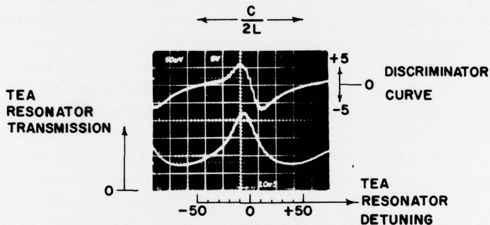
FIGURE 2 - TEA resonator spectral transmission and discriminator curve as obtained by scanning the cavity length.
