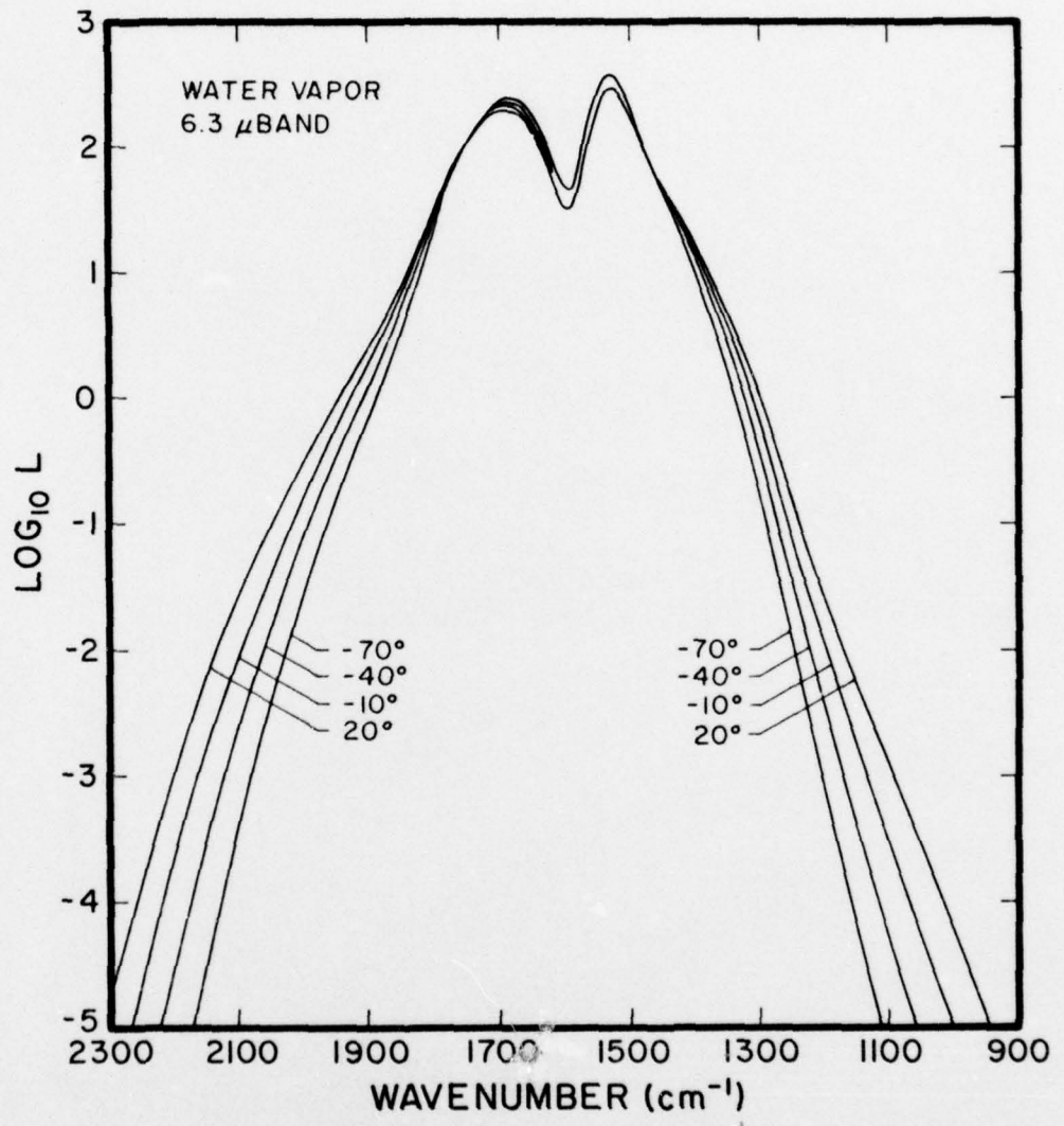
Figure 2. Generalized absorption coefficient for the 6.3 \mu\text{m} water vapor band for various temperatures ( ^{\circ}\text{C} ).
