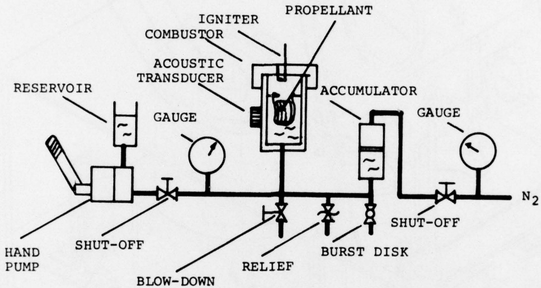
Fig. 2-1 The intermediate pressure combustor system The combustor cell is pressurized with water using a hand pump. The propellant grain is then ignited and its acoustic output in the UHFAE range is sensed by an acoustic emissions transducer. The pressure in the combustor is kept constant using the nitrogen accumulator system shown. After the burn, spent water is exhausted and pressure is relieved by opening the blow-down valve.
