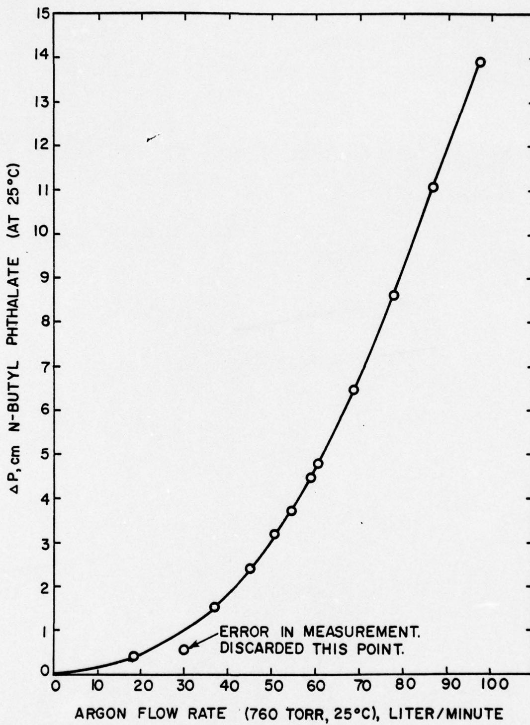
Figure 20. Nozzle calibration.
