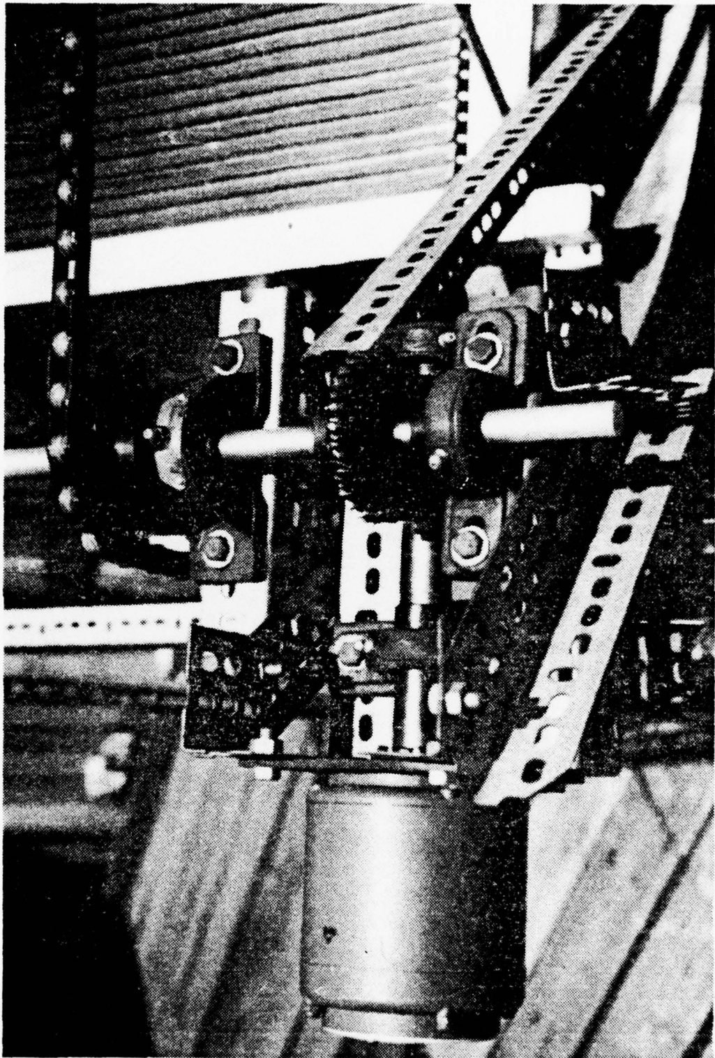
Figure 14. Drive detail.
