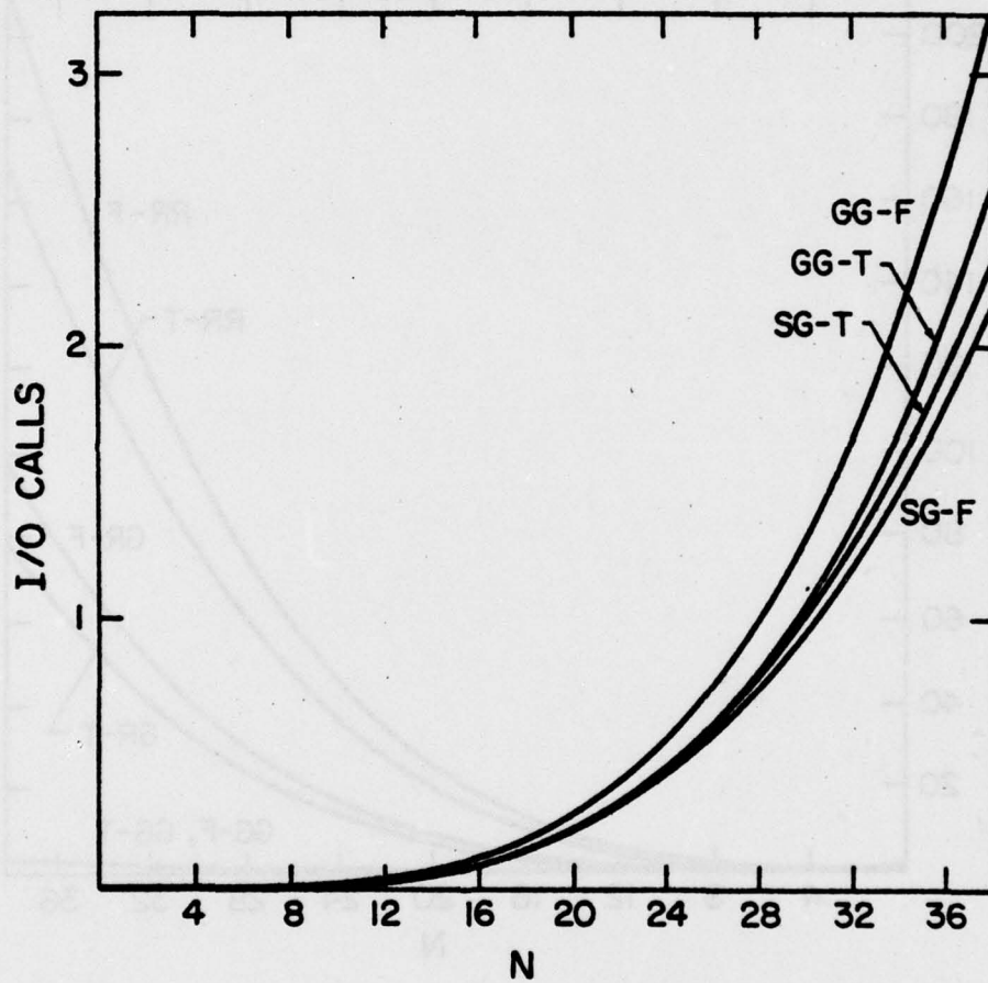
Figure 4. comparison of I/O Times (only GG, SG) for an E2S2 Problem
