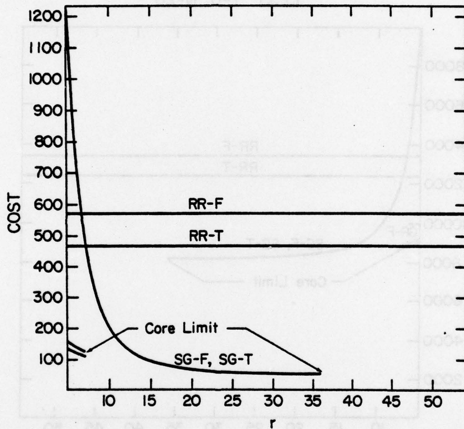
Figure 14. Cost of Run for a Complex Shell Problem (U=9120, b=912), For a Mini-Computer with a Floating Processor
