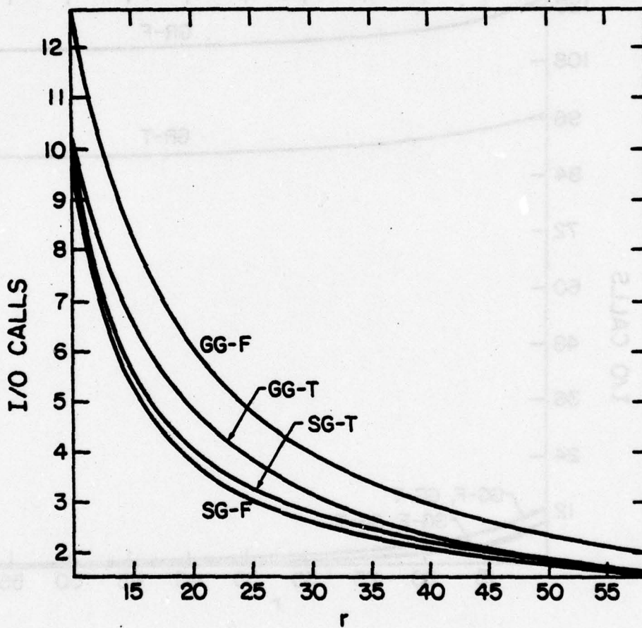
Figure 7. I/O Calls for Group Reduction Schemes (GG,SG) (U=3200, b=84)
