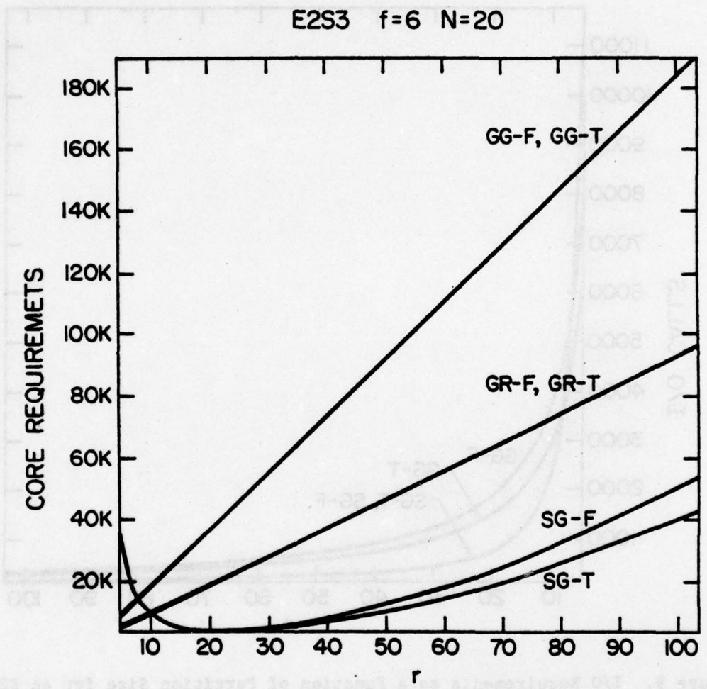
Figure 8. Core Requirements as a Function of Partition Size for an E2S3 Model (U=9120, b=912)
