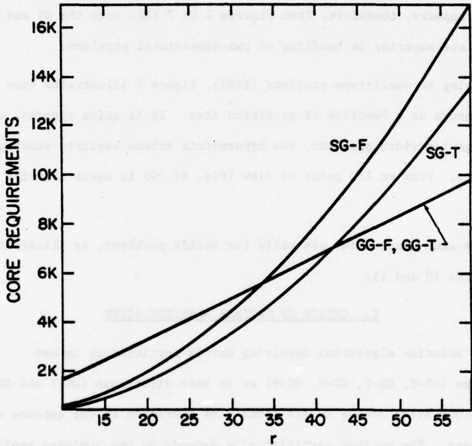
Figure 5. Core Requirement for an E2S2 Model as a Function of Partition Size (U=3200, b+84)
